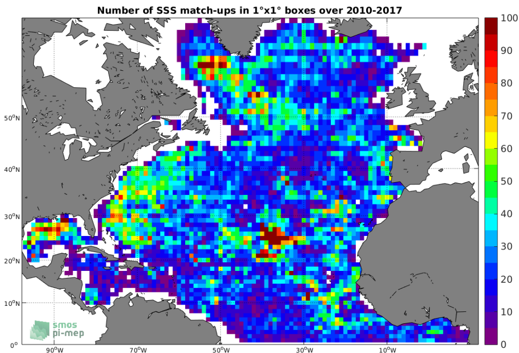
Figure 4: Number of SSS match-ups between Argo SSS and the SMOS-L3-CATDS-CECOS-LOCEAN-V3-18DAYS-25KM SSS product for the North Atlantic Ocean Pi-MEP region over 1^\circ \times 1^\circ boxes and for the full satellite product period.
