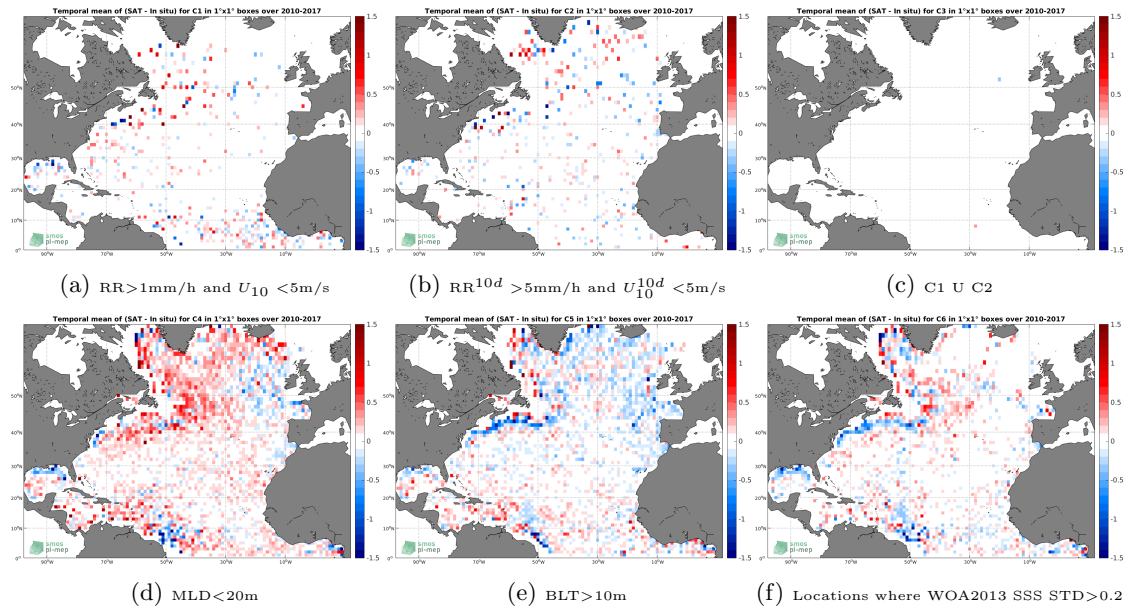
Figure 12: Temporal mean gridded over spatial boxes of size 1^\circ \times 1^\circ of \Delta SSS (SMOS-L3-CATDS-CECOS-LOCEAN-V3-18DAYS-25KM - Argo) for 6 different subdatasets corresponding to: RR > 1\text{mm/h} and U_{10} < 5\text{m/s} (a), RR^{10d} > 5\text{mm/h} and U_{10}^{10d} < 5\text{m/s} (b), C1 U C2 (c), MLD < 20\text{m} (d), BLT > 10\text{m} (e), Locations where WOA2013 SSS STD > 0.2 (f).
