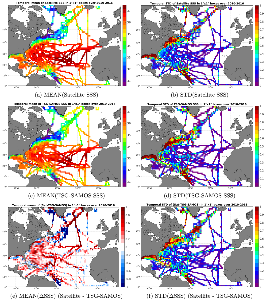
Figure 6: Temporal mean (left) and STD (right) of SSS from SMOS-L3-CATDS-CECOS-LOCEAN-V2.1-9DAYS-25KM (top), TSG-SAMOS (middle), and of \Delta SSS (Satellite - TSG-SAMOS). Only match-up pairs are used to generate these maps.
