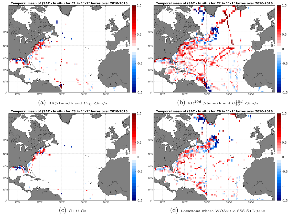
Figure 12: Temporal mean gridded over spatial boxes of size 1^\circ \times 1^\circ of \Delta SSS (SMOS-L3-CATDS-CECOS-LOCEAN-V2.1-9DAYS-25KM - TSG-SAMOS) for 4 different subdatasets corresponding to:RR > 1 mm/h and U_{10} < 5 m/s (a), RR 10d > 5 mm/h and U_{10}^{10d} < 5 m/s (b), C1 U C2 (c),Locations where WOA2013 SSS STD > 0.2 (d).
