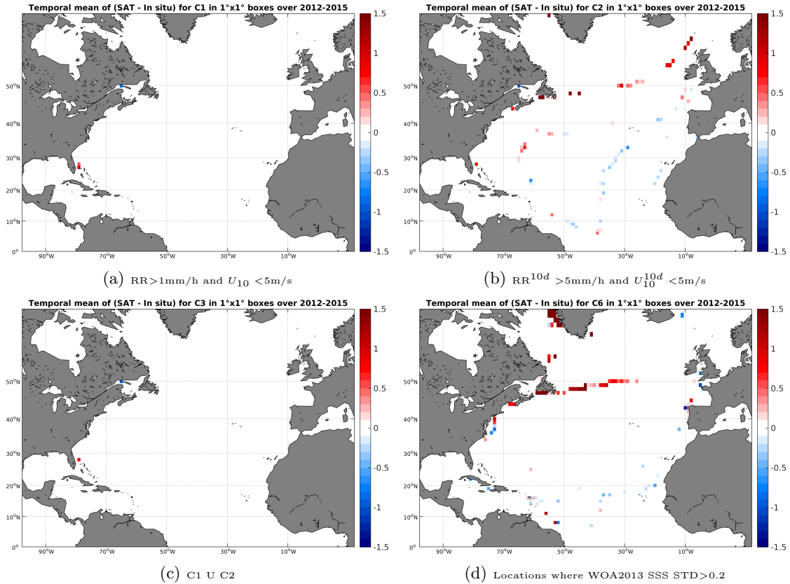
Figure 12: Temporal mean gridded over spatial boxes of size 1°x1° of \Delta SSS (SMOS-L3-CATDS-CECOS-LOCEAN-V2.1-9DAYS-25KM - TSG-GOSUD-Sailing-ship) for 4 different subdatasets corresponding to:RR>1mm/h and U_{10} < 5m/s (a), RR^{10d} > 5mm/h and U_{10}^{10d} < 5m/s (b), C1 U C2 (c),Locations where WOA2013 SSS STD>0.2 (d).
