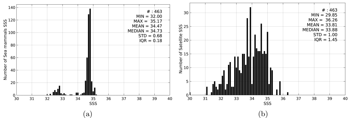
Figure 2: Histograms of SSS from Sea mammals (a) and SMOS-L3-CATDS-CECOS-LOCEAN-V2.1-9DAYS-25KM (b) considering all match-up pairs per bins of 0.1 over the North Atlantic Ocean Pi-MEP region and for the full satellite product period.
