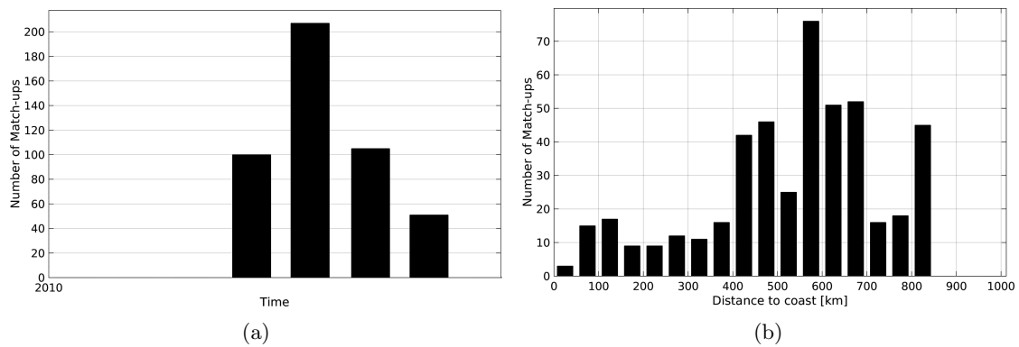
Figure 1: Number of match-ups between Sea mammals and SMOS-L3-CATDS-CECOS-LOCEAN-V2.1-9DAYS-25KM SSS as a function of time (a) and as function of the distance to coast (b) over the North Atlantic Ocean Pi-MEP region and for the full satellite product period.
