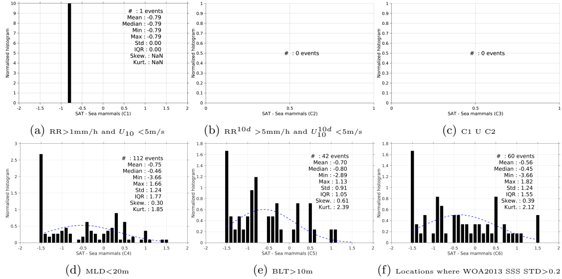
Figure 13: Normalized histogram of \Delta SSS (SMOS-L3-CATDS-CECOS-LOCEAN-V2.1-9DAYS-25KM - Sea mammals) for 6 different subdatasets corresponding to: RR > 1\text{mm/h} and U_{10} < 5\text{m/s} (a), RR^{10d} > 5\text{mm/h} and U_{10}^{10d} < 5\text{m/s} (b), C1 U C2 (c), MLD < 20\text{m} (d), BLT > 10\text{m} (e), Locations where WOA2013 SSS STD > 0.2 (f).
