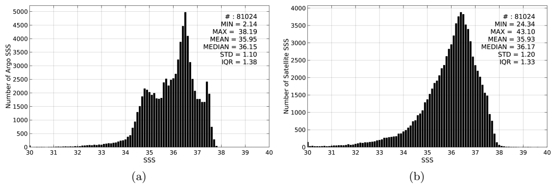
Figure 2: Histograms of SSS from Argo (a) and SMOS-L3-CATDS-CECOS-LOCEAN-V2.1-9DAYS-25KM (b) considering all match-up pairs per bins of 0.1 over the North Atlantic Ocean Pi-MEP region and for the full satellite product period.
