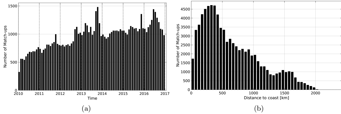
Figure 1: Number of match-ups between Argo and SMOS-L3-CATDS-CECOS-LOCEAN-V2.1-9DAYS-25KM SSS as a function of time (a) and as function of the distance to coast (b) over the North Atlantic Ocean Pi-MEP region and for the full satellite product period.
