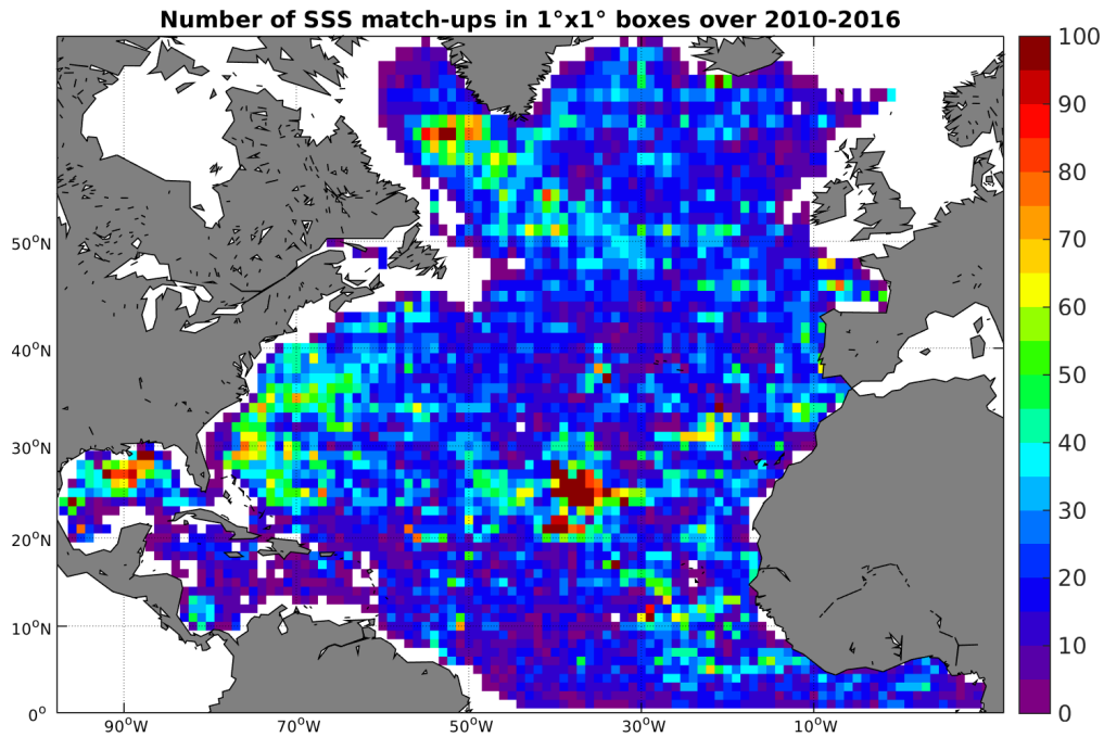
Figure 4: Number of SSS match-ups between Argo SSS and the SMOS-L3-CATDS-CECOS-LOCEAN-V2.1-9DAYS-25KM SSS product for the North Atlantic Ocean Pi-MEP region over 1^\circ \times 1^\circ boxes and for the full satellite product period.
