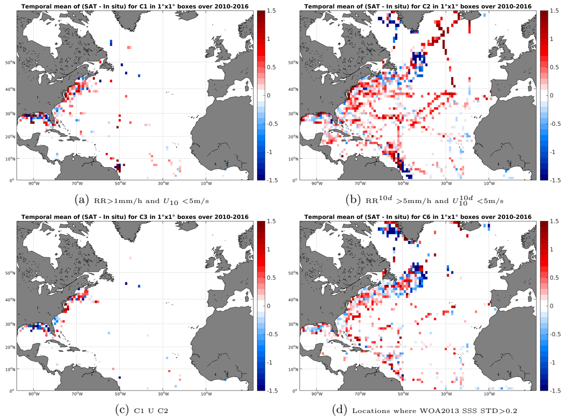
Figure 12: Temporal mean gridded over spatial boxes of size 1^\circ \times 1^\circ of \Delta SSS (SMOS-L3-CATDS-CECOS-LOCEAN-V2-9DAYS-25KM - TSG-SAMOS) for 4 different subdatasets corresponding to:RR > 1 mm/h and U_{10} < 5 m/s (a), RR 10d > 5 mm/h and U_{10}^{10d} < 5 m/s (b), C1 U C2 (c),Locations where WOA2013 SSS STD > 0.2 (d).
