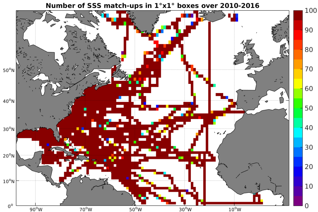
Figure 4: Number of SSS match-ups between TSG-SAMOS SSS and the SMOS-L3-CATDS-CECOS-LOCEAN-V2-9DAYS-25KM SSS product for the North Atlantic Ocean Pi-MEP region over 1^\circ \times 1^\circ boxes and for the full satellite product period.
