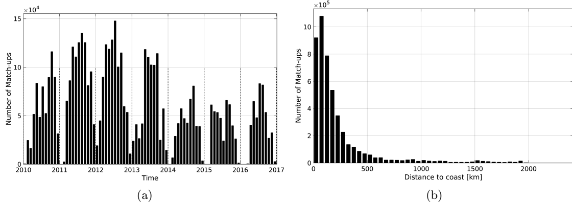
Figure 1: Number of match-ups between TSG-SAMOS and SMOS-L3-CATDS-CECOS-LOCEAN-V2-9DAYS-25KM SSS as a function of time (a) and as function of the distance to coast (b) over the North Atlantic Ocean Pi-MEP region and for the full satellite product period.
