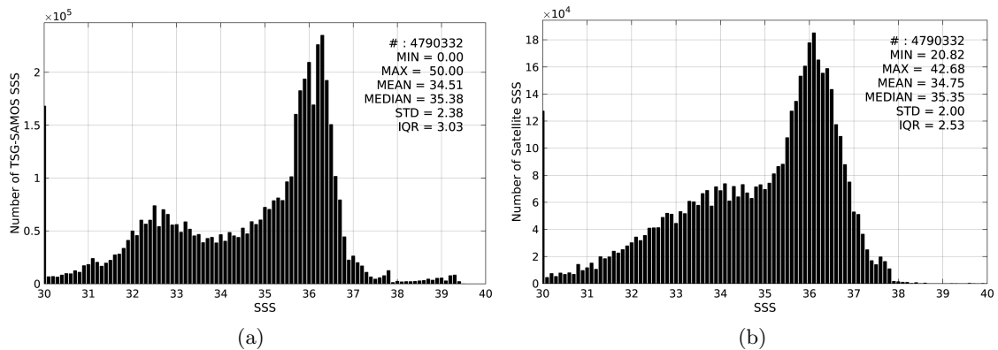
Figure 2: Histograms of SSS from TSG-SAMOS (a) and SMOS-L3-CATDS-CECOS-LOCEAN-V2-9DAYS-25KM (b) considering all match-up pairs per bins of 0.1 over the North Atlantic Ocean Pi-MEP region and for the full satellite product period.
