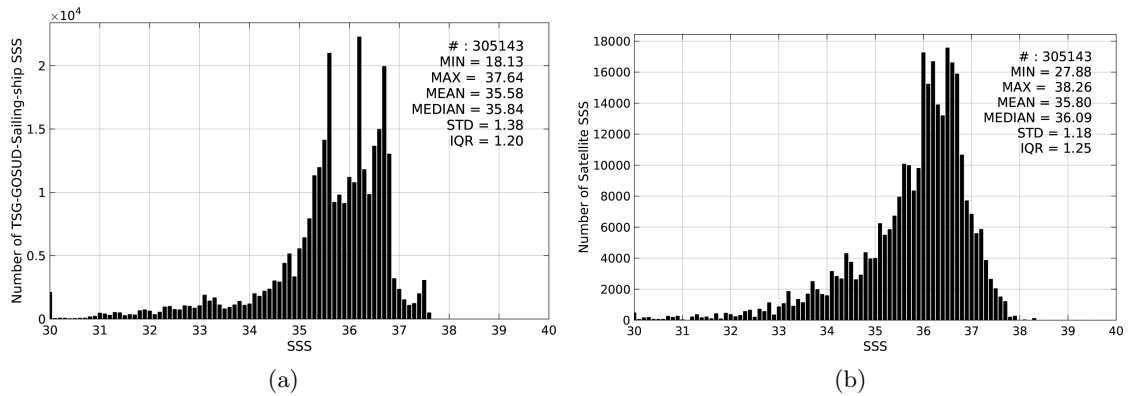
Figure 2: Histograms of SSS from TSG-GOSUD-Sailing-ship (a) and SMOS-L3-CATDS-CECOS-LOCEAN-V2-9DAYS-25KM (b) considering all match-up pairs per bins of 0.1 over the North Atlantic Ocean Pi-MEP region and for the full satellite product period.
