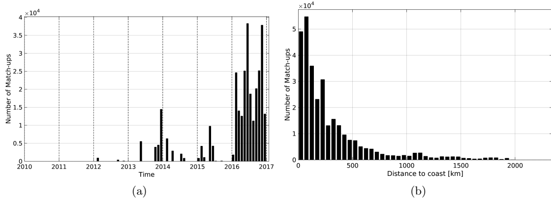
Figure 1: Number of match-ups between TSG-GOSUD-Sailing-ship and SMOS-L3-CATDS-CECOS-LOCEAN-V2-9DAYS-25KM SSS as a function of time (a) and as function of the distance to coast (b) over the North Atlantic Ocean Pi-MEP region and for the full satellite product period.
