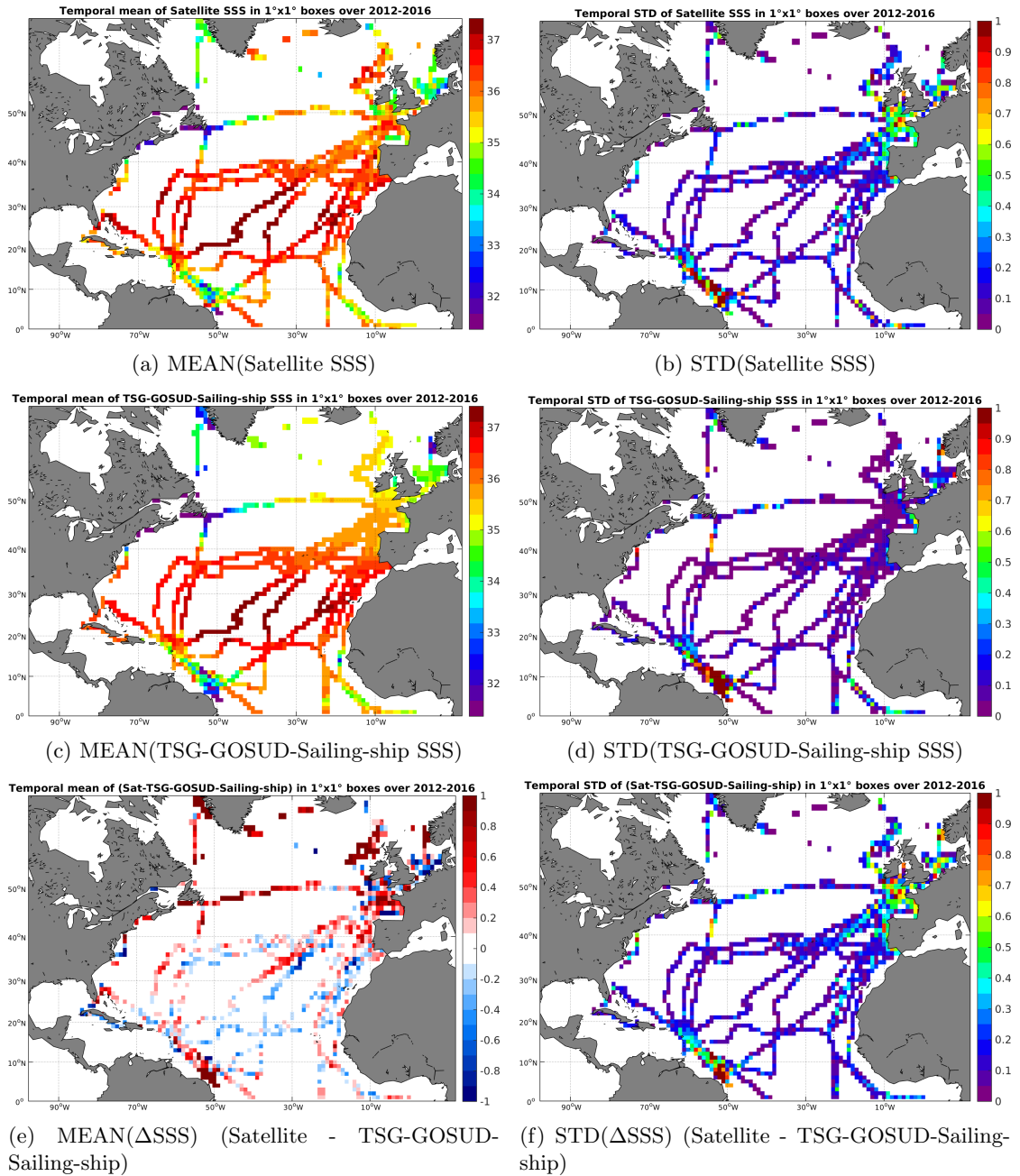
Figure 6: Temporal mean (left) and STD (right) of SSS from SMOS-L3-CATDS-CECOS-LOCEAN-V2-9DAYS-25KM (top), TSG-GOSUD-Sailing-ship (middle), and of \Delta SSS (Satellite - TSG-GOSUD-Sailing-ship). Only match-up pairs are used to generate these maps.
