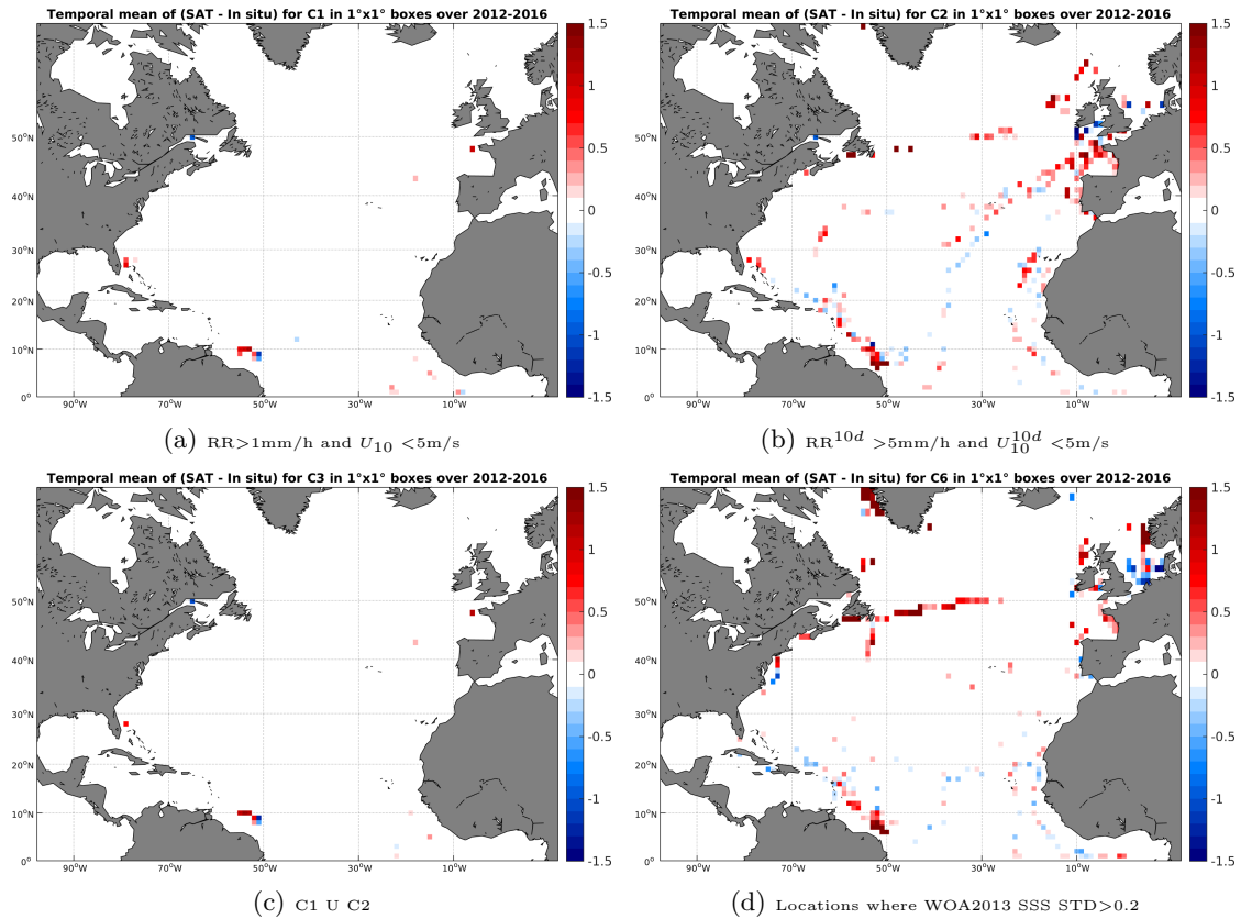
Figure 12: Temporal mean gridded over spatial boxes of size 1^\circ \times 1^\circ of \Delta SSS (SMOS-L3-CATDS-CECOS-LOCEAN-V2-9DAYS-25KM - TSG-GOSUD-Sailing-ship) for 4 different subdatasets corresponding to:RR>1mm/h and U_{10} < 5\text{m/s} (a), RR^{10d} > 5\text{mm/h} and U_{10}^{10d} < 5\text{m/s} (b), C1 U C2 (c),Locations where WOA2013 SSS STD>0.2 (d).
