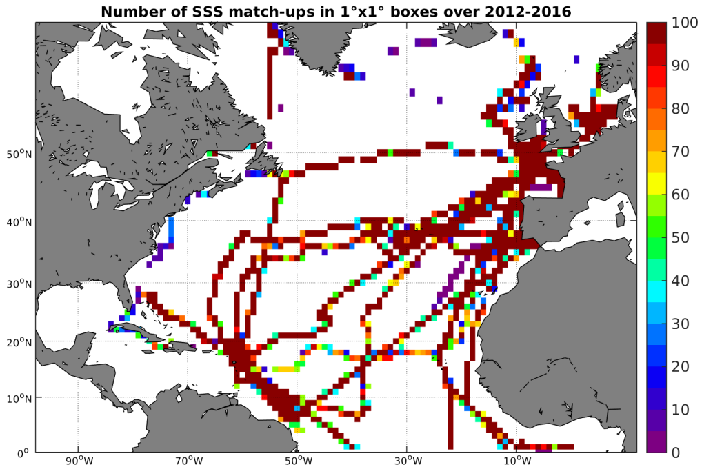
Figure 4: Number of SSS match-ups between TSG-GOSUD-Sailing-ship SSS and the SMOS-L3-CATDS-CECOS-LOCEAN-V2-9DAYS-25KM SSS product for the North Atlantic Ocean Pi-MEP region over 1^\circ \times 1^\circ boxes and for the full satellite product period.
