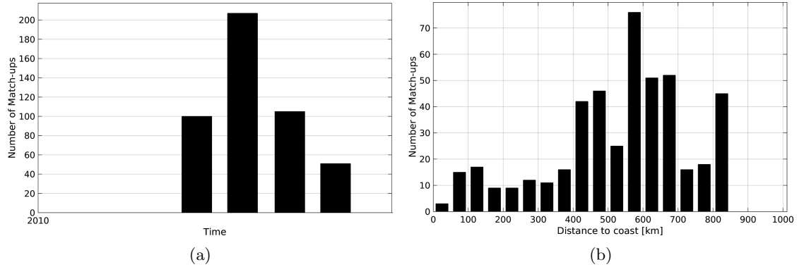
Figure 1: Number of match-ups between Sea mammals and SMOS-L3-CATDS-CECOS-LOCEAN-V2-9DAYS-25KM SSS as a function of time (a) and as function of the distance to coast (b) over the North Atlantic Ocean Pi-MEP region and for the full satellite product period.
