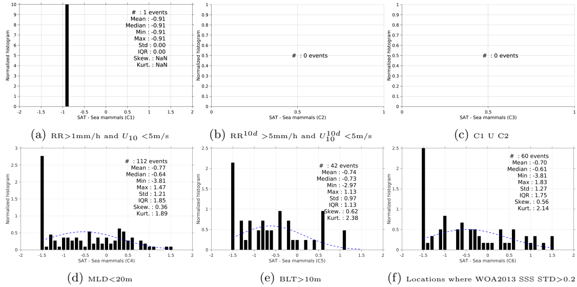
Figure 13: Normalized histogram of \Delta SSS (SMOS-L3-CATDS-CECOS-LOCEAN-V2-9DAYS-25KM - Sea mammals) for 6 different subdatasets corresponding to: RR>1mm/h and U_{10} < 5\text{m/s} (a), RR^{10d} > 5\text{mm/h} and U_{10}^{10d} < 5\text{m/s} (b), C1 U C2 (c),MLD<20m (d),BLT>10m (e),Locations where WOA2013 SSS STD>0.2 (f).
