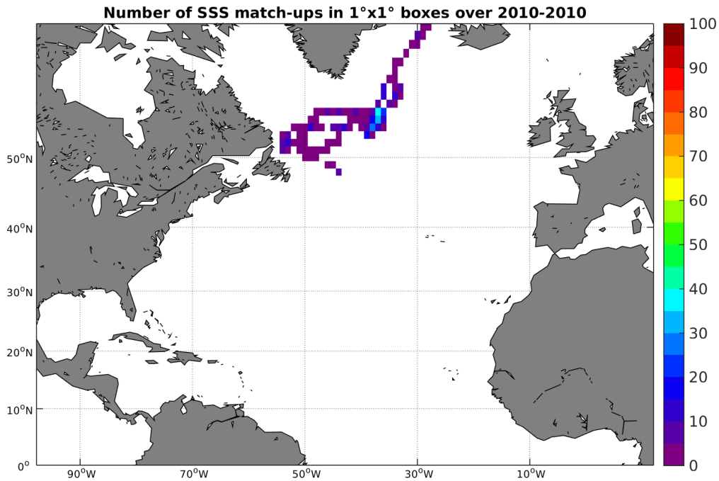
Figure 4: Number of SSS match-ups between Sea mammals SSS and the SMOS-L3-CATDS-CECOS-LOCEAN-V2-9DAYS-25KM SSS product for the North Atlantic Ocean Pi-MEP region over 1^\circ \times 1^\circ boxes and for the full satellite product period.
