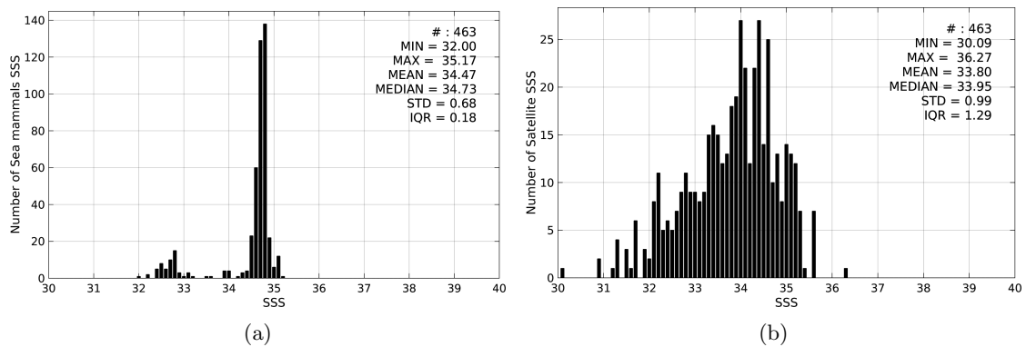
Figure 2: Histograms of SSS from Sea mammals (a) and SMOS-L3-CATDS-CECOS-LOCEAN-V2-9DAYS-25KM (b) considering all match-up pairs per bins of 0.1 over the North Atlantic Ocean Pi-MEP region and for the full satellite product period.
