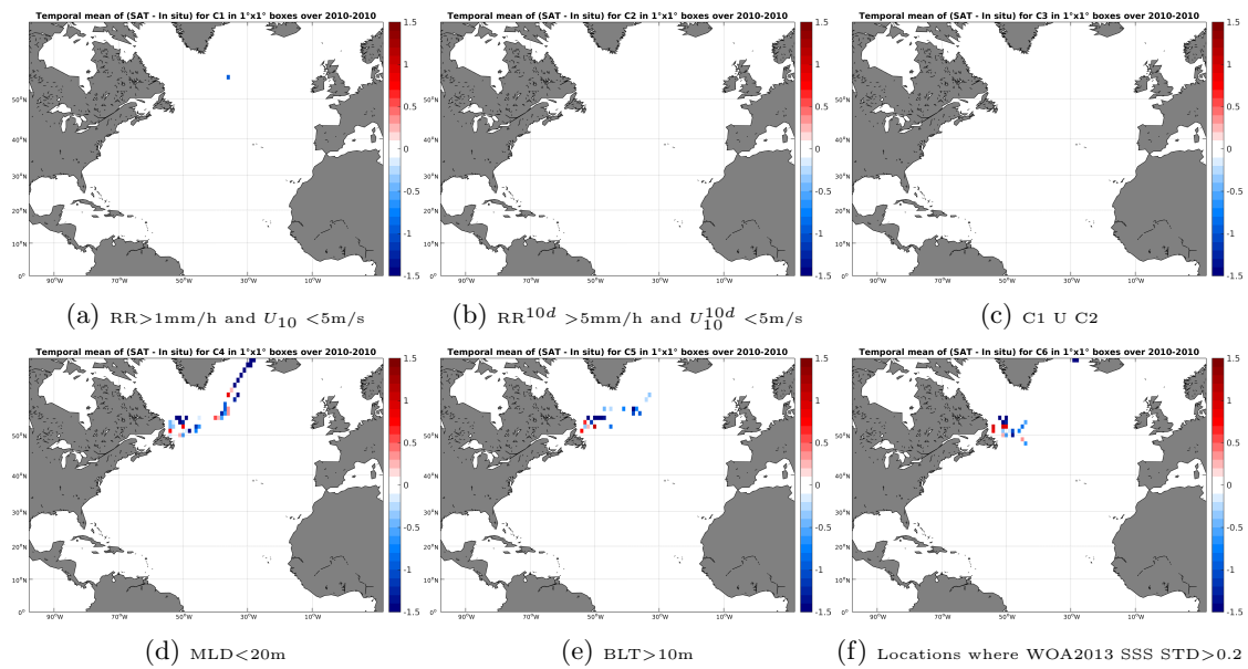
Figure 12: Temporal mean gridded over spatial boxes of size 1^\circ \times 1^\circ of \Delta SSS (SMOS-L3-CATDS-CECOS-LOCEAN-V2-9DAYS-25KM - Sea mammals) for 6 different subdatasets corresponding to: RR > 1\text{mm/h} and U_{10} < 5\text{m/s} (a), RR^{10d} > 5\text{mm/h} and U_{10}^{10d} < 5\text{m/s} (b), C1 U C2 (c), MLD < 20\text{m} (d), BLT > 10\text{m} (e), Locations where WOA2013 SSS STD > 0.2 (f).
