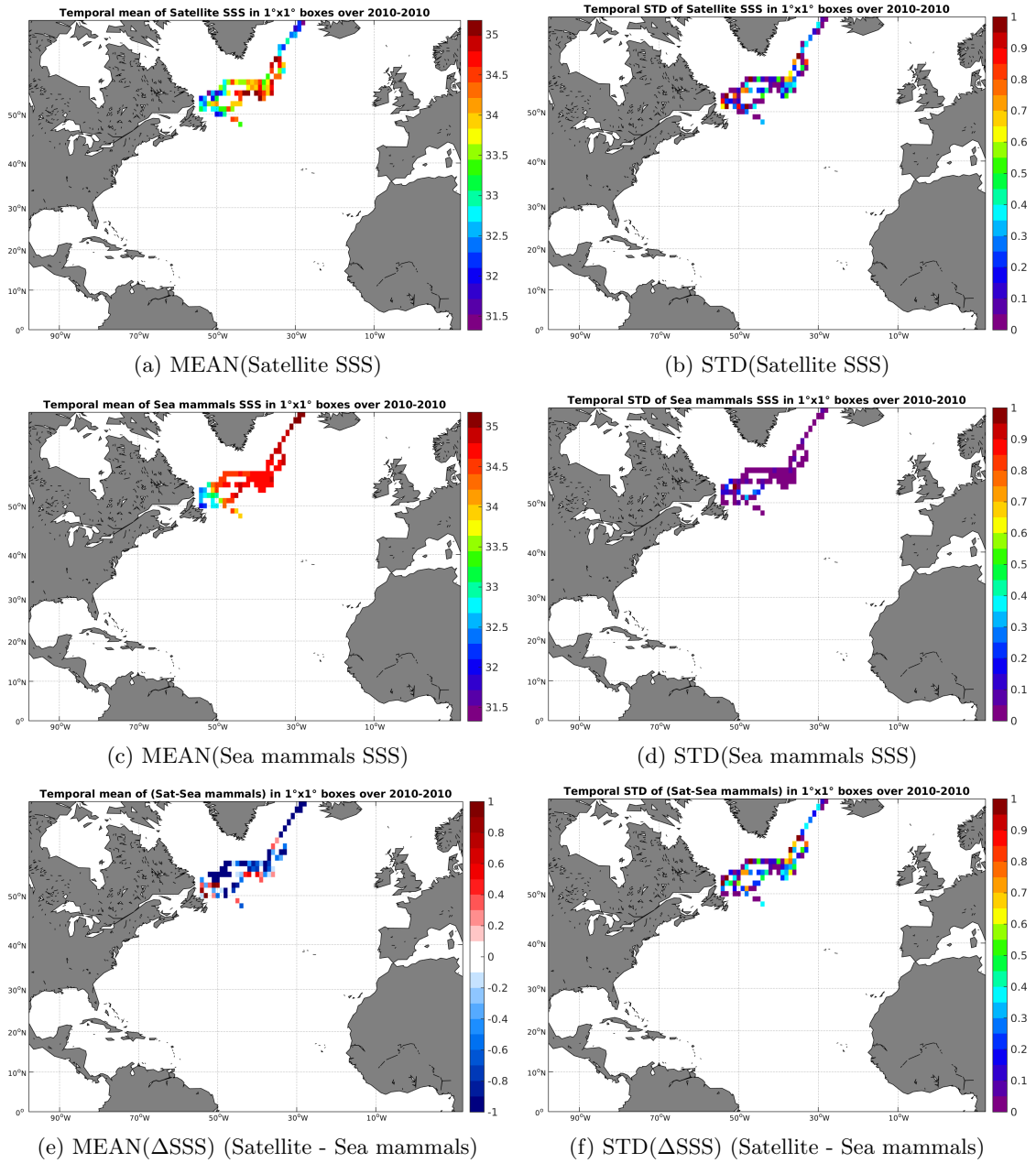
Figure 6: Temporal mean (left) and STD (right) of SSS from SMOS-L3-CATDS-CECOS-LOCEAN-V2-9DAYS-25KM (top), Sea mammals (middle), and of \Delta SSS (Satellite - Sea mammals). Only match-up pairs are used to generate these maps.
