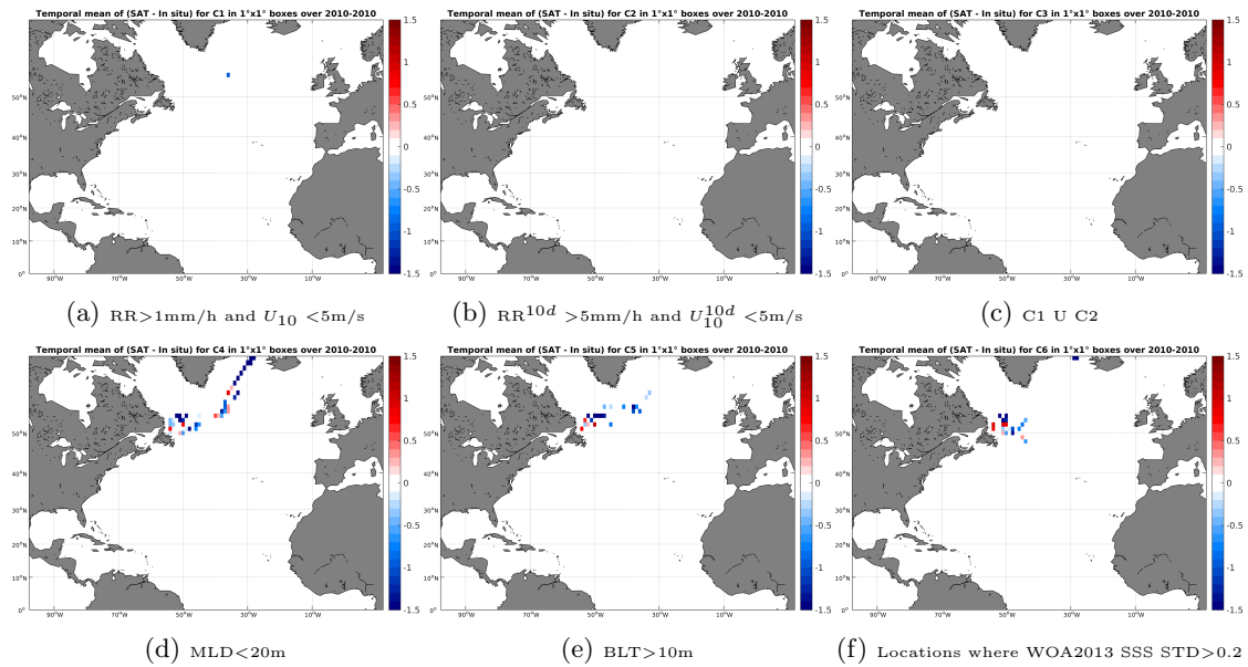
Figure 12: Temporal mean gridded over spatial boxes of size 1^\circ \times 1^\circ of \Delta SSS (SMOS-L3-CATDS-CECOS-LOCEAN-V2-9DAYS-25KM - Sea mammals) for 6 different subdatasets corresponding to:RR >1 mm/h and U_{10} < 5 m/s (a), RR^{10d} > 5 mm/h and U_{10}^{10d} < 5 m/s (b), C1 U C2 (c),MLD <20 m (d),BLT >10 m (e),Locations where WOA2013 SSS STD >0.2 (f).
