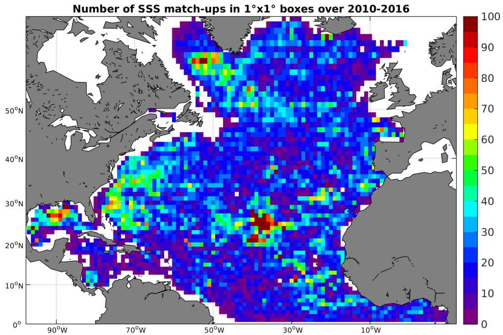
Figure 4: Number of SSS match-ups between Argo SSS and the SMOS-L3-CATDS-CECOS-LOCEAN-V2-9DAYS-25KM SSS product for the North Atlantic Ocean Pi-MEP region over 1^\circ \times 1^\circ boxes and for the full satellite product period.
