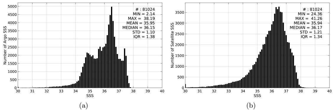
Figure 2: Histograms of SSS from Argo (a) and SMOS-L3-CATDS-CECOS-LOCEAN-V2-9DAYS-25KM (b) considering all match-up pairs per bins of 0.1 over the North Atlantic Ocean Pi-MEP region and for the full satellite product period.
