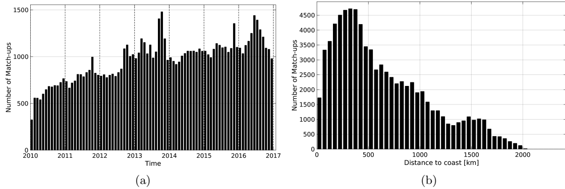
Figure 1: Number of match-ups between Argo and SMOS-L3-CATDS-CECOS-LOCEAN-V2-9DAYS-25KM SSS as a function of time (a) and as function of the distance to coast (b) over the North Atlantic Ocean Pi-MEP region and for the full satellite product period.
