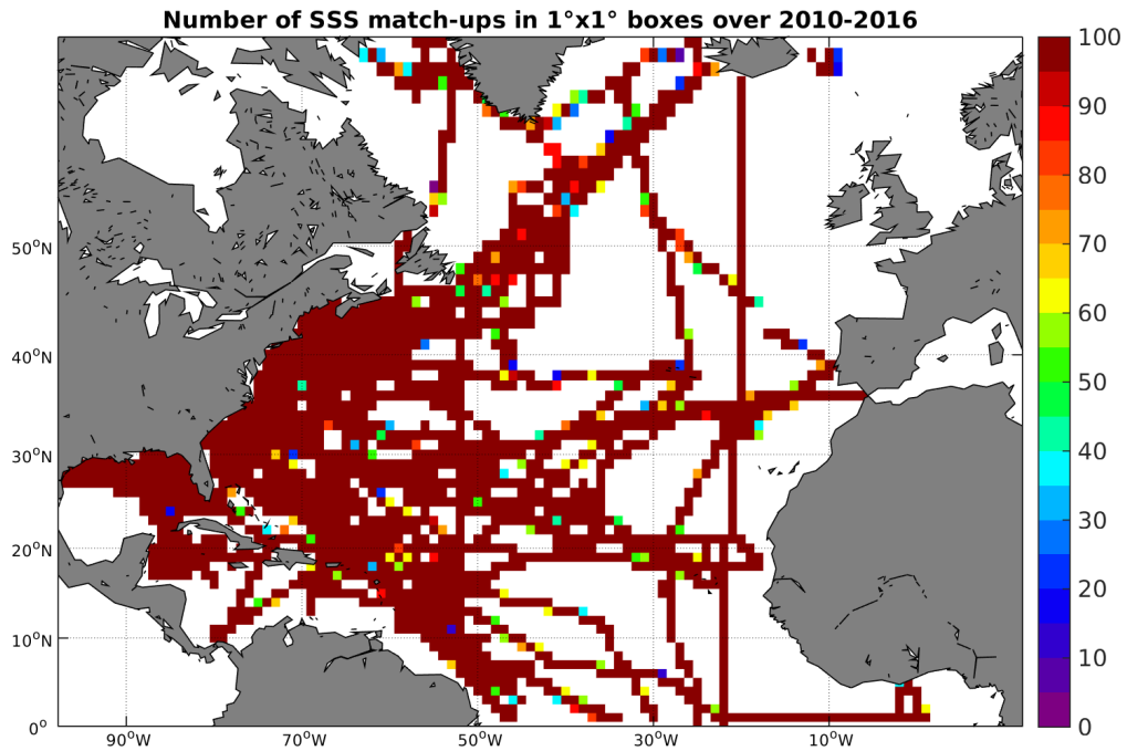
Figure 4: Number of SSS match-ups between TSG-SAMOS SSS and the SMOS-L3-CATDS-CECOS-LOCEAN-V2-18DAYS-25KM SSS product for the North Atlantic Ocean Pi-MEP region over 1^\circ \times 1^\circ boxes and for the full satellite product period.
