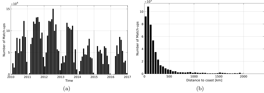
Figure 1: Number of match-ups between TSG-SAMOS and SMOS-L3-CATDS-CECOS-LOCEAN-V2-18DAYS-25KM SSS as a function of time (a) and as function of the distance to coast (b) over the North Atlantic Ocean Pi-MEP region and for the full satellite product period.
