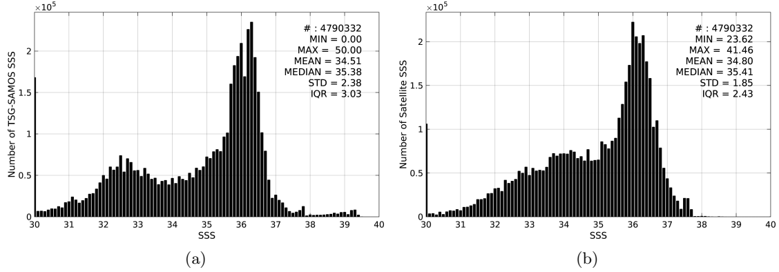
Figure 2: Histograms of SSS from TSG-SAMOS (a) and SMOS-L3-CATDS-CECOS-LOCEAN-V2-18DAYS-25KM (b) considering all match-up pairs per bins of 0.1 over the North Atlantic Ocean Pi-MEP region and for the full satellite product period.
