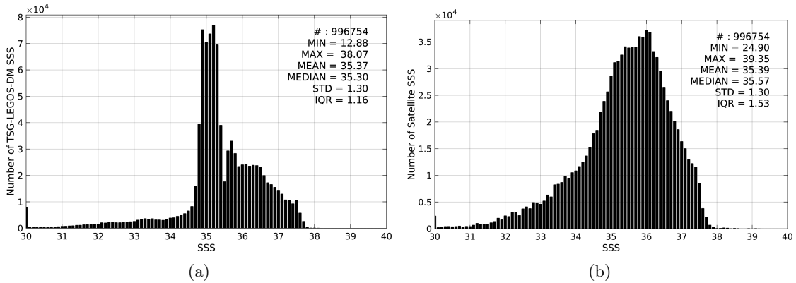
Figure 2: Histograms of SSS from TSG-LEGOS-DM (a) and SMOS-L3-CATDS-CECOS-LOCEAN-V2-18DAYS-25KM (b) considering all match-up pairs per bins of 0.1 over the North Atlantic Ocean Pi-MEP region and for the full satellite product period.
