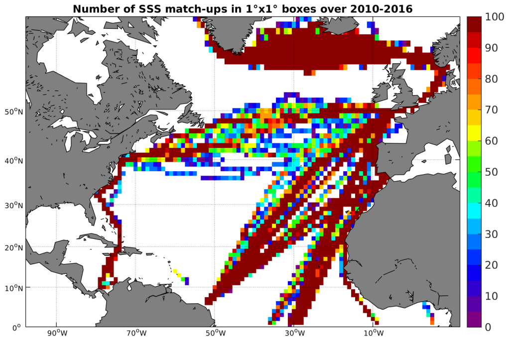
Figure 4: Number of SSS match-ups between TSG-LEGOS-DM SSS and the SMOS-L3-CATDS-CECOS-LOCEAN-V2-18DAYS-25KM SSS product for the North Atlantic Ocean Pi-MEP region over 1^\circ \times 1^\circ boxes and for the full satellite product period.
