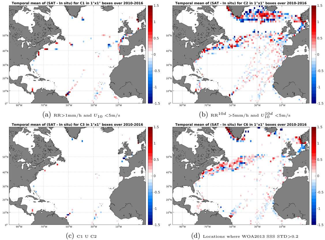
Figure 12: Temporal mean gridded over spatial boxes of size 1^\circ \times 1^\circ of \Delta SSS (SMOS-L3-CATDS-CECOS-LOCEAN-V2-18DAYS-25KM - TSG-LEGOS-DM) for 4 different subdatasets corresponding to:RR>1mm/h and U_{10} < 5 m/s (a), RR^{10d} > 5 mm/h and U_{10}^{10d} < 5 m/s (b), C1 U C2 (c),Locations where WOA2013 SSS STD>0.2 (d).
