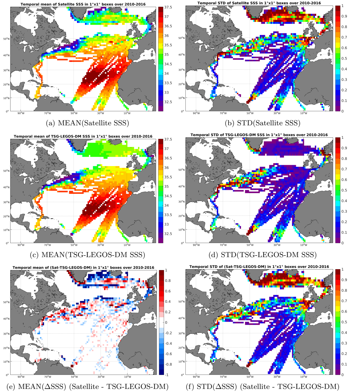
Figure 6: Temporal mean (left) and STD (right) of SSS from SMOS-L3-CATDS-CECOS-LOCEAN-V2-18DAYS-25KM (top), TSG-LEGOS-DM (middle), and of \Delta SSS (Satellite - TSG-LEGOS-DM). Only match-up pairs are used to generate these maps.
