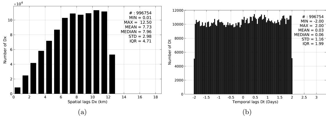
Figure 5: Histograms of the spatial (a) and temporal (b) lags between the time of the TSG-LEGOS-DM measurements and the date of the corresponding SMOS-L3-CATDS-CECOS-LOCEAN-V2-18DAYS-25KM SSS product.
