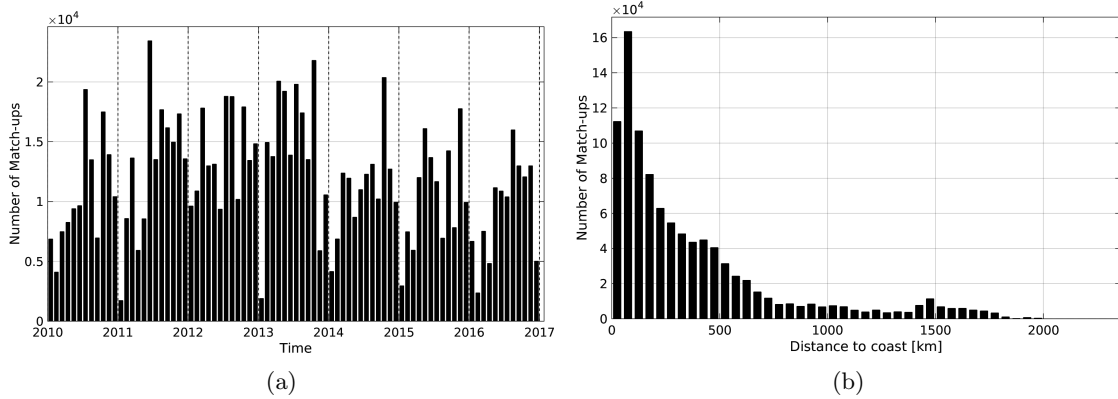
Figure 1: Number of match-ups between TSG-LEGOS-DM and SMOS-L3-CATDS-CECOS-LOCEAN-V2-18DAYS-25KM SSS as a function of time (a) and as function of the distance to coast (b) over the North Atlantic Ocean Pi-MEP region and for the full satellite product period.
