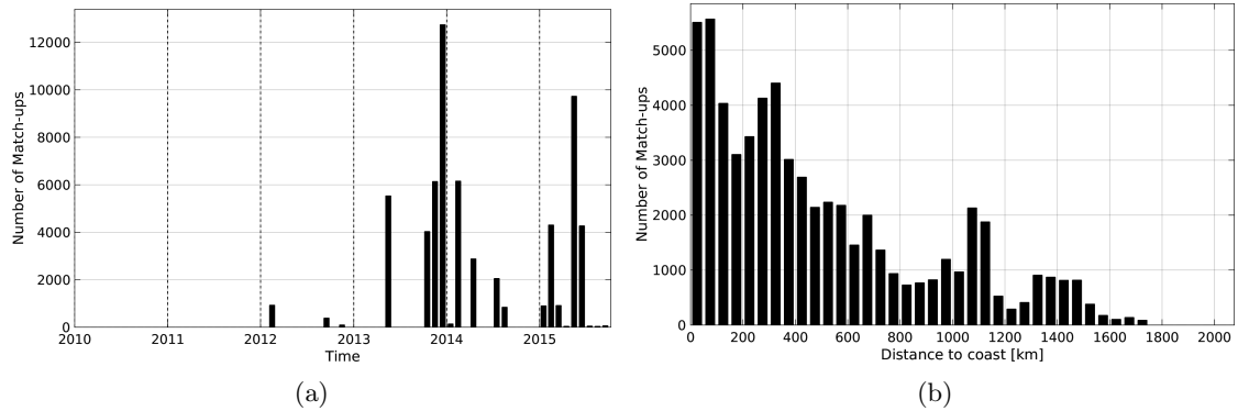
Figure 1: Number of match-ups between TSG-GOSUD-Sailing-ship and SMOS-L3-CATDS-CECOS-LOCEAN-V2-18DAYS-25KM SSS as a function of time (a) and as function of the distance to coast (b) over the North Atlantic Ocean Pi-MEP region and for the full satellite product period.
