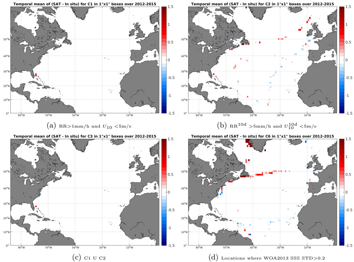
Figure 12: Temporal mean gridded over spatial boxes of size 1°x1° of \Delta SSS (SMOS-L3-CATDS-CECOS-LOCEAN-V2-18DAYS-25KM - TSG-GOSUD-Sailing-ship) for 4 different subdatasets corresponding to: RR > 1mm/h and U_{10} < 5\text{m/s} (a), RR^{10d} > 5\text{mm/h} and U_{10}^{10d} < 5\text{m/s} (b), C1 U C2 (c), Locations where WOA2013 SSS STD > 0.2 (d).
