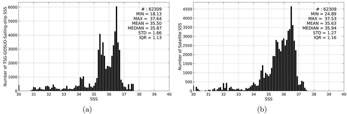
Figure 2: Histograms of SSS from TSG-GOSUD-Sailing-ship (a) and SMOS-L3-CATDS-CECOS-LOCEAN-V2-18DAYS-25KM (b) considering all match-up pairs per bins of 0.1 over the North Atlantic Ocean Pi-MEP region and for the full satellite product period.
