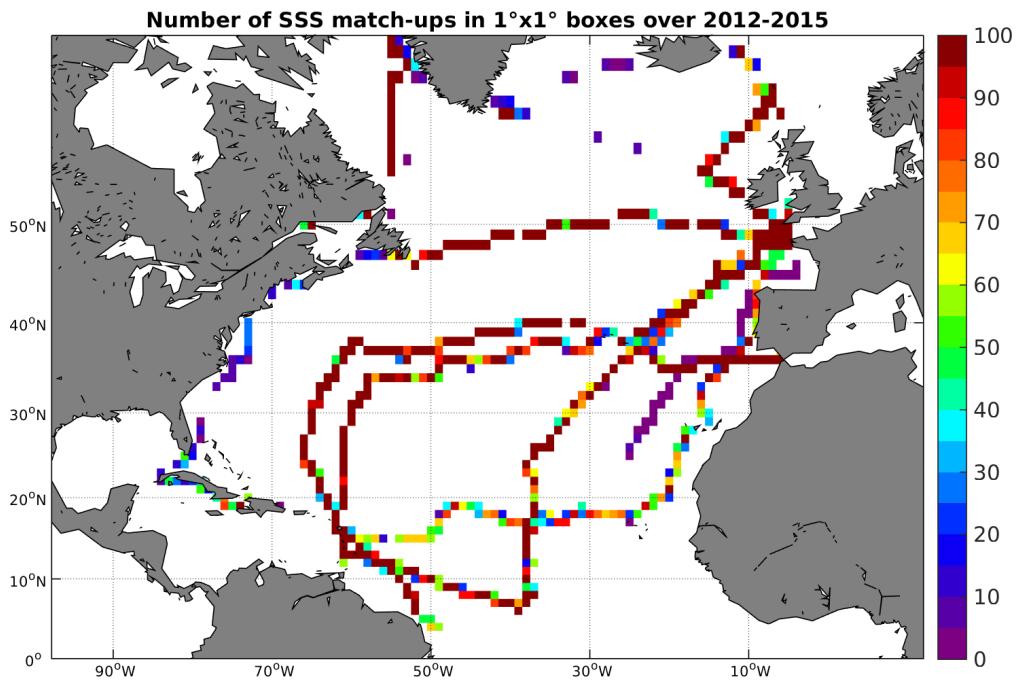
Figure 4: Number of SSS match-ups between TSG-GOSUD-Sailing-ship SSS and the SMOS-L3-CATDS-CECOS-LOCEAN-V2-18DAYS-25KM SSS product for the North Atlantic Ocean Pi-MEP region over 1^\circ \times 1^\circ boxes and for the full satellite product period.
