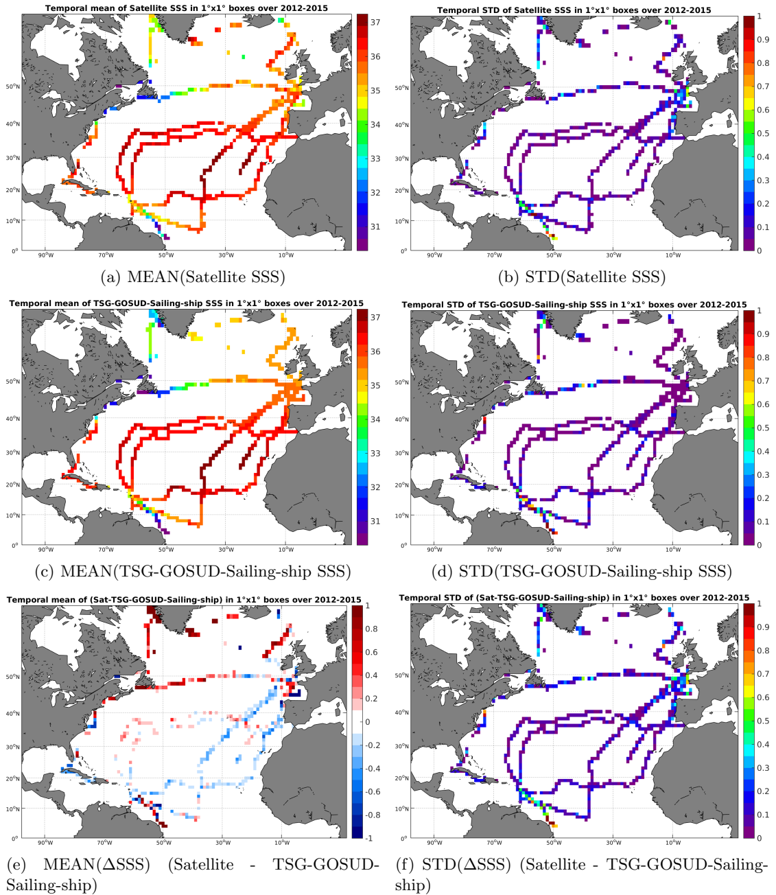
Figure 6: Temporal mean (left) and STD (right) of SSS from SMOS-L3-CATDS-CECOS-LOCEAN-V2-18DAYS-25KM (top), TSG-GOSUD-Sailing-ship (middle), and of \Delta SSS (Satellite - TSG-GOSUD-Sailing-ship). Only match-up pairs are used to generate these maps.
