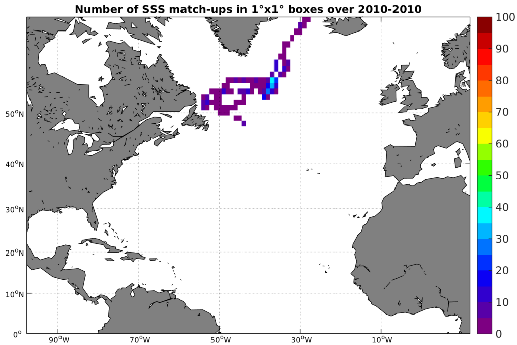
Figure 4: Number of SSS match-ups between Sea mammals SSS and the SMOS-L3-CATDS-CECOS-LOCEAN-V2-18DAYS-25KM SSS product for the North Atlantic Ocean Pi-MEP region over 1^\circ \times 1^\circ boxes and for the full satellite product period.
