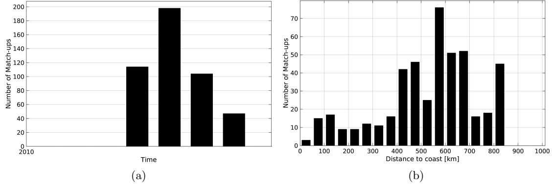
Figure 1: Number of match-ups between Sea mammals and SMOS-L3-CATDS-CECOS-LOCEAN-V2-18DAYS-25KM SSS as a function of time (a) and as function of the distance to coast (b) over the North Atlantic Ocean Pi-MEP region and for the full satellite product period.
