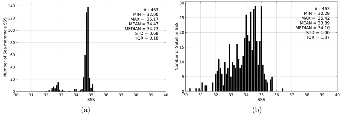
Figure 2: Histograms of SSS from Sea mammals (a) and SMOS-L3-CATDS-CECOS-LOCEAN-V2-18DAYS-25KM (b) considering all match-up pairs per bins of 0.1 over the North Atlantic Ocean Pi-MEP region and for the full satellite product period.
