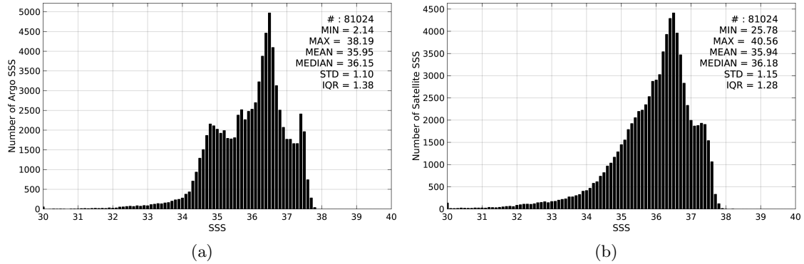
Figure 2: Histograms of SSS from Argo (a) and SMOS-L3-CATDS-CECOS-LOCEAN-V2-18DAYS-25KM (b) considering all match-up pairs per bins of 0.1 over the North Atlantic Ocean Pi-MEP region and for the full satellite product period.
