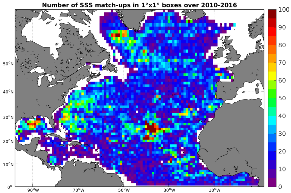
Figure 4: Number of SSS match-ups between Argo SSS and the SMOS-L3-CATDS-CECOS-LOCEAN-V2-18DAYS-25KM SSS product for the North Atlantic Ocean Pi-MEP region over 1^\circ \times 1^\circ boxes and for the full satellite product period.
