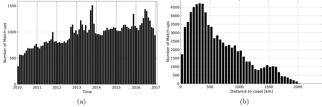
Figure 1: Number of match-ups between Argo and SMOS-L3-CATDS-CECOS-LOCEAN-V2-18DAYS-25KM SSS as a function of time (a) and as function of the distance to coast (b) over the North Atlantic Ocean Pi-MEP region and for the full satellite product period.
