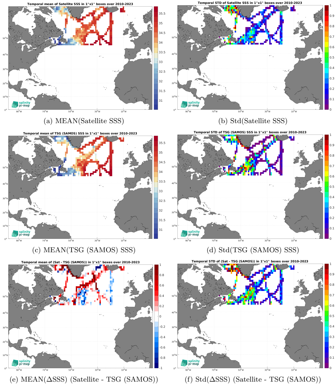
Figure 7: Temporal mean (left) and Std (right) of SSS from SMOS SSS L3 Arctic v2 - 9 Days (CATDS-CEC-LOCEAN) (top), TSG (SAMOS) (middle), and of \Delta SSS (Satellite - TSG (SAMOS)). Only match-up pairs are used to generate these maps.
