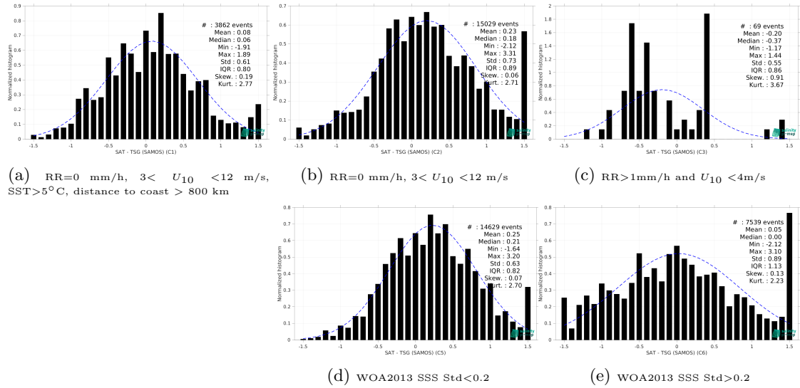
Figure 15: Normalized histogram of \Delta SSS (SMOS SSS L3 Arctic v2 - 9 Days (CATDS-CEC-LOCEAN) - TSG (SAMOS)) for 5 different subdatasets corresponding to: RR=0 mm/h, 3 < U_{10} < 12 m/s, SST>5°C, distance to coast > 800 km (a), RR=0 mm/h, 3 < U_{10} < 12 m/s (b), RR>1mm/h and U_{10} < 4 m/s (c), WOA2013 SSS Std<0.2 (d), WOA2013 SSS Std>0.2 (e).
