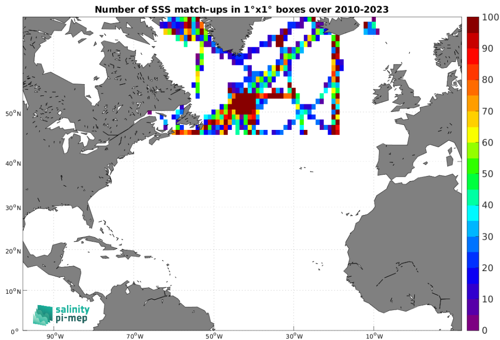
Figure 5: Number of SSS match-ups between TSG (SAMOS) SSS and the SMOS SSS L3 Arctic v2 - 9 Days (CATDS-CEC-LOCEAN) SSS product for the North Atlantic Ocean Pi-MEP region over 1^\circ \times 1^\circ boxes and for the full satellite product period.
