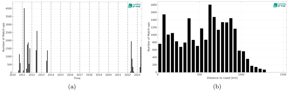
Figure 2: Number of match-ups between TSG (SAMOS) and SMOS SSS L3 Arctic v2 - 9 Days (CATDS-CEC-LOCEAN) SSS as a function of time (a) and as function of the distance to coast (b) over the North Atlantic Ocean Pi-MEP region and for the full satellite product period.
