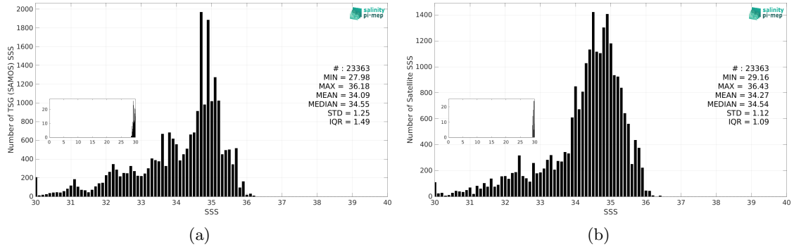
Figure 3: Histograms of SSS from TSG (SAMOS) (a) and SMOS SSS L3 Arctic v2 - 9 Days (CATDS-CEC-LOCEAN) (b) considering all match-up pairs per bins of 0.1 over the North Atlantic Ocean Pi-MEP region and for the full satellite product period.
