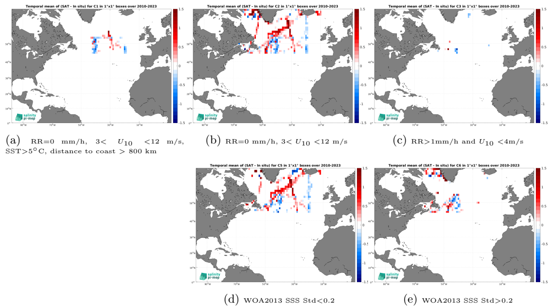
Figure 14: Temporal mean gridded over spatial boxes of size 1^\circ \times 1^\circ of \Delta\text{SSS} (SMOS SSS L3 Arctic v2 - 9 Days (CATDS-CEC-LOCEAN) - TSG (SAMOS)) for 5 different subdatasets corresponding to:RR=0 mm/h, 3 < U_{10} < 12 m/s, SST >5^\circ\text{C} , distance to coast > 800 km (a), RR=0 mm/h, 3 < U_{10} < 12 m/s (b), RR >1 mm/h and U_{10} < 4 m/s (c), WOA2013 SSS Std <0.2 (d), WOA2013 SSS Std >0.2 (e).
