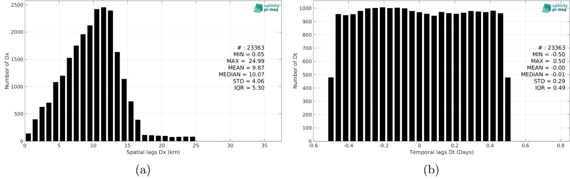
Figure 5: Histograms of the spatial (a) and temporal (b) lags between the location/time of the TSG (SAMOS) measurement and the date of the corresponding SMOS SSS L3 Arctic v2 - 9 Days (CATDS-CEC-LOCEAN) SSS pixel.
