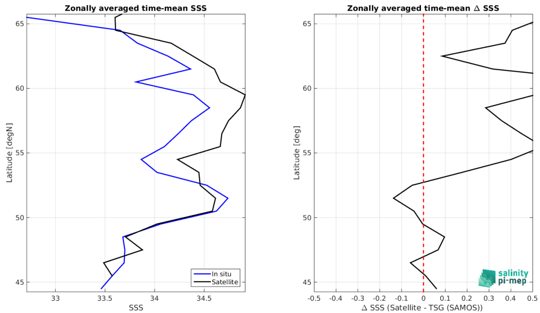
Figure 8: Left panel: Zonal mean SSS from SMOS SSS L3 Arctic v2 - 9 Days (CATDS-CEC-LOCEAN) satellite product (black) and from TSG (SAMOS) (blue). Right panel: Zonal mean of \Delta SSS (Satellite - TSG (SAMOS)) for all the collected Pi-MEP match-up pairs estimated over the full satellite product period.
