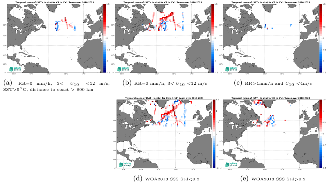
Figure 12: Temporal mean gridded over spatial boxes of size 1^{\circ}\times 1^{\circ} of \Delta\text{SSS} (SMOS SSS L3 Arctic v2 - 9 Days (CATDS-CEC-LOCEAN) - TSG (SAMOS)) for 5 different subdatasets corresponding to: RR=0 mm/h, 3 < U_{10} < 12 m/s, SST > 5^{\circ}\text{C} , distance to coast > 800 km (a), RR=0 mm/h, 3 < U_{10} < 12 m/s (b), RR > 1 mm/h and U_{10} < 4 m/s (c), WOA2013 SSS Std < 0.2 (d), WOA2013 SSS Std > 0.2 (e).
