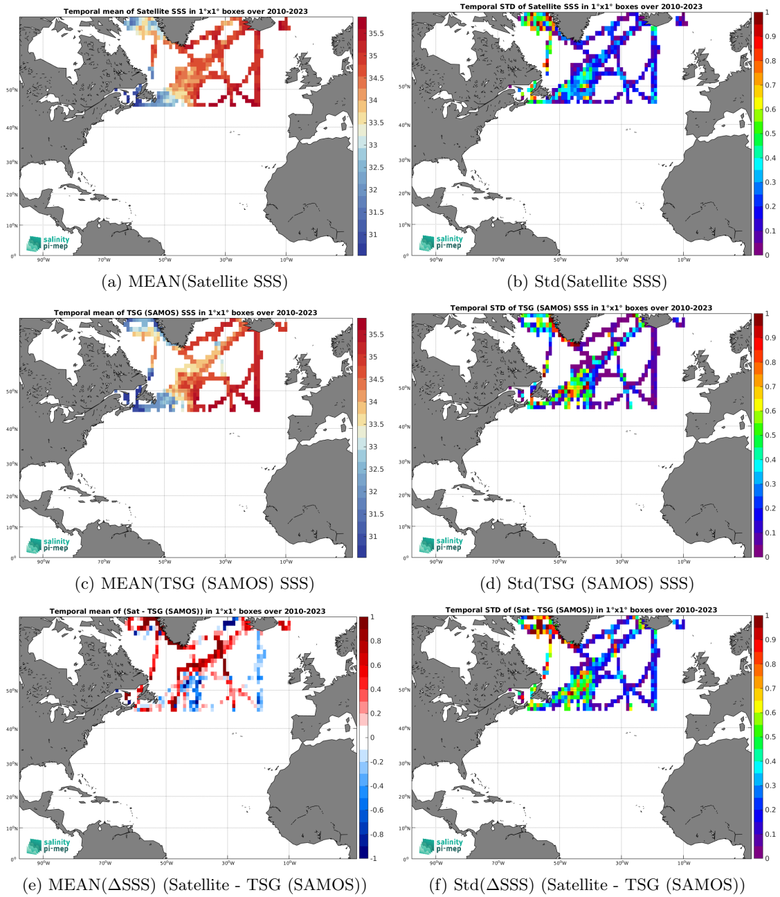
Figure 6: Temporal mean (left) and Std (right) of SSS from SMOS SSS L3 Arctic v2 - 9 Days (CATDS-CEC-LOCEAN) (top), TSG (SAMOS) (middle), and of \Delta SSS (Satellite - TSG (SAMOS)). Only match-up pairs are used to generate these maps.
