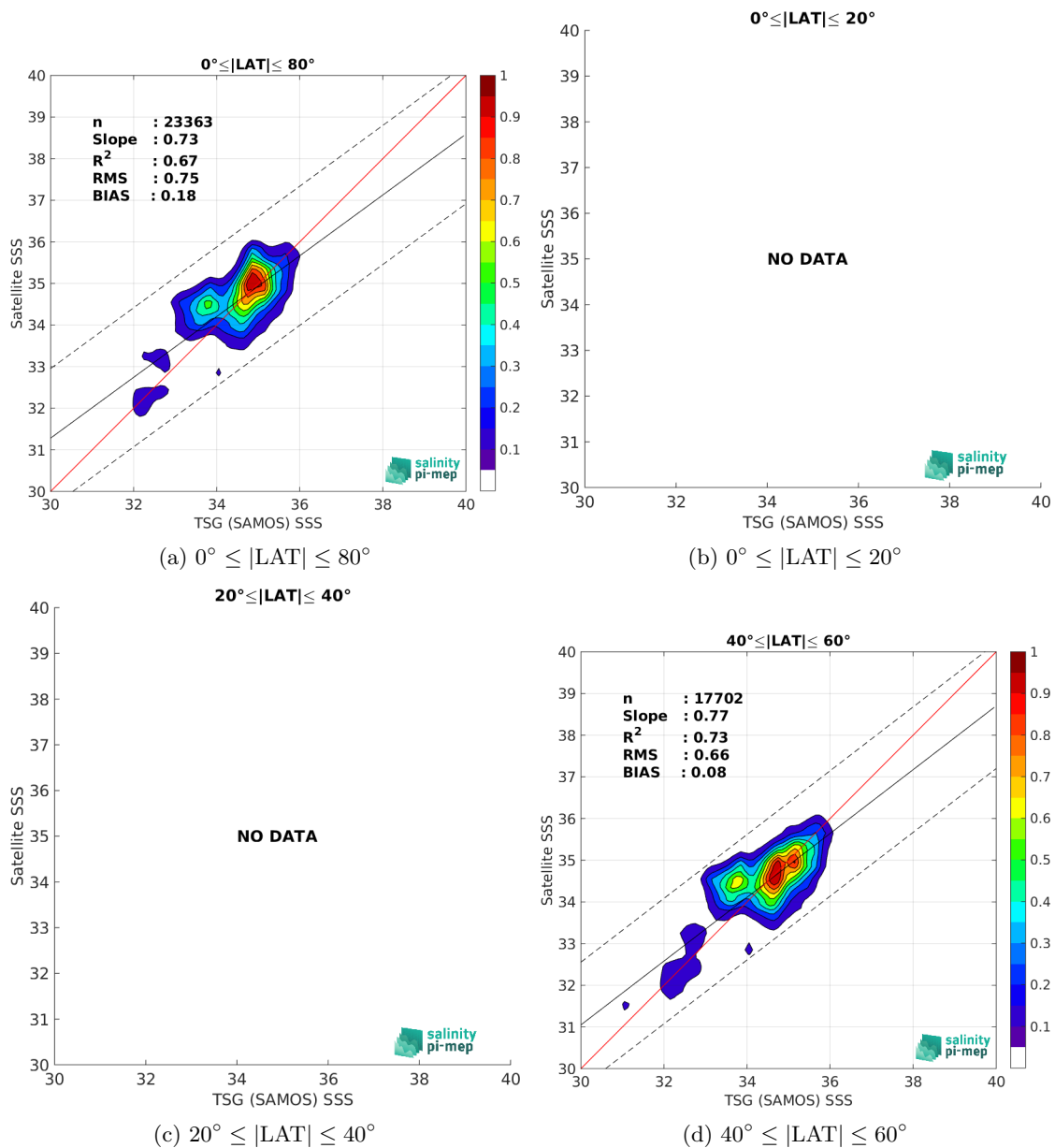
Figure 9: Contour maps of the concentration of SMOS SSS L3 Arctic v2 - 9 Days (CATDS-CEC-LOCEAN) SSS (y-axis) versus TSG (SAMOS) SSS (x-axis) at match-up pairs for different latitude bands. For each plot, the red line shows x=y . The black thin and dashed lines indicate a linear fit through the data cloud and the \pm 95\% confidence levels, respectively. The number match-up pairs n , the slope and R^2 coefficient of the linear fit, the root mean square (RMS) and the mean bias between satellite and in situ data are indicated for each latitude band in each plots.
