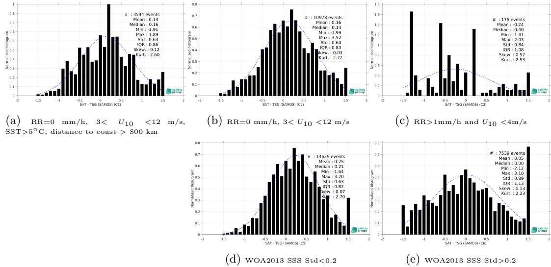
Figure 13: Normalized histogram of \Delta SSS (SMOS SSS L3 Arctic v2 - 9 Days (CATDS-CEC-LOCEAN) - TSG (SAMOS)) for 5 different subdatasets corresponding to: RR=0 mm/h, 3 < U_{10} < 12 m/s, SST>5°C, distance to coast > 800 km (a), RR=0 mm/h, 3 < U_{10} < 12 m/s (b), RR>1mm/h and U_{10} < 4 m/s (c), WOA2013 SSS Std<0.2 (d), WOA2013 SSS Std>0.2 (e).
