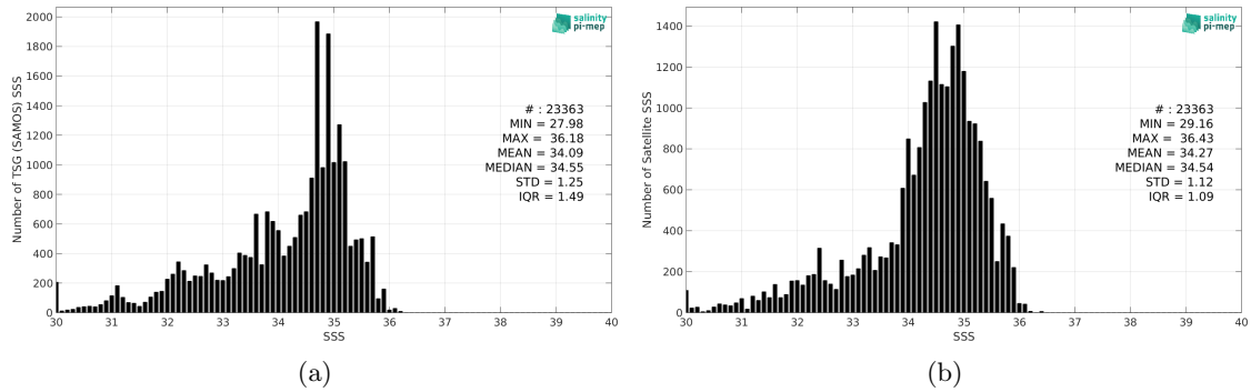
Figure 2: Histograms of SSS from TSG (SAMOS) (a) and SMOS SSS L3 Arctic v2 - 9 Days (CATDS-CEC-LOCEAN) (b) considering all match-up pairs per bins of 0.1 over the North Atlantic Ocean Pi-MEP region and for the full satellite product period.
