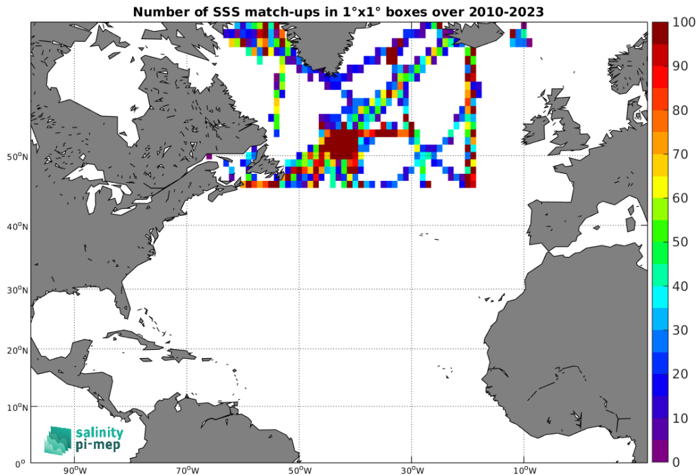
Figure 4: Number of SSS match-ups between TSG (SAMOS) SSS and the SMOS SSS L3 Arctic v2 - 9 Days (CATDS-CEC-LOCEAN) SSS product for the North Atlantic Ocean Pi-MEP region over 1^\circ \times 1^\circ boxes and for the full satellite product period.
