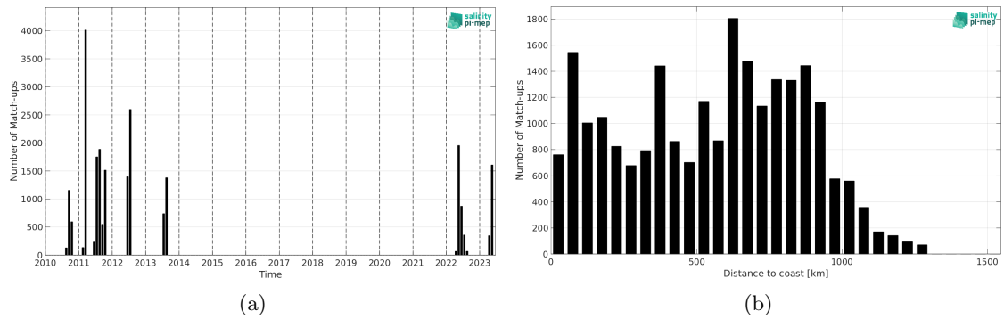
Figure 1: Number of match-ups between TSG (SAMOS) and SMOS SSS L3 Arctic v2 - 9 Days (CATDS-CEC-LOCEAN) SSS as a function of time (a) and as function of the distance to coast (b) over the North Atlantic Ocean Pi-MEP region and for the full satellite product period.
