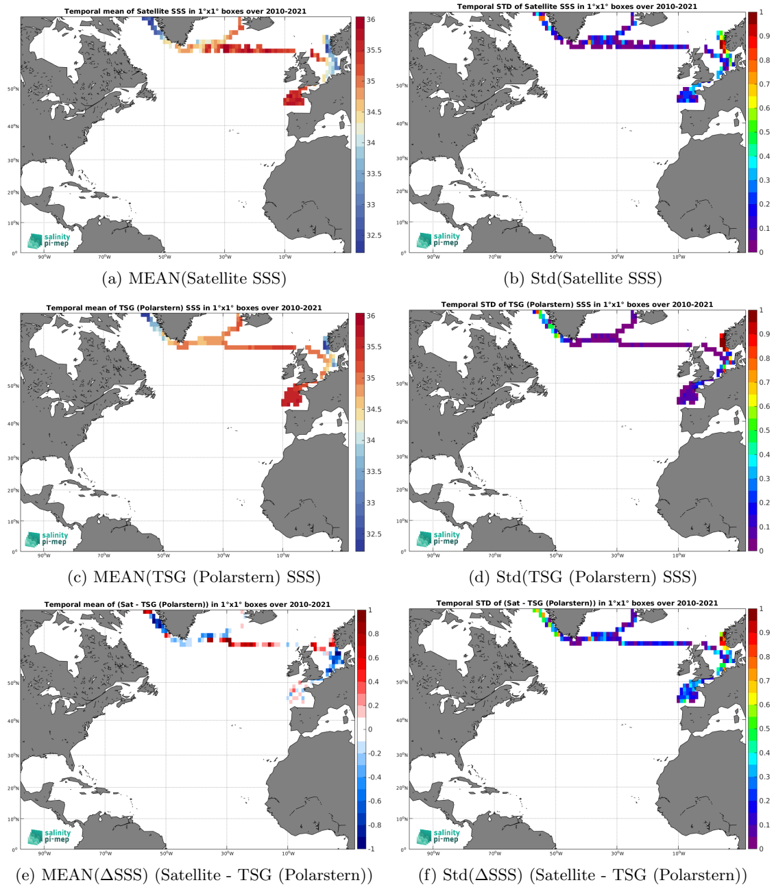
Figure 6: Temporal mean (left) and Std (right) of SSS from SMOS SSS L3 Arctic v2 - 9 Days (CATDS-CEC-LOCEAN) (top), TSG (Polarstern) (middle), and of \Delta SSS (Satellite - TSG (Polarstern)). Only match-up pairs are used to generate these maps.
