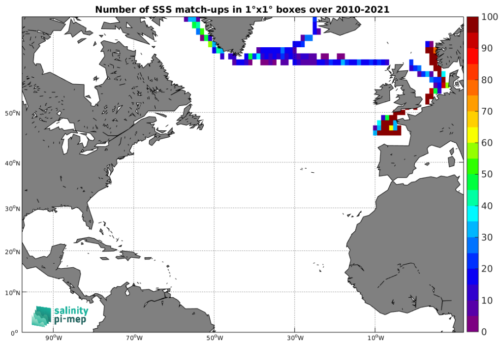
Figure 4: Number of SSS match-ups between TSG (Polarstern) SSS and the SMOS SSS L3 Arctic v2 - 9 Days (CATDS-CEC-LOCEAN) SSS product for the North Atlantic Ocean Pi-MEP region over 1^\circ \times 1^\circ boxes and for the full satellite product period.
