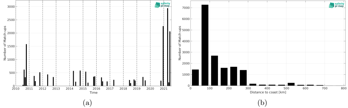
Figure 1: Number of match-ups between TSG (Polarstern) and SMOS SSS L3 Arctic v2 - 9 Days (CATDS-CEC-LOCEAN) SSS as a function of time (a) and as function of the distance to coast (b) over the North Atlantic Ocean Pi-MEP region and for the full satellite product period.
