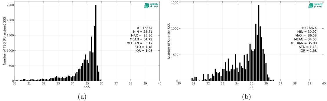
Figure 2: Histograms of SSS from TSG (Polarstern) (a) and SMOS SSS L3 Arctic v2 - 9 Days (CATDS-CEC-LOCEAN) (b) considering all match-up pairs per bins of 0.1 over the North Atlantic Ocean Pi-MEP region and for the full satellite product period.
