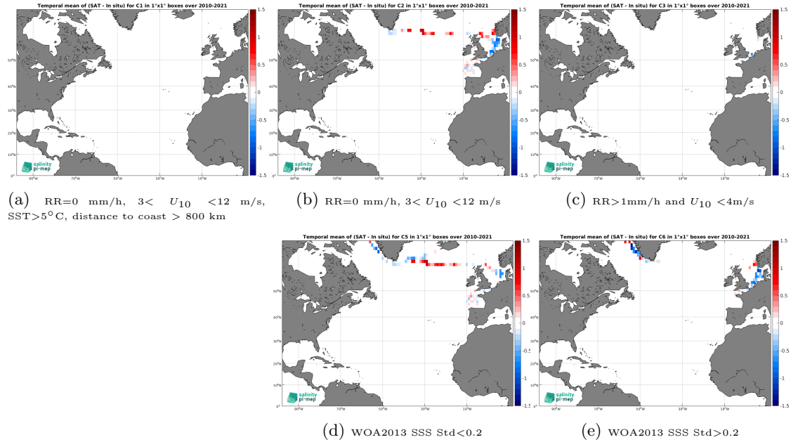
Figure 12: Temporal mean gridded over spatial boxes of size 1^{\circ}\times 1^{\circ} of \Delta\text{SSS} (SMOS SSS L3 Arctic v2 - 9 Days (CATDS-CEC-LOCEAN) - TSG (Polarstern)) for 5 different subdatasets corresponding to: RR=0 mm/h, 3 < U_{10} < 12 m/s, SST > 5^{\circ}\text{C} , distance to coast > 800 km (a), RR=0 mm/h, 3 < U_{10} < 12 m/s (b), RR > 1 mm/h and U_{10} < 4 m/s (c), WOA2013 SSS Std < 0.2 (d), WOA2013 SSS Std > 0.2 (e).
