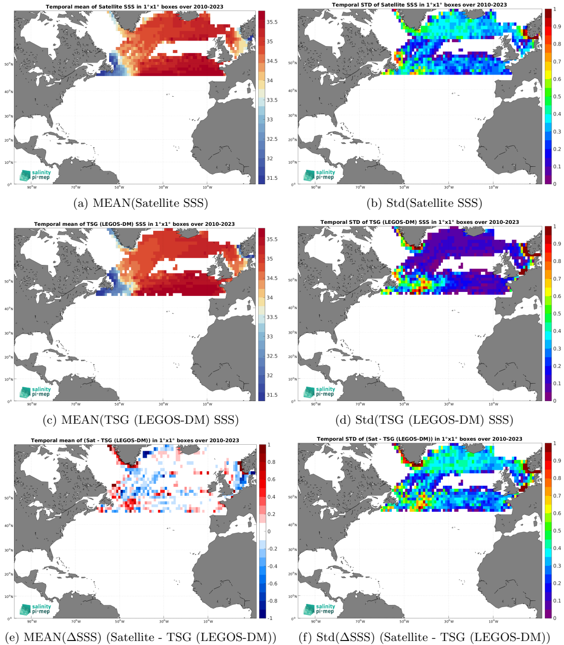
Figure 7: Temporal mean (left) and Std (right) of SSS from SMOS SSS L3 Arctic v2 - 9 Days (CATDS-CEC-LOCEAN) (top), TSG (LEGOS-DM) (middle), and of \Delta SSS (Satellite - TSG (LEGOS-DM)). Only match-up pairs are used to generate these maps.
