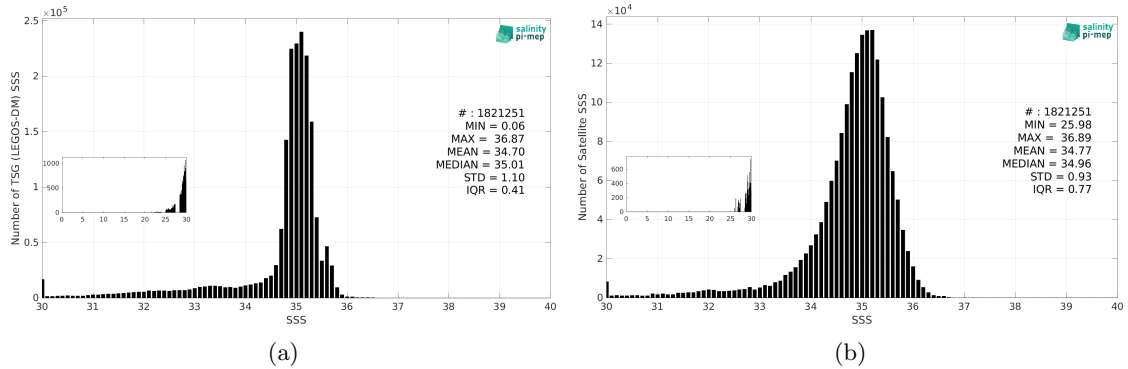
Figure 3: Histograms of SSS from TSG (LEGOS-DM) (a) and SMOS SSS L3 Arctic v2 - 9 Days (CATDS-CEC-LOCEAN) (b) considering all match-up pairs per bins of 0.1 over the North Atlantic Ocean Pi-MEP region and for the full satellite product period.
