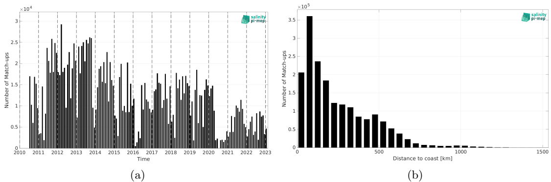
Figure 2: Number of match-ups between TSG (LEGOS-DM) and SMOS SSS L3 Arctic v2 - 9 Days (CATDS-CEC-LOCEAN) SSS as a function of time (a) and as function of the distance to coast (b) over the North Atlantic Ocean Pi-MEP region and for the full satellite product period.
