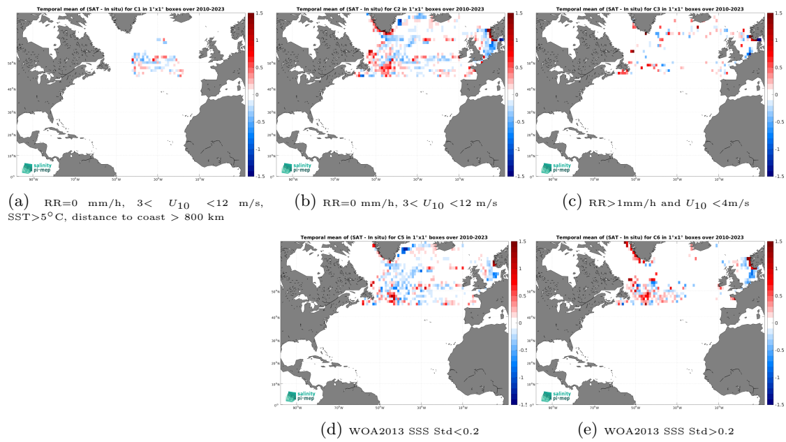
Figure 14: Temporal mean gridded over spatial boxes of size 1^\circ \times 1^\circ of \Delta\text{SSS} (SMOS SSS L3 Arctic v2 - 9 Days (CATDS-CEC-LOCEAN) - TSG (LEGOS-DM)) for 5 different subdatasets corresponding to:RR=0 mm/h, 3 < U_{10} < 12 m/s, SST >5^\circ\text{C} , distance to coast > 800 km (a), RR=0 mm/h, 3 < U_{10} < 12 m/s (b), RR >1 mm/h and U_{10} < 4 m/s (c), WOA2013 SSS Std <0.2 (d), WOA2013 SSS Std >0.2 (e).
