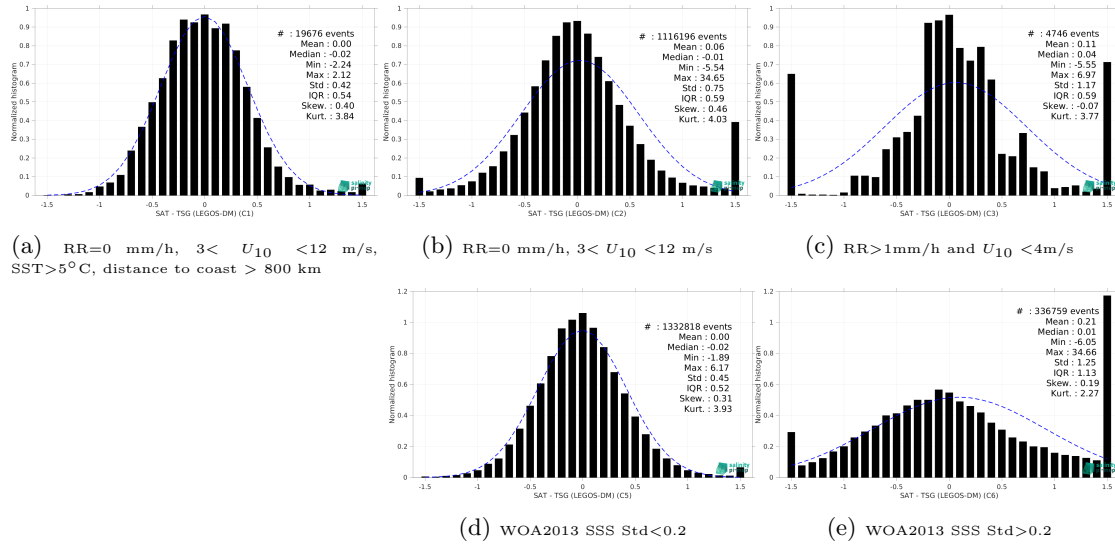
Figure 15: Normalized histogram of \Delta SSS (SMOS SSS L3 Arctic v2 - 9 Days (CATDS-CEC-LOCEAN) - TSG (LEGOS-DM)) for 5 different subdatasets corresponding to: RR=0 mm/h, 3 < U_{10} < 12 m/s, SST>5°C, distance to coast > 800 km (a), RR=0 mm/h, 3 < U_{10} < 12 m/s (b), RR>1mm/h and U_{10} < 4 m/s (c), WOA2013 SSS Std<0.2 (d), WOA2013 SSS Std>0.2 (e).
