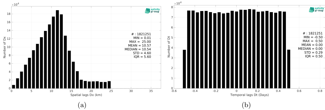
Figure 6: Histograms of the spatial (a) and temporal (b) lags between the location/time of the TSG (LEGOS-DM) measurement and the date of the corresponding SMOS SSS L3 Arctic v2 - 9 Days (CATDS-CEC-LOCEAN) SSS pixel.
