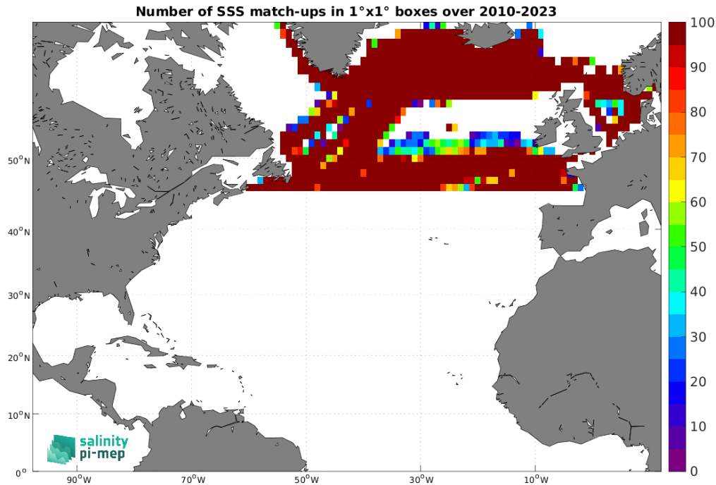
Figure 5: Number of SSS match-ups between TSG (LEGOS-DM) SSS and the SMOS SSS L3 Arctic v2 - 9 Days (CATDS-CEC-LOCEAN) SSS product for the North Atlantic Ocean Pi-MEP region over 1^\circ \times 1^\circ boxes and for the full satellite product period.
