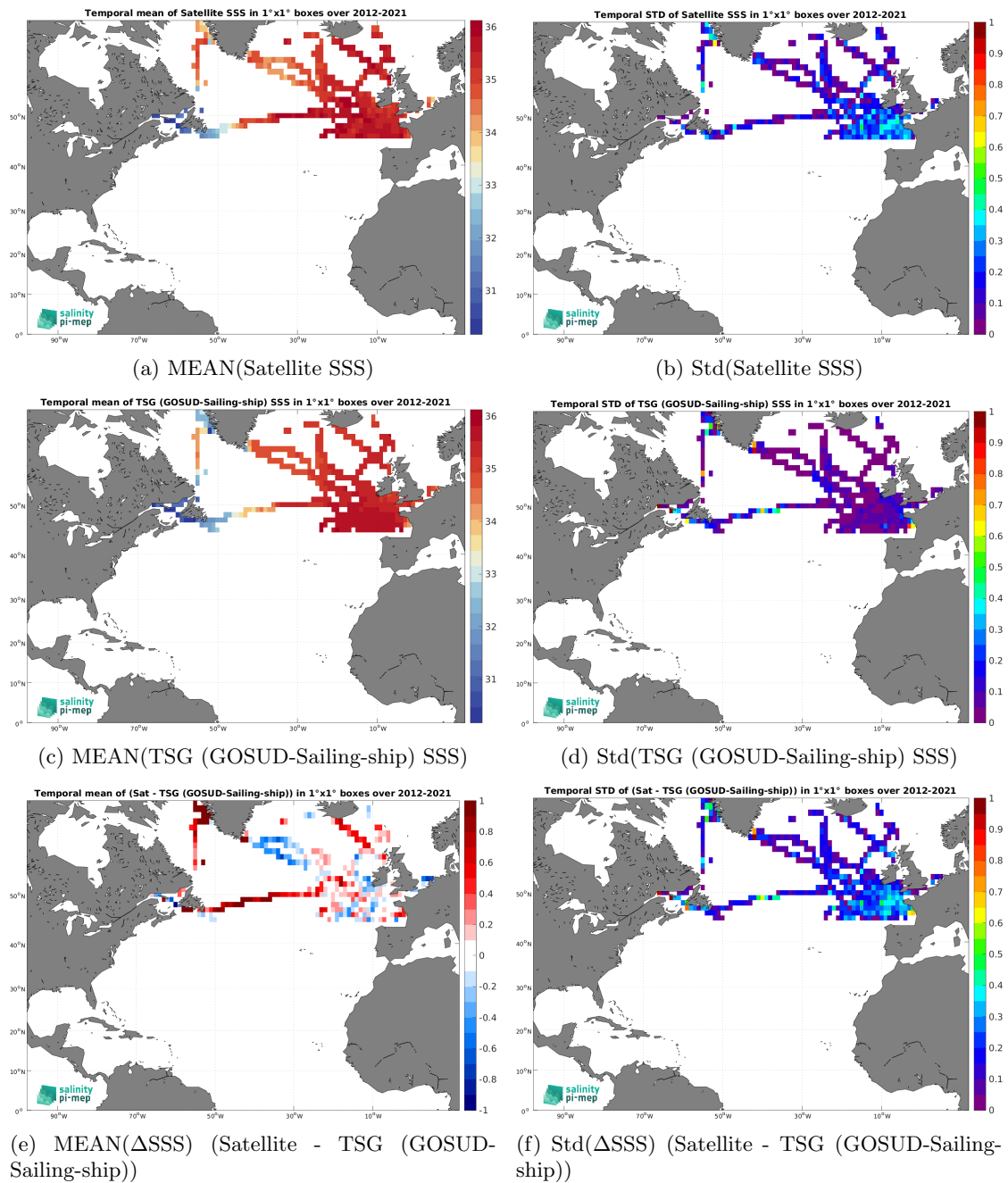
Figure 7: Temporal mean (left) and Std (right) of SSS from SMOS SSS L3 Arctic v2 - 9 Days (CATDS-CEC-LOCEAN) (top), TSG (GOSUD-Sailing-ship) (middle), and of \Delta SSS (Satellite - TSG (GOSUD-Sailing-ship)). Only match-up pairs are used to generate these maps.
