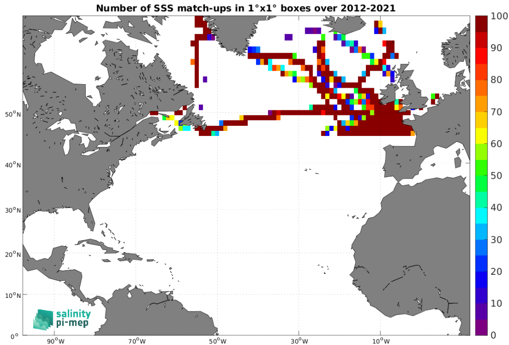
Figure 5: Number of SSS match-ups between TSG (GOSUD-Sailing-ship) SSS and the SMOS SSS L3 Arctic v2 - 9 Days (CATDS-CEC-LOCEAN) SSS product for the North Atlantic Ocean Pi-MEP region over 1^\circ \times 1^\circ boxes and for the full satellite product period.
