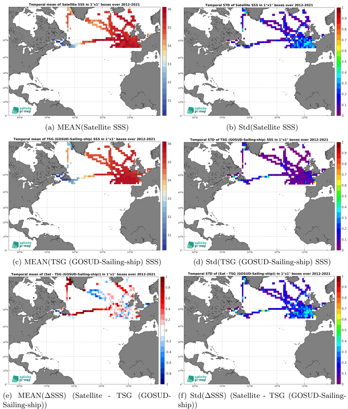
Figure 6: Temporal mean (left) and Std (right) of SSS from SMOS SSS L3 Arctic v2 - 9 Days (CATDS-CEC-LOCEAN) (top), TSG (GOSUD-Sailing-ship) (middle), and of \Delta SSS (Satellite - TSG (GOSUD-Sailing-ship)). Only match-up pairs are used to generate these maps.
