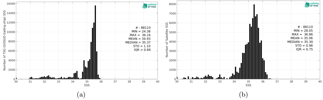
Figure 2: Histograms of SSS from TSG (GOSUD-Sailing-ship) (a) and SMOS SSS L3 Arctic v2 - 9 Days (CATDS-CEC-LOCEAN) (b) considering all match-up pairs per bins of 0.1 over the North Atlantic Ocean Pi-MEP region and for the full satellite product period.
