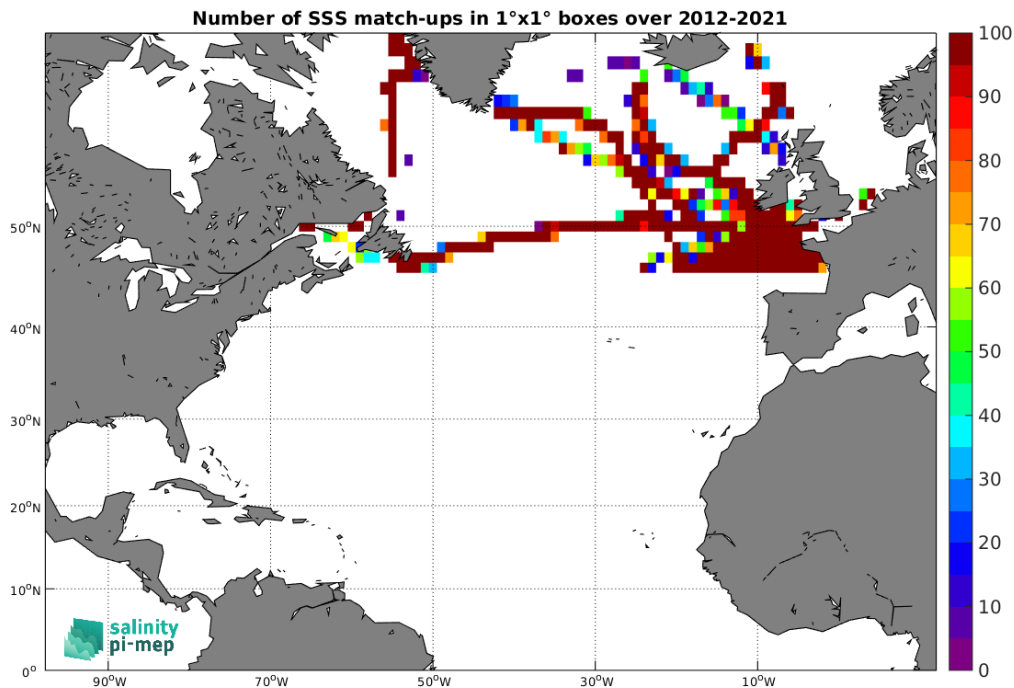
Figure 4: Number of SSS match-ups between TSG (GOSUD-Sailing-ship) SSS and the SMOS SSS L3 Arctic v2 - 9 Days (CATDS-CEC-LOCEAN) SSS product for the North Atlantic Ocean Pi-MEP region over 1^\circ \times 1^\circ boxes and for the full satellite product period.
