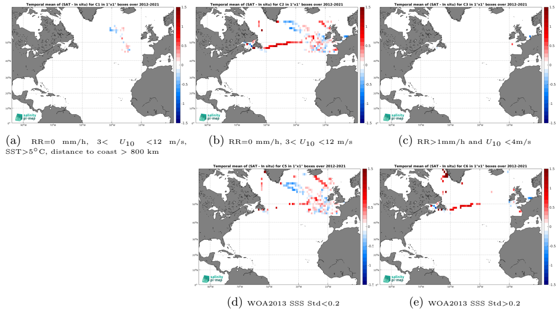
Figure 12: Temporal mean gridded over spatial boxes of size 1^{\circ}\times 1^{\circ} of \Delta SSS (SMOS SSS L3 Arctic v2 - 9 Days (CATDS-CEC-LOCEAN) - TSG (GOSUD-Sailing-ship)) for 5 different subdatasets corresponding to:RR=0 mm/h, 3 < U_{10} < 12 m/s, SST >5^{\circ}\text{C} , distance to coast > 800 km (a), RR=0 mm/h, 3 < U_{10} < 12 m/s (b), RR >1 mm/h and U_{10} < 4 m/s (c), WOA2013 SSS Std <0.2 (d), WOA2013 SSS Std >0.2 (e).
