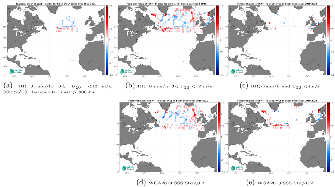
Figure 14: Temporal mean gridded over spatial boxes of size 1^\circ \times 1^\circ of \Delta SSS (SMOS SSS L3 Arctic v2 - 9 Days (CATDS-CEC-LOCEAN) - TSG (GOSUD-Research-vessel)) for 5 different subdatasets corresponding to:RR=0 mm/h, 3 < U_{10} < 12 m/s, SST >5^\circ\text{C} , distance to coast > 800 km (a), RR=0 mm/h, 3 < U_{10} < 12 m/s (b), RR >1 mm/h and U_{10} < 4 m/s (c), WOA2013 SSS Std <0.2 (d), WOA2013 SSS Std >0.2 (e).
