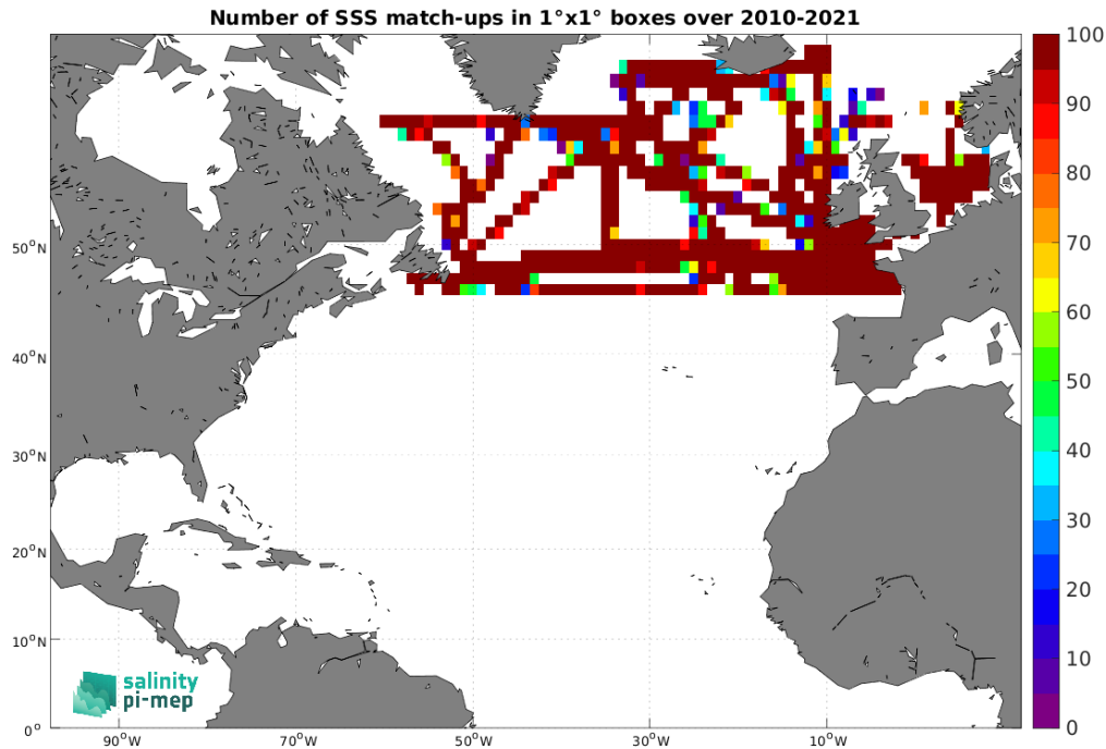
Figure 5: Number of SSS match-ups between TSG (GOSUD-Research-vessel) SSS and the SMOS SSS L3 Arctic v2 - 9 Days (CATDS-CEC-LOCEAN) SSS product for the North Atlantic Ocean Pi-MEP region over 1^\circ \times 1^\circ boxes and for the full satellite product period.
