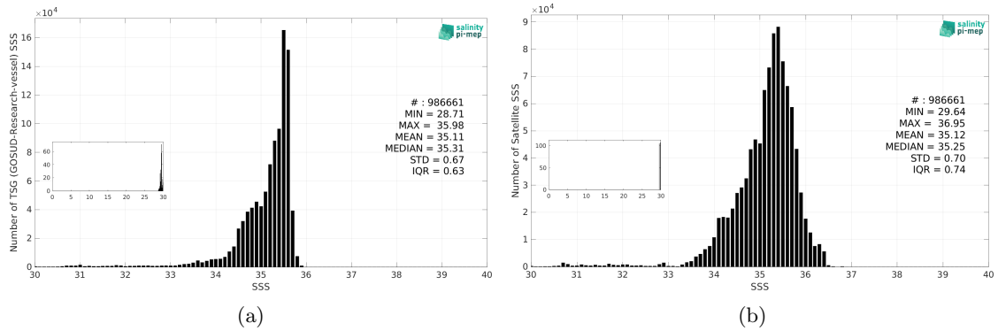
Figure 3: Histograms of SSS from TSG (GOSUD-Research-vessel) (a) and SMOS SSS L3 Arctic v2 - 9 Days (CATDS-CEC-LOCEAN) (b) considering all match-up pairs per bins of 0.1 over the North Atlantic Ocean Pi-MEP region and for the full satellite product period.
