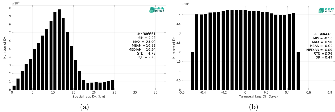
Figure 6: Histograms of the spatial (a) and temporal (b) lags between the location/time of the TSG (GOSUD-Research-vessel) measurement and the date of the corresponding SMOS SSS L3 Arctic v2 - 9 Days (CATDS-CEC-LOCEAN) SSS pixel.
