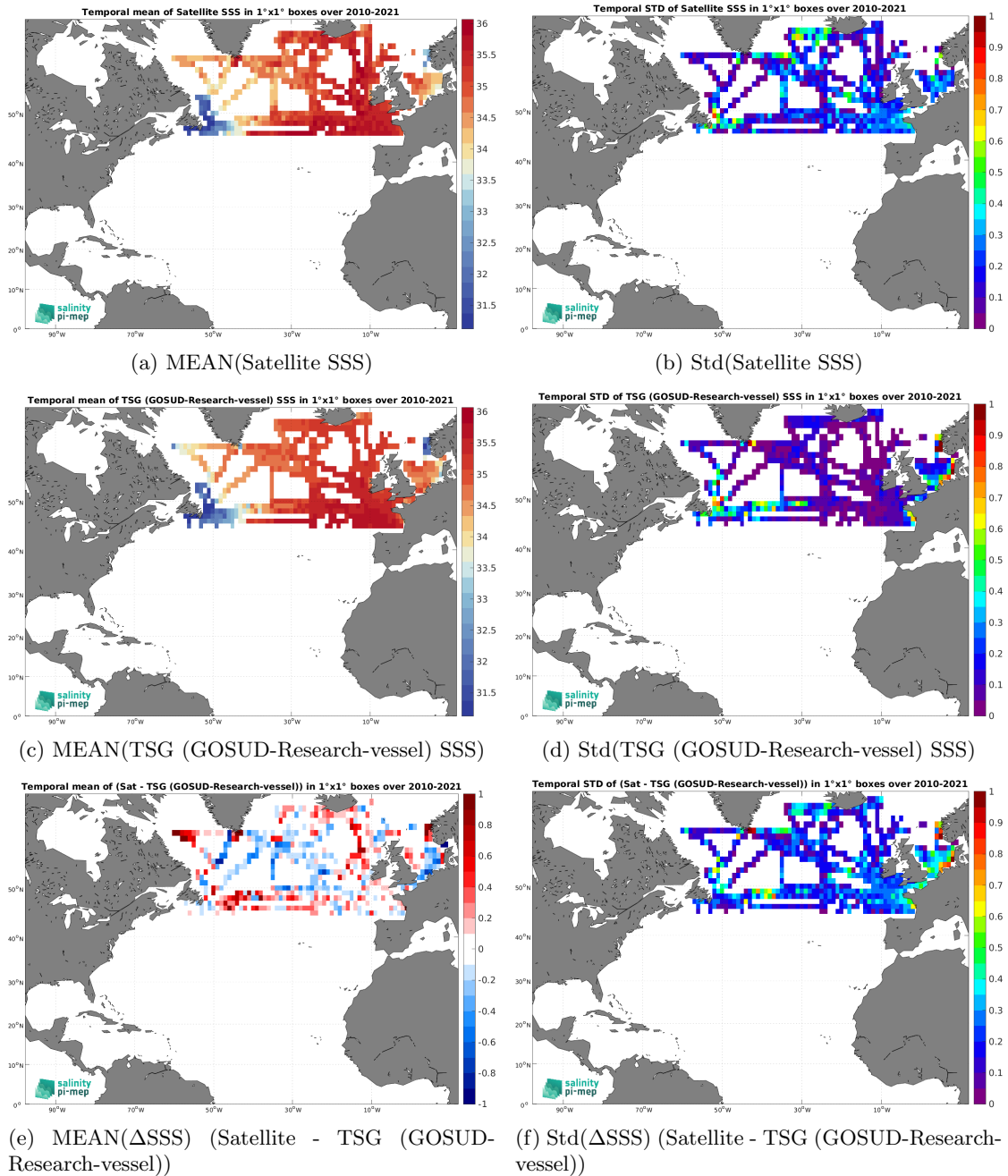
Figure 7: Temporal mean (left) and Std (right) of SSS from SMOS SSS L3 Arctic v2 - 9 Days (CATDS-CEC-LOCEAN) (top), TSG (GOSUD-Research-vessel) (middle), and of \Delta SSS (Satellite - TSG (GOSUD-Research-vessel)). Only match-up pairs are used to generate these maps.
