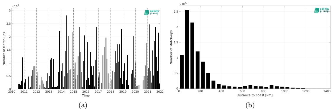
Figure 2: Number of match-ups between TSG (GOSUD-Research-vessel) and SMOS SSS L3 Arctic v2 - 9 Days (CATDS-CEC-LOCEAN) SSS as a function of time (a) and as function of the distance to coast (b) over the North Atlantic Ocean Pi-MEP region and for the full satellite product period.
