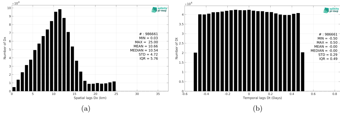
Figure 5: Histograms of the spatial (a) and temporal (b) lags between the location/time of the TSG (GOSUD-Research-vessel) measurement and the date of the corresponding SMOS SSS L3 Arctic v2 - 9 Days (CATDS-CEC-LOCEAN) SSS pixel.
