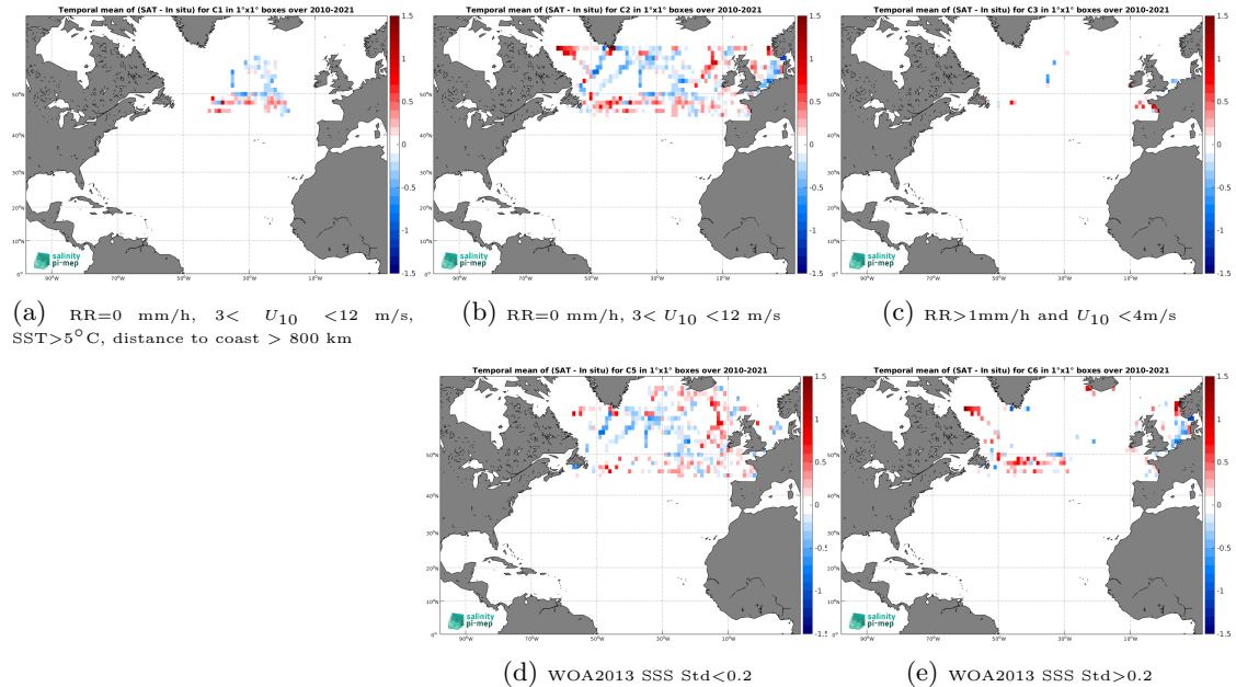
Figure 12: Temporal mean gridded over spatial boxes of size 1^{\circ}\times 1^{\circ} of \Delta SSS (SMOS SSS L3 Arctic v2 - 9 Days (CATDS-CEC-LOCEAN) - TSG (GOSUD-Research-vessel)) for 5 different subdatasets corresponding to:RR=0 mm/h, 3 < U_{10} < 12 m/s, SST >5^{\circ}\text{C} , distance to coast > 800 km (a), RR=0 mm/h, 3 < U_{10} < 12 m/s (b), RR >1 mm/h and U_{10} < 4 m/s (c), WOA2013 SSS Std <0.2 (d), WOA2013 SSS Std >0.2 (e).
