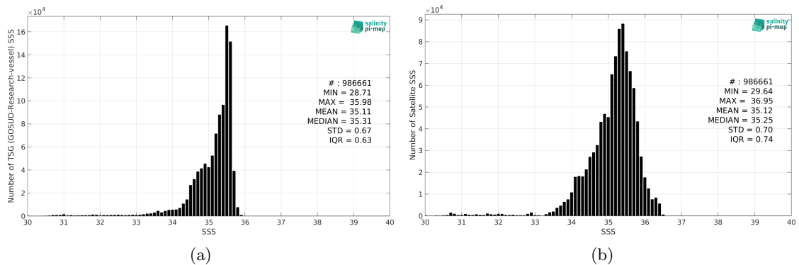
Figure 2: Histograms of SSS from TSG (GOSUD-Research-vessel) (a) and SMOS SSS L3 Arctic v2 - 9 Days (CATDS-CEC-LOCEAN) (b) considering all match-up pairs per bins of 0.1 over the North Atlantic Ocean Pi-MEP region and for the full satellite product period.
