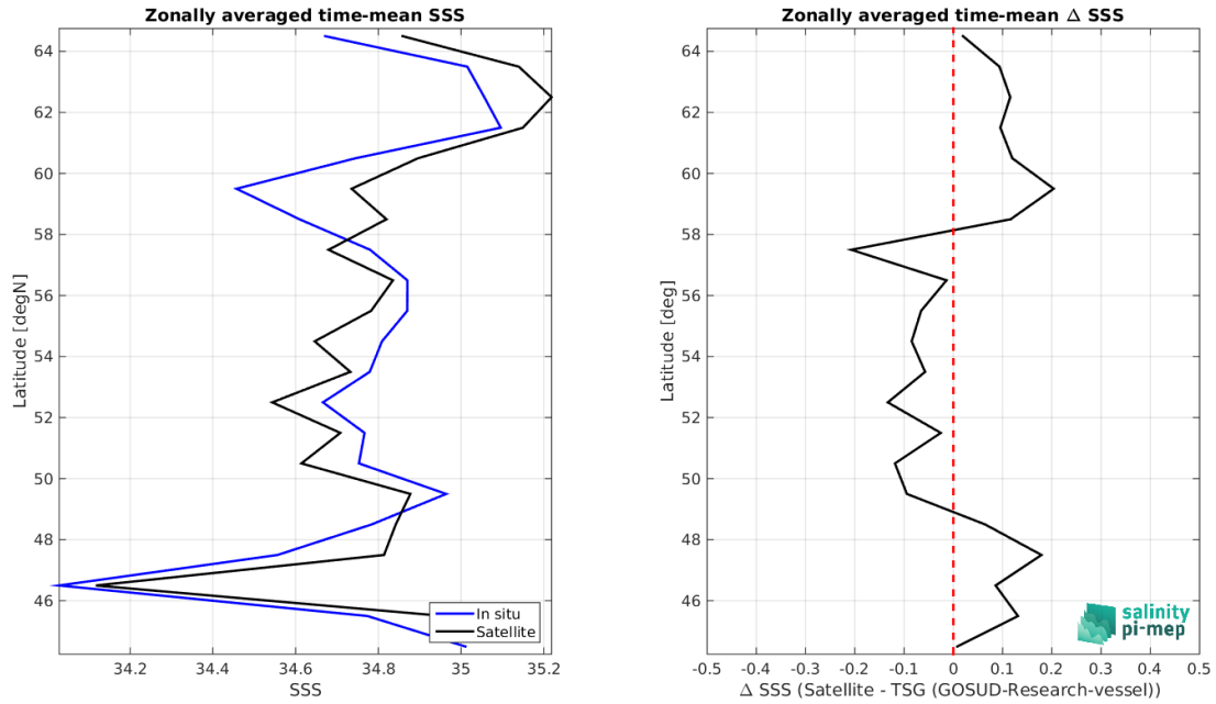
Figure 8: Left panel: Zonal mean SSS from SMOS SSS L3 Arctic v2 - 9 Days (CATDS-CEC-LOCEAN) satellite product (black) and from TSG (GOSUD-Research-vessel) (blue). Right panel: Zonal mean of \Delta SSS (Satellite - TSG (GOSUD-Research-vessel)) for all the collected Pi-MEP match-up pairs estimated over the full satellite product period.
