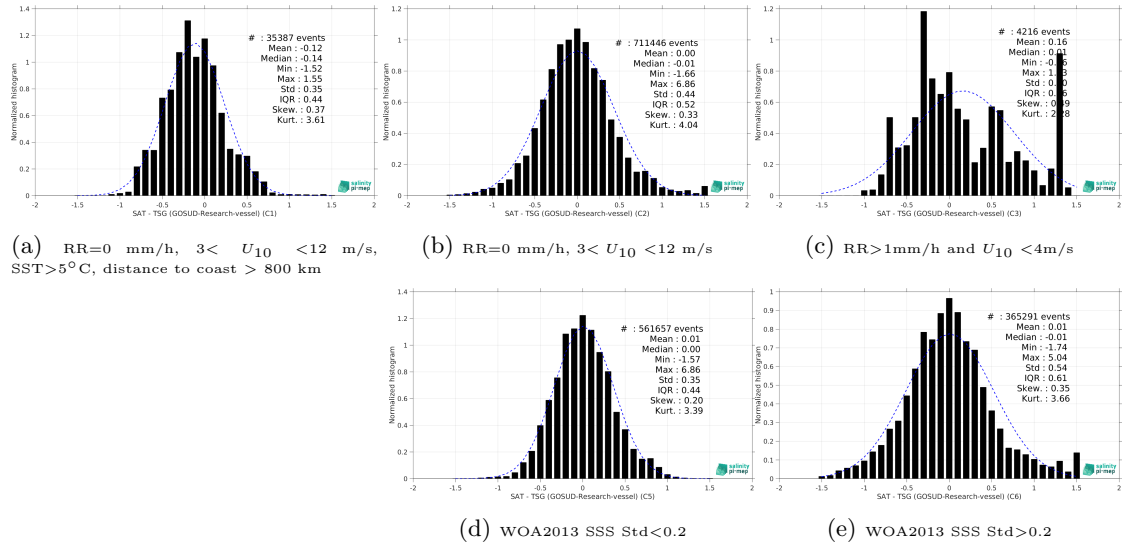
Figure 13: Normalized histogram of \Delta SSS (SMOS SSS L3 Arctic v2 - 9 Days (CATDS-CEC-LOCEAN) - TSG (GOSUD-Research-vessel)) for 5 different subdatasets corresponding to: RR=0 mm/h, 3 < U_{10} < 12 m/s, SST>5°C, distance to coast > 800 km (a), RR=0 mm/h, 3 < U_{10} < 12 m/s (b), RR>1mm/h and U_{10} < 4 m/s (c), WOA2013 SSS Std<0.2 (d), WOA2013 SSS Std>0.2 (e).
