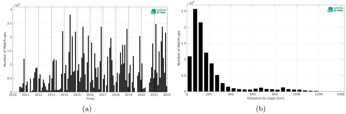
Figure 1: Number of match-ups between TSG (GOSUD-Research-vessel) and SMOS SSS L3 Arctic v2 - 9 Days (CATDS-CEC-LOCEAN) SSS as a function of time (a) and as function of the distance to coast (b) over the North Atlantic Ocean Pi-MEP region and for the full satellite product period.
