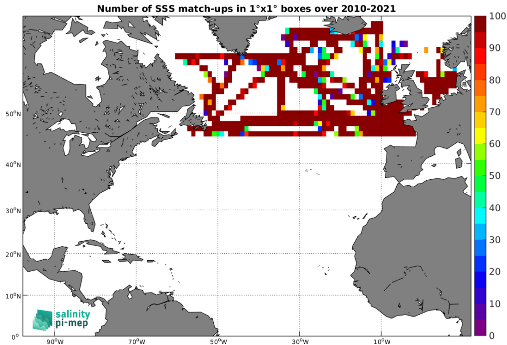
Figure 4: Number of SSS match-ups between TSG (GOSUD-Research-vessel) SSS and the SMOS SSS L3 Arctic v2 - 9 Days (CATDS-CEC-LOCEAN) SSS product for the North Atlantic Ocean Pi-MEP region over 1^\circ \times 1^\circ boxes and for the full satellite product period.
