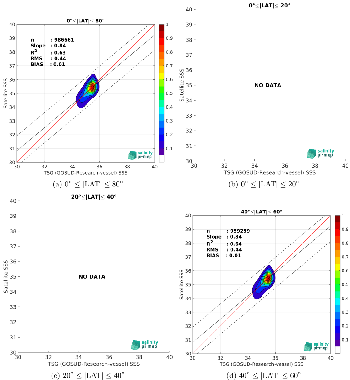
Figure 9: Contour maps of the concentration of SMOS SSS L3 Arctic v2 - 9 Days (CATDS-CEC-LOCEAN) SSS (y-axis) versus TSG (GOSUD-Research-vessel) SSS (x-axis) at match-up pairs for different latitude bands. For each plot, the red line shows x=y . The black thin and dashed lines indicate a linear fit through the data cloud and the \pm 95\% confidence levels, respectively. The number match-up pairs n , the slope and R^2 coefficient of the linear fit, the root mean square (RMS) and the mean bias between satellite and in situ data are indicated for each latitude band in each plots.
