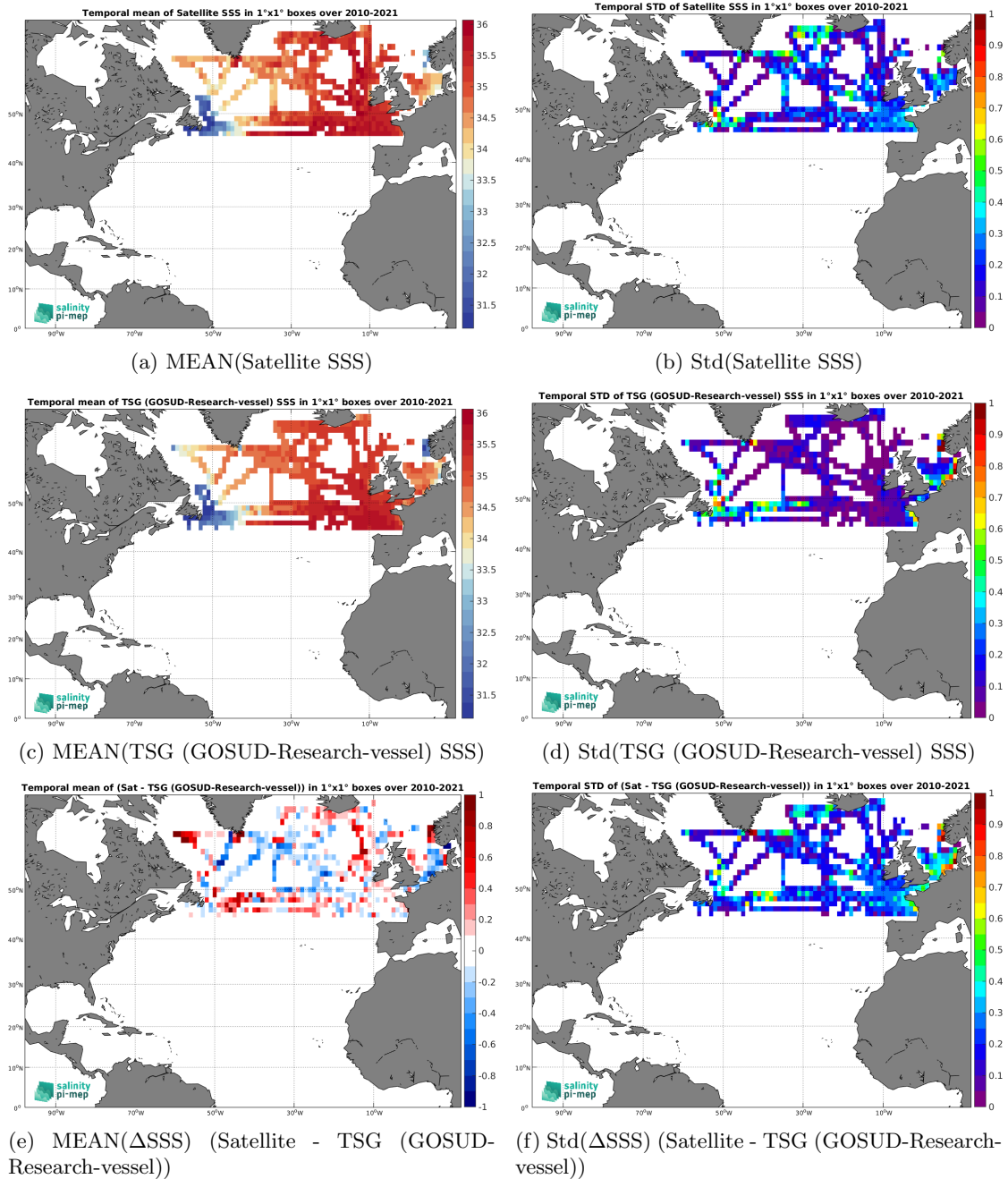
Figure 6: Temporal mean (left) and Std (right) of SSS from SMOS SSS L3 Arctic v2 - 9 Days (CATDS-CEC-LOCEAN) (top), TSG (GOSUD-Research-vessel) (middle), and of \Delta SSS (Satellite - TSG (GOSUD-Research-vessel)). Only match-up pairs are used to generate these maps.
