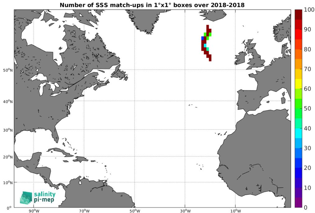
Figure 4: Number of SSS match-ups between TSG (CSIC-UTM) SSS and the SMOS SSS L3 Arctic v2 - 9 Days (CATDS-CEC-LOCEAN) SSS product for the North Atlantic Ocean Pi-MEP region over 1^\circ \times 1^\circ boxes and for the full satellite product period.
