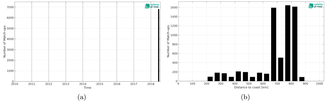
Figure 1: Number of match-ups between TSG (CSIC-UTM) and SMOS SSS L3 Arctic v2 - 9 Days (CATDS-CEC-LOCEAN) SSS as a function of time (a) and as function of the distance to coast (b) over the North Atlantic Ocean Pi-MEP region and for the full satellite product period.
