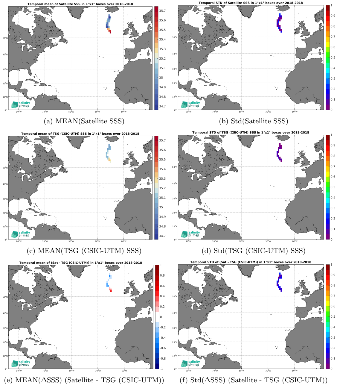
Figure 6: Temporal mean (left) and Std (right) of SSS from SMOS SSS L3 Arctic v2 - 9 Days (CATDS-CEC-LOCEAN) (top), TSG (CSIC-UTM) (middle), and of \Delta SSS (Satellite - TSG (CSIC-UTM)). Only match-up pairs are used to generate these maps.
