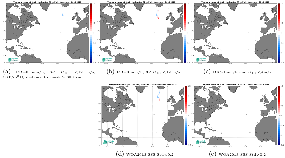
Figure 12: Temporal mean gridded over spatial boxes of size 1^{\circ}\times 1^{\circ} of \Delta\text{SSS} (SMOS SSS L3 Arctic v2 - 9 Days (CATDS-CEC-LOCEAN) - TSG (CSIC-UTM)) for 5 different subdatasets corresponding to:RR=0 mm/h, 3 < U_{10} < 12 m/s, SST > 5^{\circ}\text{C} , distance to coast > 800 km (a), RR=0 mm/h, 3 < U_{10} < 12 m/s (b), RR > 1 mm/h and U_{10} < 4 m/s (c), WOA2013 SSS Std < 0.2 (d), WOA2013 SSS Std > 0.2 (e).
