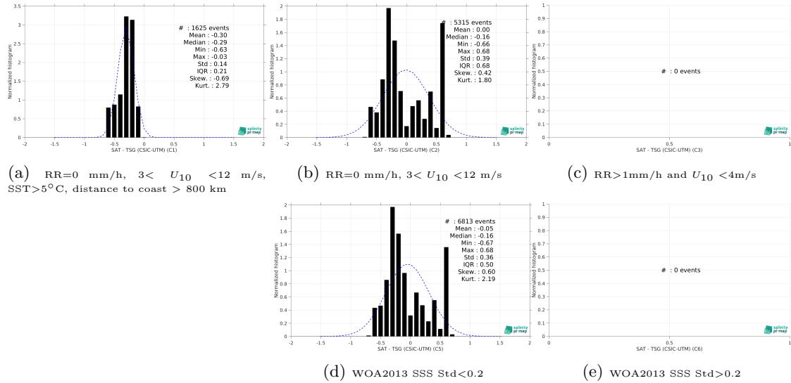
Figure 13: Normalized histogram of \Delta SSS (SMOS SSS L3 Arctic v2 - 9 Days (CATDS-CEC-LOCEAN) - TSG (CSIC-UTM)) for 5 different subdatasets corresponding to: RR=0 mm/h, 3 < U_{10} < 12 m/s, SST > 5°C, distance to coast > 800 km (a), RR=0 mm/h, 3 < U_{10} < 12 m/s (b), RR > 1mm/h and U_{10} < 4 m/s (c), WOA2013 SSS Std < 0.2 (d), WOA2013 SSS Std > 0.2 (e).
