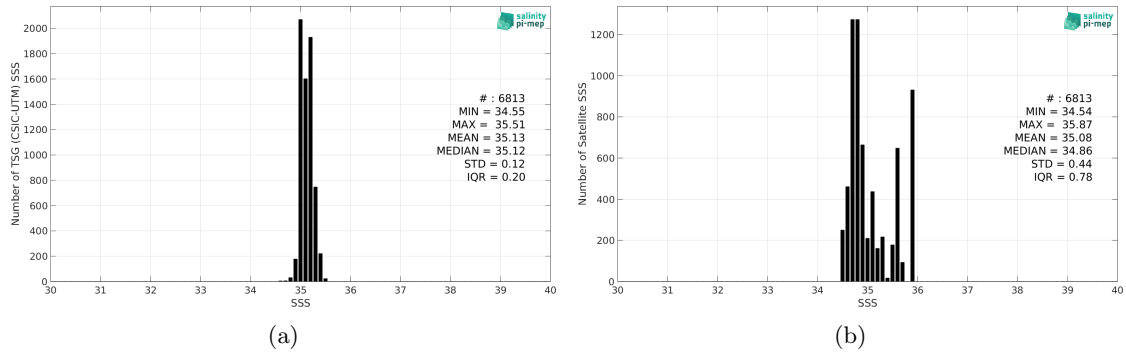
Figure 2: Histograms of SSS from TSG (CSIC-UTM) (a) and SMOS SSS L3 Arctic v2 - 9 Days (CATDS-CEC-LOCEAN) (b) considering all match-up pairs per bins of 0.1 over the North Atlantic Ocean Pi-MEP region and for the full satellite product period.
