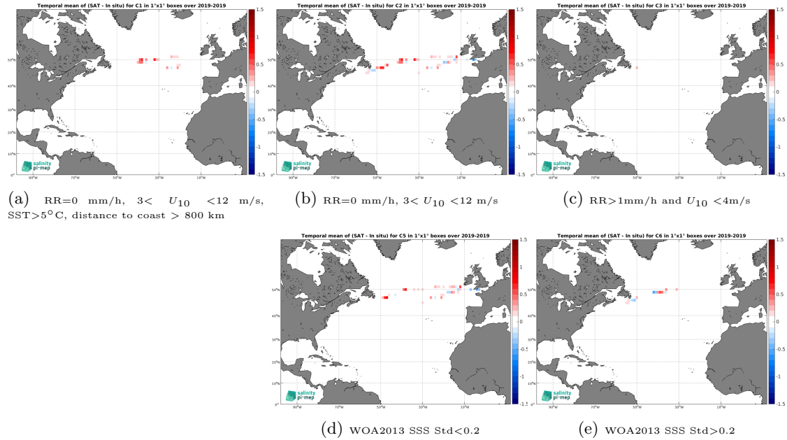
Figure 12: Temporal mean gridded over spatial boxes of size 1^{\circ}\times 1^{\circ} of \Delta\text{SSS} (SMOS SSS L3 Arctic v2 - 9 Days (CATDS-CEC-LOCEAN) - Sairdrone) for 5 different subdatasets corresponding to:RR=0 mm/h, 3 < U_{10} < 12 m/s, SST > 5^{\circ}\text{C} , distance to coast > 800 km (a), RR=0 mm/h, 3 < U_{10} < 12 m/s (b), RR > 1 mm/h and U_{10} < 4 m/s (c), WOA2013 SSS Std < 0.2 (d), WOA2013 SSS Std > 0.2 (e).
