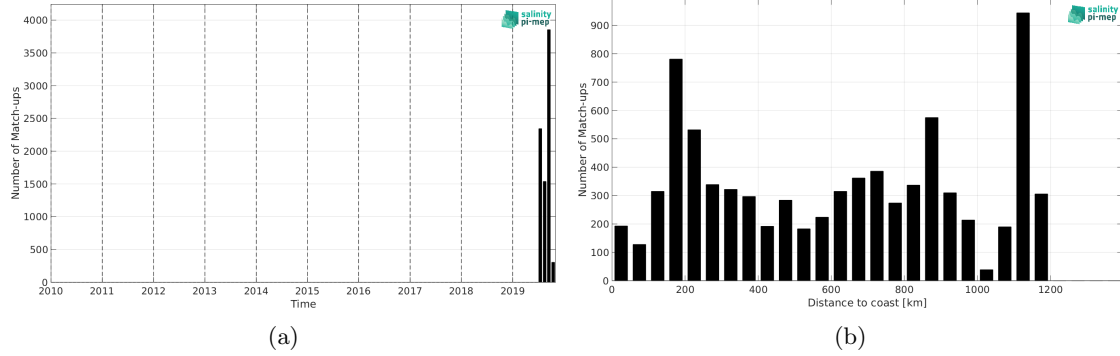
Figure 1: Number of match-ups between Saildrone and SMOS SSS L3 Arctic v2 - 9 Days (CATDS-CEC-LOCEAN) SSS as a function of time (a) and as function of the distance to coast (b) over the North Atlantic Ocean Pi-MEP region and for the full satellite product period.
