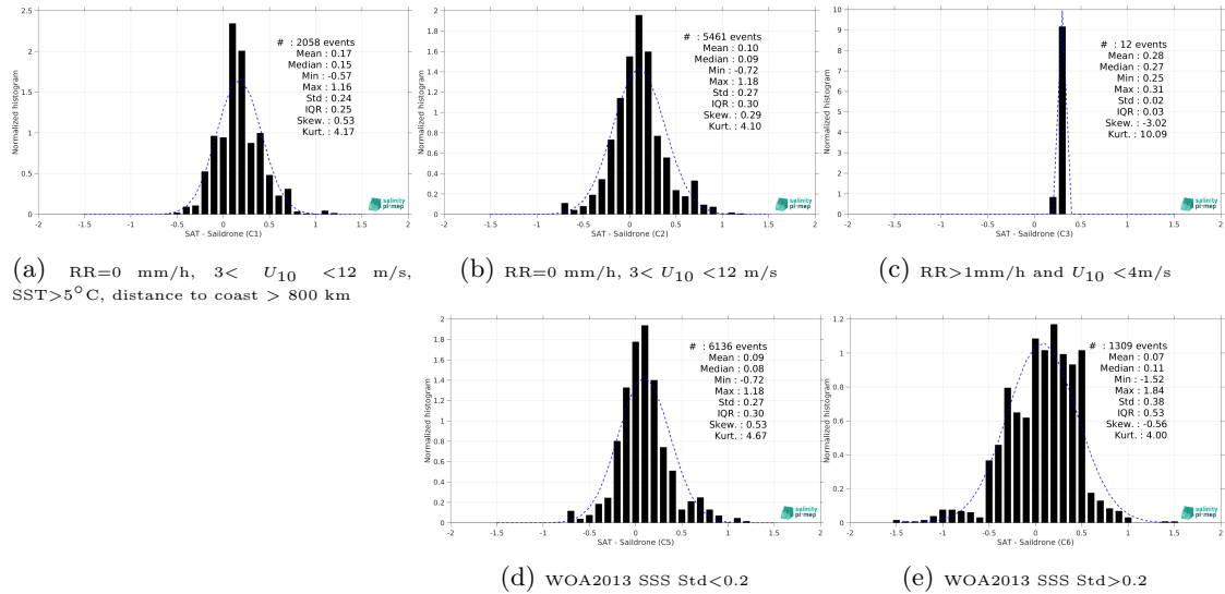
Figure 13: Normalized histogram of \Delta SSS (SMOS SSS L3 Arctic v2 - 9 Days (CATDS-CEC-LOCEAN) - Saildrone) for 5 different subdatasets corresponding to: RR=0 mm/h, 3 < U_{10} < 12 m/s, SST>5°C, distance to coast > 800 km (a), RR=0 mm/h, 3 < U_{10} < 12 m/s (b), RR>1mm/h and U_{10} < 4 m/s (c), WOA2013 SSS Std<0.2 (d), WOA2013 SSS Std>0.2 (e).
