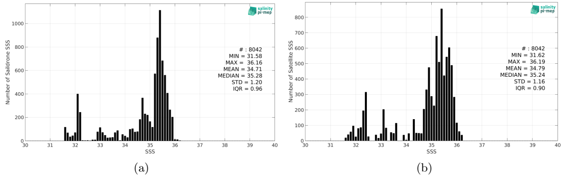
Figure 2: Histograms of SSS from Saildrone (a) and SMOS SSS L3 Arctic v2 - 9 Days (CATDS-CEC-LOCEAN) (b) considering all match-up pairs per bins of 0.1 over the North Atlantic Ocean Pi-MEP region and for the full satellite product period.
