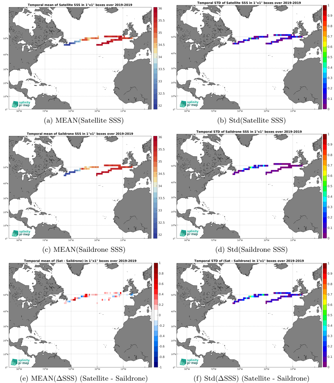
Figure 6: Temporal mean (left) and Std (right) of SSS from SMOS SSS L3 Arctic v2 - 9 Days (CATDS-CEC-LOCEAN) (top), Saildrone (middle), and of \Delta SSS (Satellite - Saildrone). Only match-up pairs are used to generate these maps.
