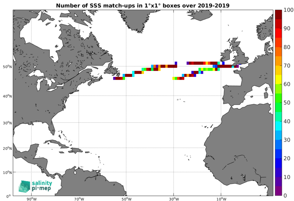
Figure 4: Number of SSS match-ups between Saildrone SSS and the SMOS SSS L3 Arctic v2 - 9 Days (CATDS-CEC-LOCEAN) SSS product for the North Atlantic Ocean Pi-MEP region over 1^\circ \times 1^\circ boxes and for the full satellite product period.
