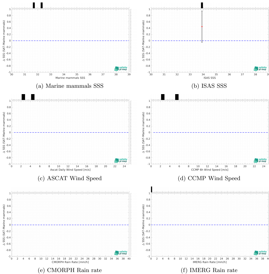
Figure 11: \Delta SSS (Satellite - Marine mammals) sorted as function of Marine mammals SSS values (a), ISAS SSS (b), ASCAT Wind speed (c), CCMP Wind speed (d), CMORPH rain rate (e) and IMERG rain rate (f). In all plots the median and Std of \Delta SSS for each bin is indicated by the red curves and black vertical thick bars ( \pm 1 Std).
