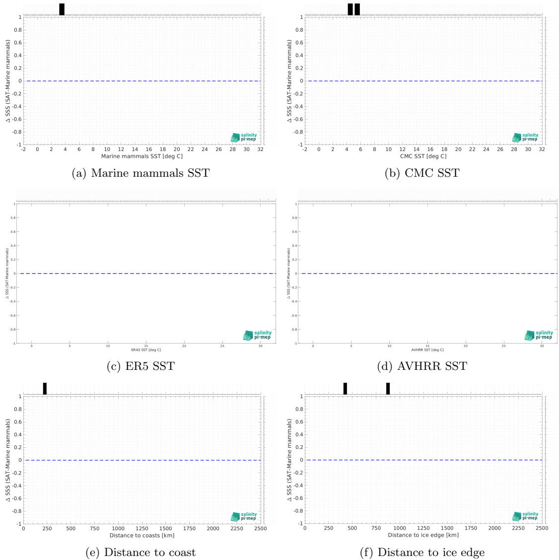
Figure 12: \Delta SSS (Satellite - Marine mammals) sorted as function of Marine mammals SST values (a), CMC SST (b), ERA5 SST (c), AVHRR SST (d), distance to coast (e) and distance to ice edge (f). In all plots the median and Std of \Delta SSS for each bin is indicated by the red curves and black vertical thick bars ( \pm 1 Std). Links to similar figures sorted as function of Sea ice fraction and in situ measurement depth .
