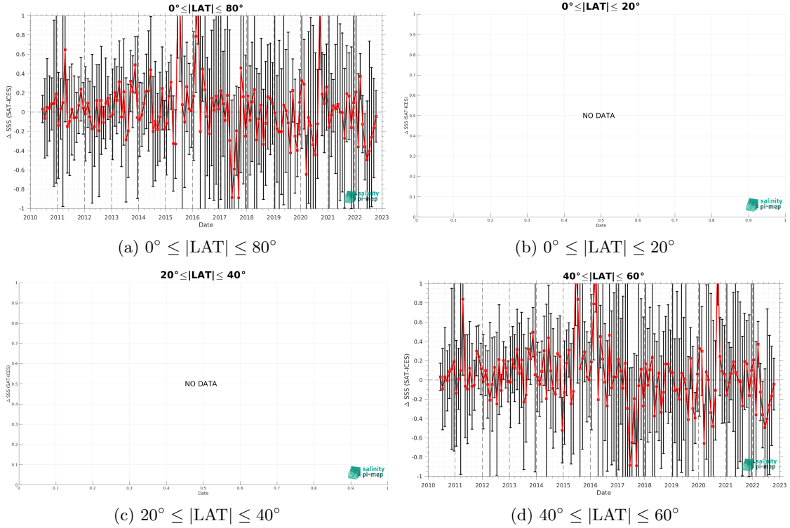
Figure 11: Monthly median (red curves) of \Delta SSS (Satellite - ICES) and \pm 1 Std (black vertical thick bars) as function of time for all the collected Pi-MEP match-up pairs estimated over the North Atlantic Ocean Pi-MEP region and for the full satellite product period are shown for different latitude bands: (a) 80^{\circ}\text{S}-80^{\circ}\text{N} , (b) 20^{\circ}\text{S}-20^{\circ}\text{N} , (c) 40^{\circ}\text{S}-20^{\circ}\text{S} and 20^{\circ}\text{N}-40^{\circ}\text{N} and (d) 60^{\circ}\text{S}-40^{\circ}\text{S} and 40^{\circ}\text{N}-60^{\circ}\text{N} .
