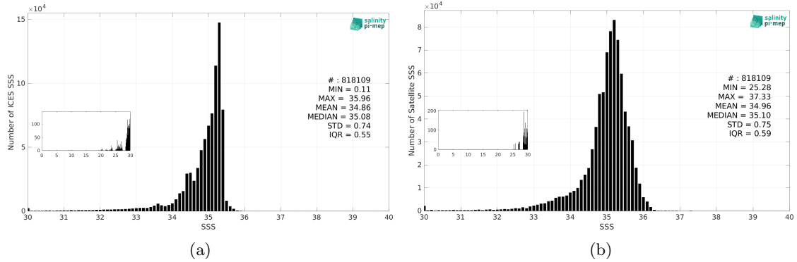
Figure 3: Histograms of SSS from ICES (a) and SMOS SSS L3 Arctic v2 - 9 Days (CATDS-CEC-LOCEAN) (b) considering all match-up pairs per bins of 0.1 over the North Atlantic Ocean Pi-MEP region and for the full satellite product period.
