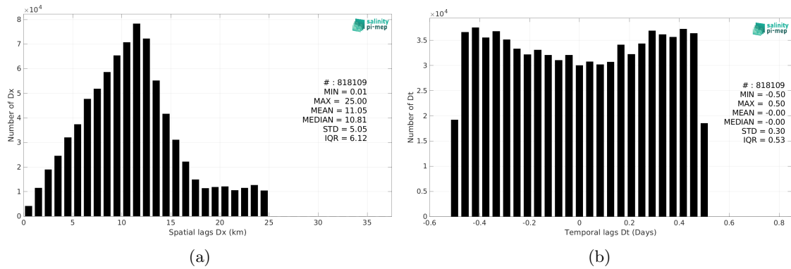
Figure 6: Histograms of the spatial (a) and temporal (b) lags between the location/time of the ICES measurement and the date of the corresponding SMOS SSS L3 Arctic v2 - 9 Days (CATDS-CEC-LOCEAN) SSS pixel.
