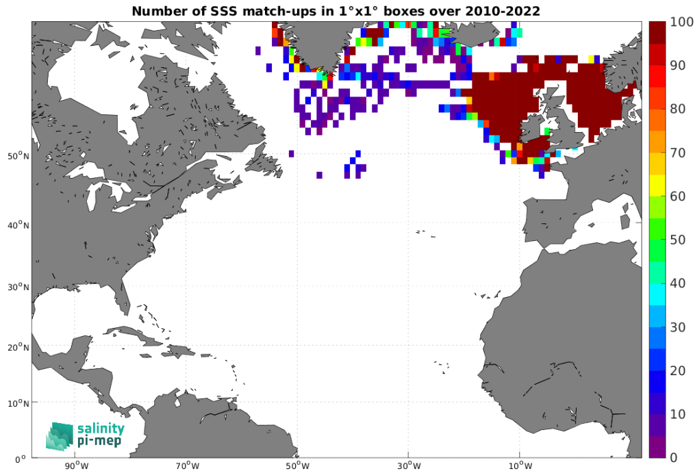
Figure 5: Number of SSS match-ups between ICES SSS and the SMOS SSS L3 Arctic v2 - 9 Days (CATDS-CEC-LOCEAN) SSS product for the North Atlantic Ocean Pi-MEP region over 1^\circ \times 1^\circ boxes and for the full satellite product period.
