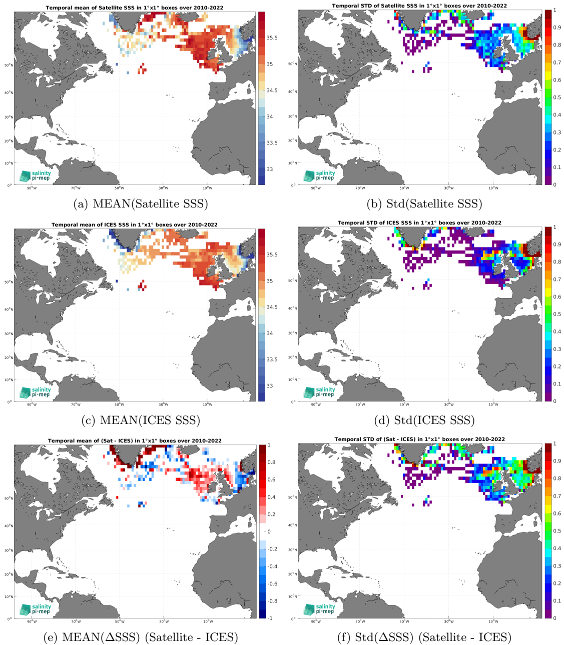
Figure 7: Temporal mean (left) and Std (right) of SSS from SMOS SSS L3 Arctic v2 - 9 Days (CATDS-CEC-LOCEAN) (top), ICES (middle), and of \Delta SSS (Satellite - ICES). Only match-up pairs are used to generate these maps.
