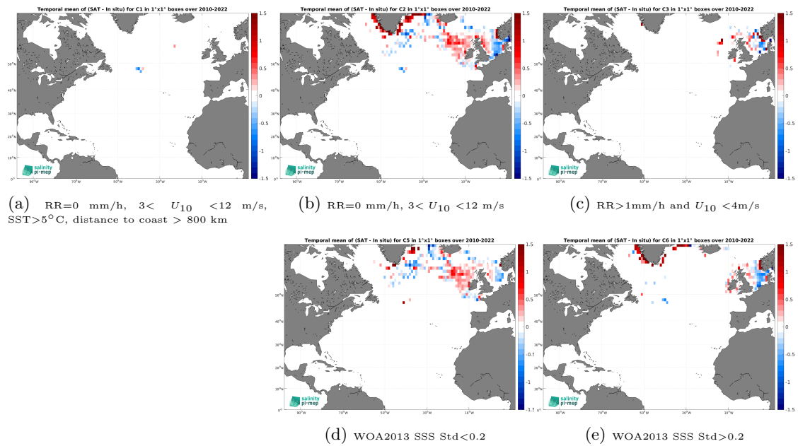
Figure 14: Temporal mean gridded over spatial boxes of size 1^\circ \times 1^\circ of \Delta\text{SSS} (SMOS SSS L3 Arctic v2 - 9 Days (CATDS-CEC-LOCEAN) - ICES) for 5 different subdatasets corresponding to:RR=0 mm/h, 3 < U_{10} < 12 m/s, SST>5°C, distance to coast > 800 km (a), RR=0 mm/h, 3 < U_{10} < 12 m/s (b), RR>1mm/h and U_{10} < 4 m/s (c), WOA2013 SSS Std<0.2 (d), WOA2013 SSS Std>0.2 (e).
