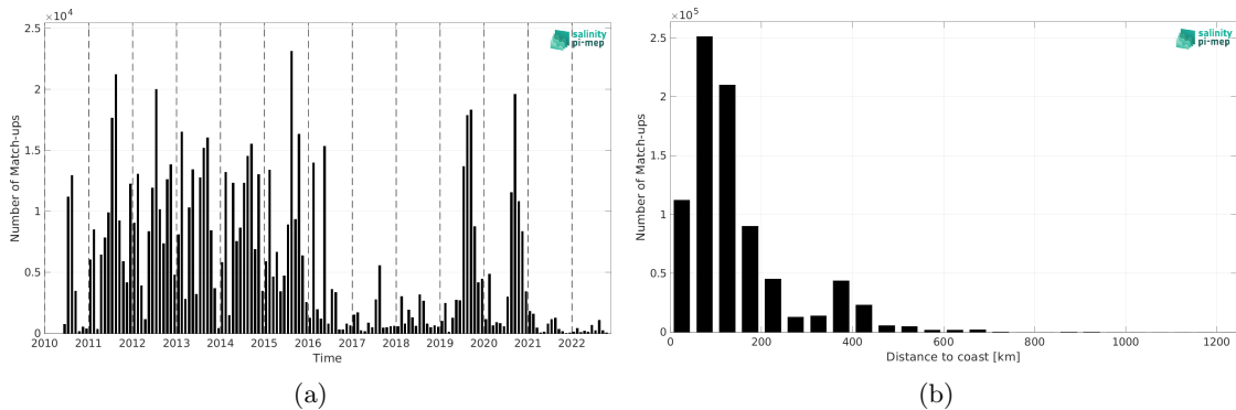
Figure 2: Number of match-ups between ICES and SMOS SSS L3 Arctic v2 - 9 Days (CATDS-CEC-LOCEAN) SSS as a function of time (a) and as function of the distance to coast (b) over the North Atlantic Ocean Pi-MEP region and for the full satellite product period.
