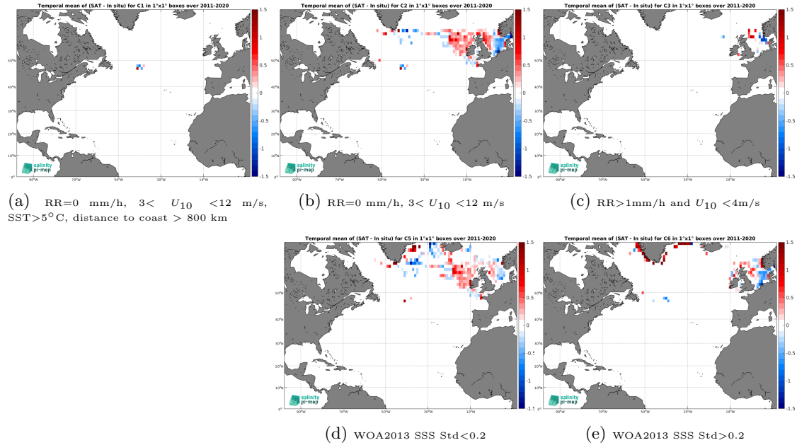
Figure 12: Temporal mean gridded over spatial boxes of size 1^{\circ}\times 1^{\circ} of \Delta\text{SSS} (SMOS SSS L3 Arctic v2 - 9 Days (CATDS-CEC-LOCEAN) - ICES) for 5 different subdatasets corresponding to:RR=0 mm/h, 3 < U_{10} < 12 m/s, SST >5^{\circ}\text{C} , distance to coast > 800 km (a), RR=0 mm/h, 3 < U_{10} < 12 m/s (b), RR >1 mm/h and U_{10} < 4 m/s (c), WOA2013 SSS Std <0.2 (d), WOA2013 SSS Std >0.2 (e).
