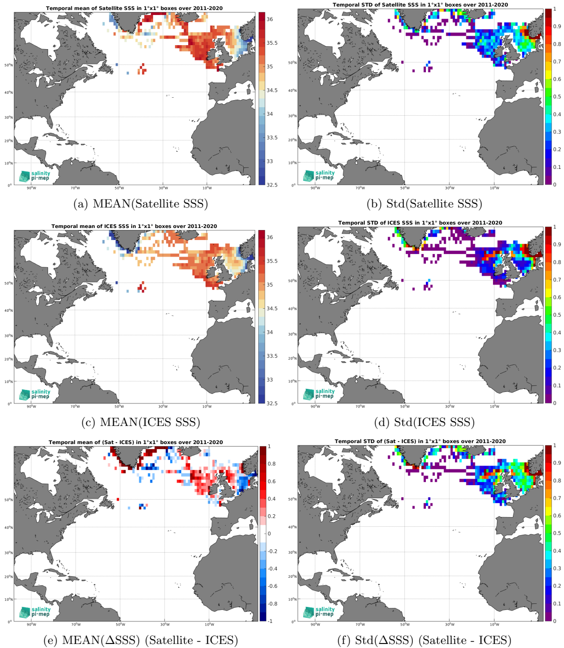
Figure 6: Temporal mean (left) and Std (right) of SSS from SMOS SSS L3 Arctic v2 - 9 Days (CATDS-CEC-LOCEAN) (top), ICES (middle), and of \Delta SSS (Satellite - ICES). Only match-up pairs are used to generate these maps.
