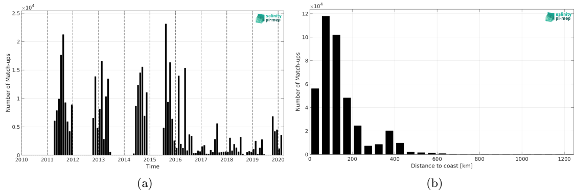
Figure 1: Number of match-ups between ICES and SMOS SSS L3 Arctic v2 - 9 Days (CATDS-CEC-LOCEAN) SSS as a function of time (a) and as function of the distance to coast (b) over the North Atlantic Ocean Pi-MEP region and for the full satellite product period.
