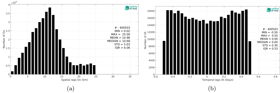
Figure 5: Histograms of the spatial (a) and temporal (b) lags between the location/time of the ICES measurement and the date of the corresponding SMOS SSS L3 Arctic v2 - 9 Days (CATDS-CEC-LOCEAN) SSS pixel.
