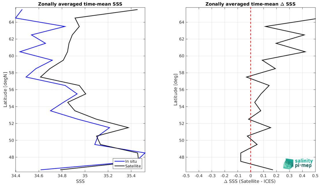
Figure 8: Left panel: Zonal mean SSS from SMOS SSS L3 Arctic v2 - 9 Days (CATDS-CEC-LOCEAN) satellite product (black) and from ICES (blue). Right panel: Zonal mean of \Delta SSS (Satellite - ICES) for all the collected Pi-MEP match-up pairs estimated over the full satellite product period.
