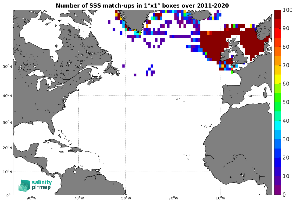
Figure 4: Number of SSS match-ups between ICES SSS and the SMOS SSS L3 Arctic v2 - 9 Days (CATDS-CEC-LOCEAN) SSS product for the North Atlantic Ocean Pi-MEP region over 1^\circ \times 1^\circ boxes and for the full satellite product period.
