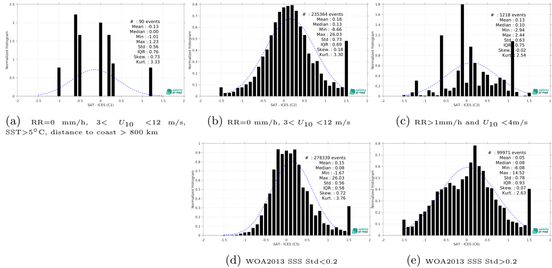
Figure 13: Normalized histogram of \Delta SSS (SMOS SSS L3 Arctic v2 - 9 Days (CATDS-CEC-LOCEAN) - ICES) for 5 different subdatasets corresponding to: RR=0 mm/h, 3 < U_{10} < 12 m/s, SST > 5°C, distance to coast > 800 km (a), RR=0 mm/h, 3 < U_{10} < 12 m/s (b), RR > 1mm/h and U_{10} < 4 m/s (c), WOA2013 SSS Std < 0.2 (d), WOA2013 SSS Std > 0.2 (e).
