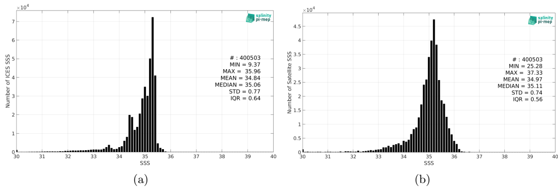
Figure 2: Histograms of SSS from ICES (a) and SMOS SSS L3 Arctic v2 - 9 Days (CATDS-CEC-LOCEAN) (b) considering all match-up pairs per bins of 0.1 over the North Atlantic Ocean Pi-MEP region and for the full satellite product period.
