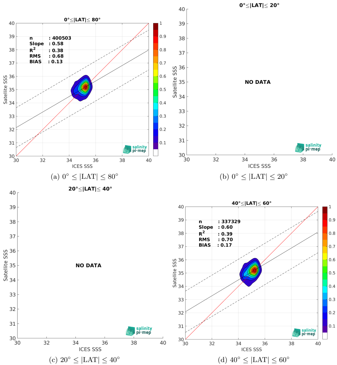
Figure 9: Contour maps of the concentration of SMOS SSS L3 Arctic v2 - 9 Days (CATDS-CEC-LOCEAN) SSS (y-axis) versus ICES SSS (x-axis) at match-up pairs for different latitude bands. For each plot, the red line shows x=y . The black thin and dashed lines indicate a linear fit through the data cloud and the \pm 95\% confidence levels, respectively. The number match-up pairs n , the slope and R^2 coefficient of the linear fit, the root mean square (RMS) and the mean bias between satellite and in situ data are indicated for each latitude band in each plots.
