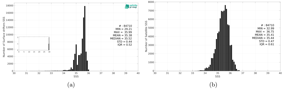
Figure 3: Histograms of SSS from Surface drifters (a) and SMOS SSS L3 Arctic v2 - 9 Days (CATDS-CEC-LOCEAN) (b) considering all match-up pairs per bins of 0.1 over the North Atlantic Ocean Pi-MEP region and for the full satellite product period.
