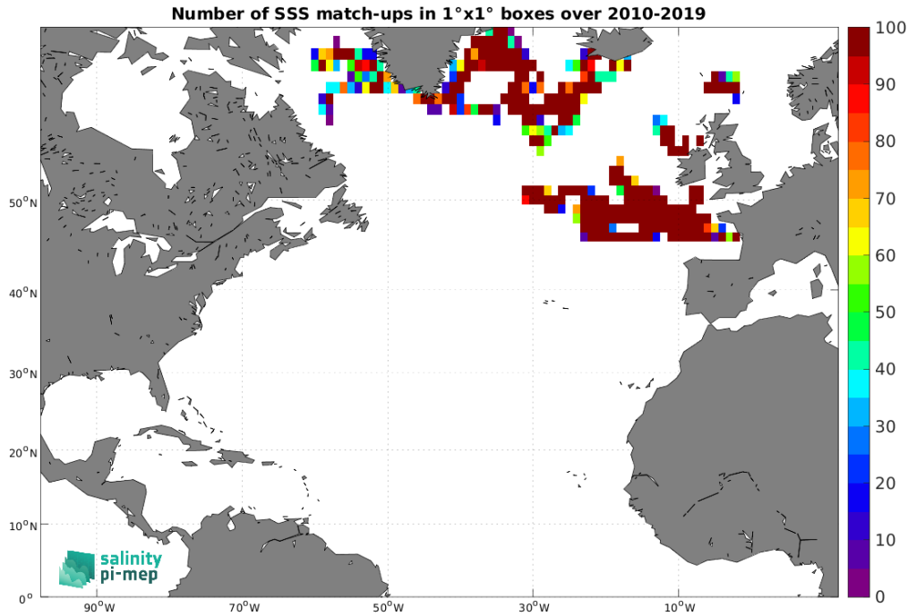
Figure 4: Number of SSS match-ups between Surface drifters SSS and the SMOS SSS L3 Arctic v2 - 9 Days (CATDS-CEC-LOCEAN) SSS product for the North Atlantic Ocean Pi-MEP region over 1^\circ \times 1^\circ boxes and for the full satellite product period.
