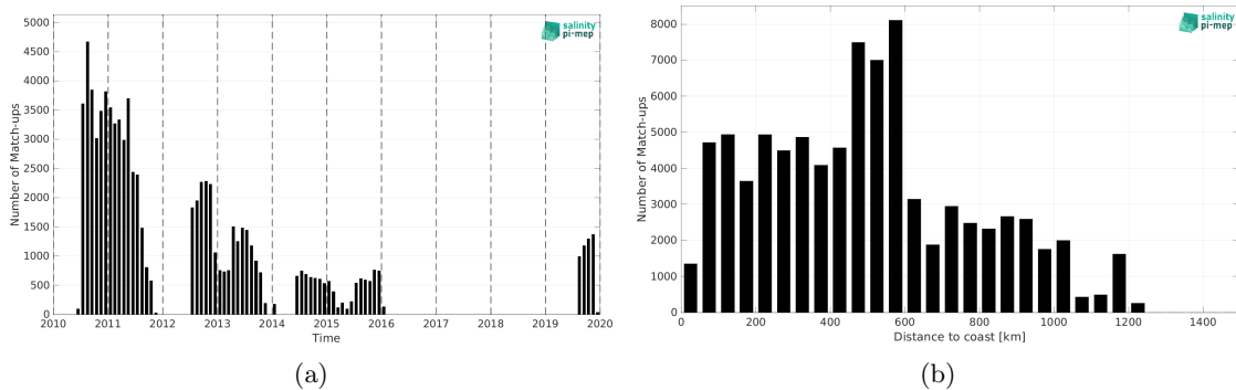
Figure 2: Number of match-ups between Surface drifters and SMOS SSS L3 Arctic v2 - 9 Days (CATDS-CEC-LOCEAN) SSS as a function of time (a) and as function of the distance to coast (b) over the North Atlantic Ocean Pi-MEP region and for the full satellite product period.
