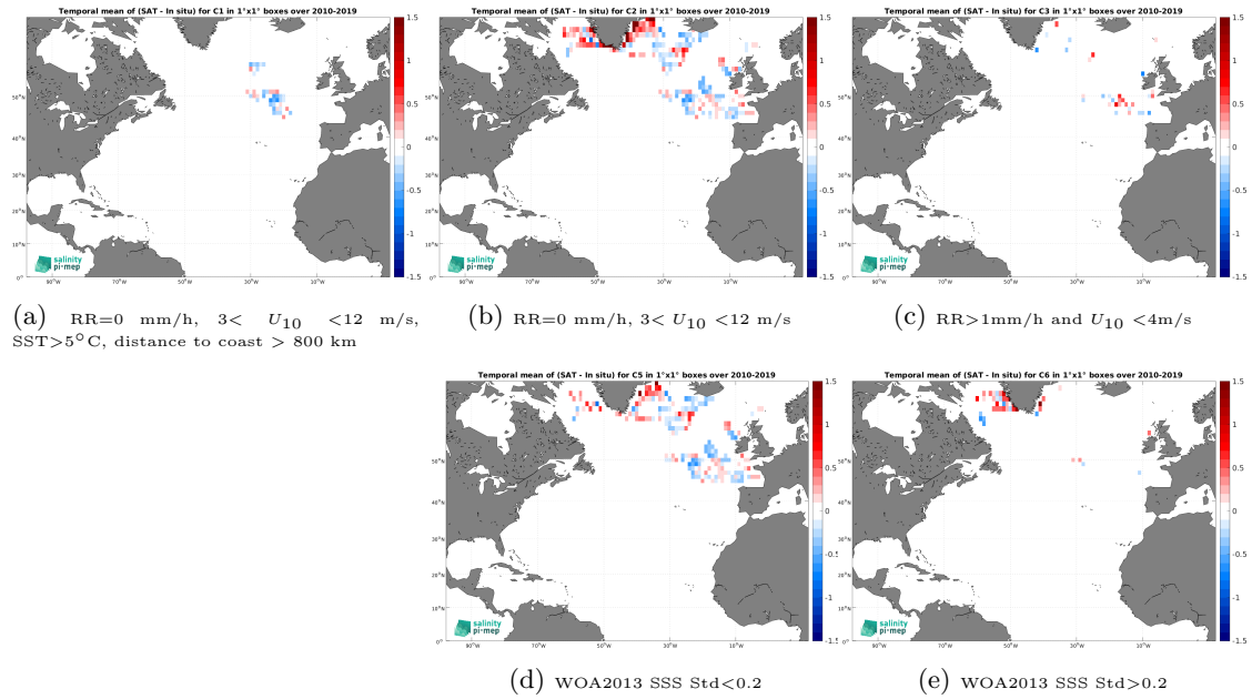
Figure 13: Temporal mean gridded over spatial boxes of size 1^\circ \times 1^\circ of \Delta\text{SSS} (SMOS SSS L3 Arctic v2 - 9 Days (CATDS-CEC-LOCEAN) - Surface drifters) for 5 different subdatasets corresponding to:RR=0 mm/h, 3 < U_{10} < 12 m/s, SST >5^\circ\text{C} , distance to coast > 800 km (a), RR=0 mm/h, 3 < U_{10} < 12 m/s (b), RR >1 mm/h and U_{10} < 4 m/s (c), WOA2013 SSS Std <0.2 (d), WOA2013 SSS Std >0.2 (e).
