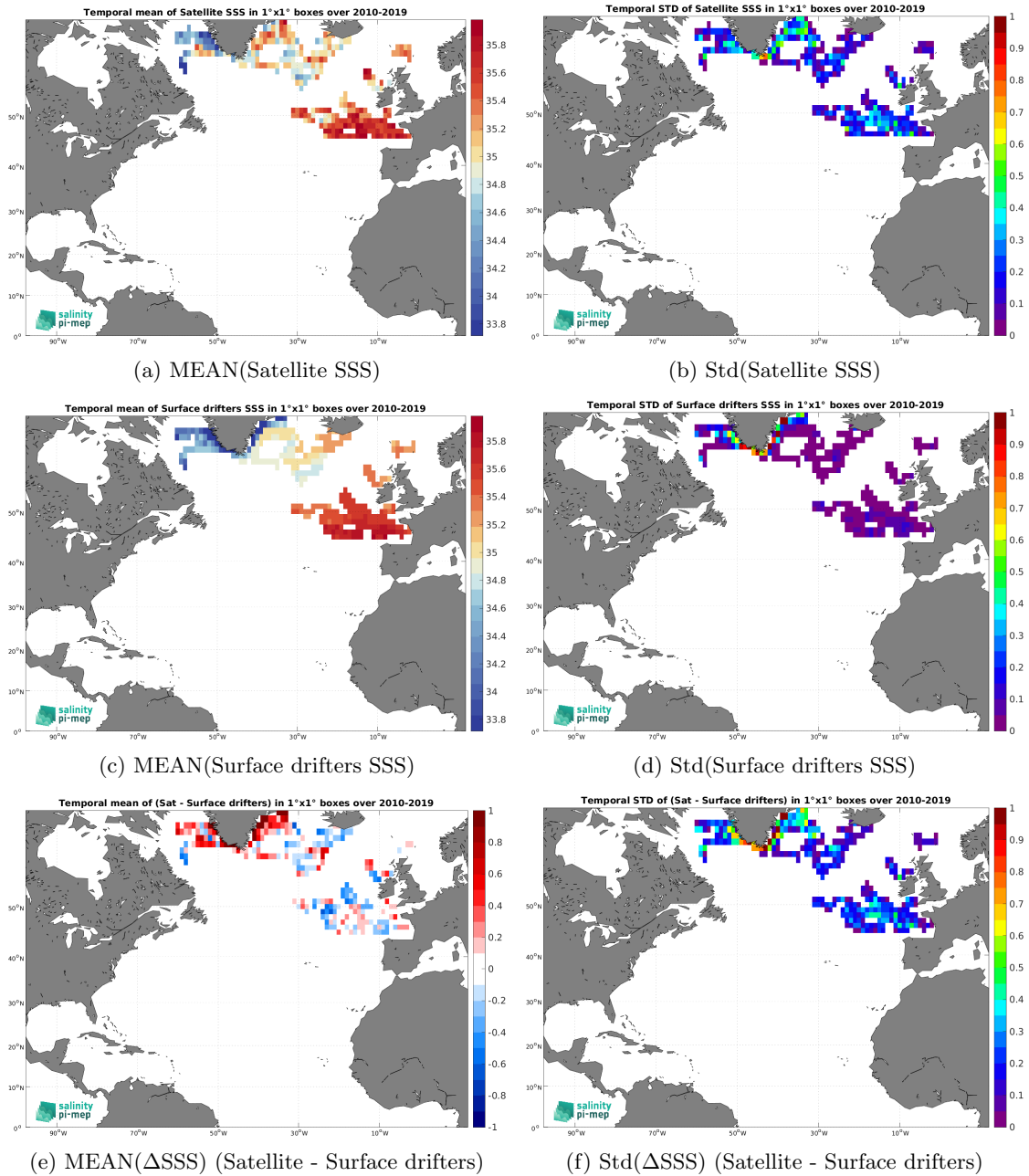
Figure 6: Temporal mean (left) and Std (right) of SSS from SMOS SSS L3 Arctic v2 - 9 Days (CATDS-CEC-LOCEAN) (top), Surface drifters (middle), and of \Delta SSS (Satellite - Surface drifters). Only match-up pairs are used to generate these maps.
