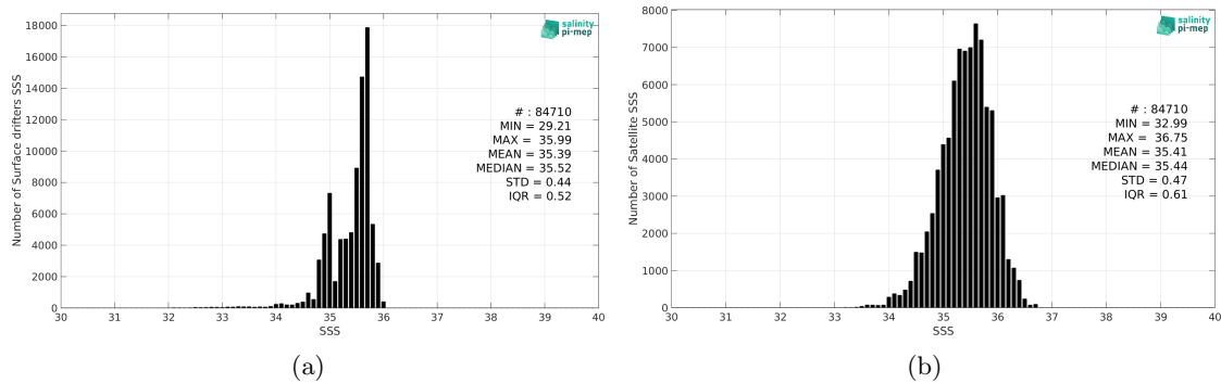
Figure 2: Histograms of SSS from Surface drifters (a) and SMOS SSS L3 Arctic v2 - 9 Days (CATDS-CEC-LOCEAN) (b) considering all match-up pairs per bins of 0.1 over the North Atlantic Ocean Pi-MEP region and for the full satellite product period.
