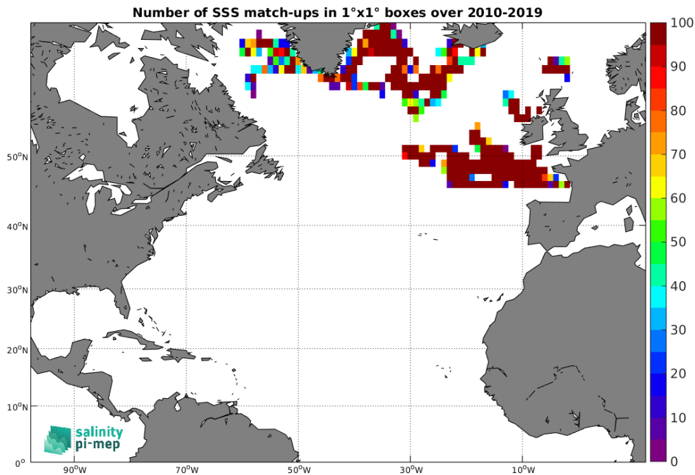
Figure 3: Number of SSS match-ups between Surface drifters SSS and the SMOS SSS L3 Arctic v2 - 9 Days (CATDS-CEC-LOCEAN) SSS product for the North Atlantic Ocean Pi-MEP region over 1^\circ \times 1^\circ boxes and for the full satellite product period.
