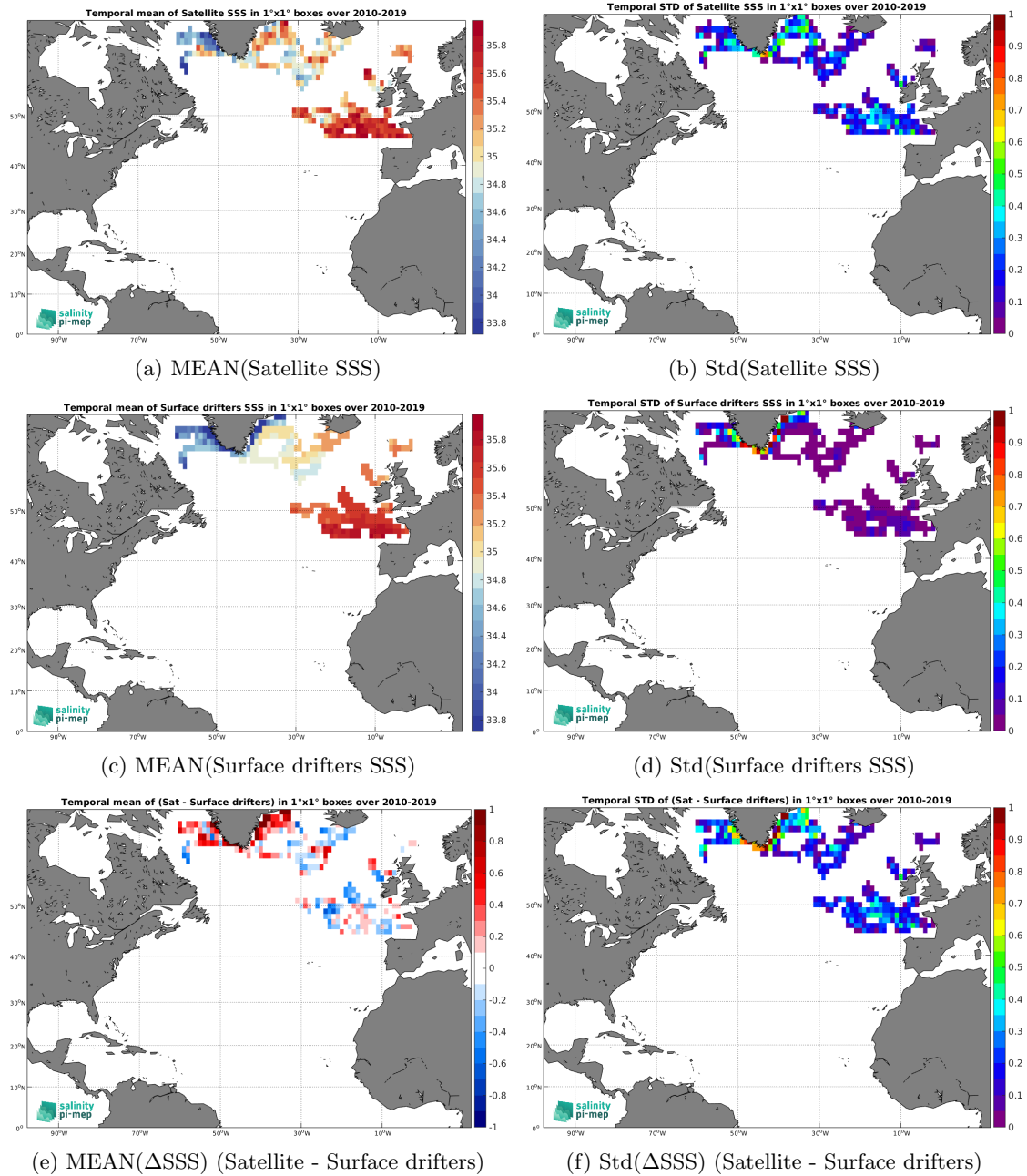
Figure 5: Temporal mean (left) and Std (right) of SSS from SMOS SSS L3 Arctic v2 - 9 Days (CATDS-CEC-LOCEAN) (top), Surface drifters (middle), and of \Delta SSS (Satellite - Surface drifters). Only match-up pairs are used to generate these maps.
