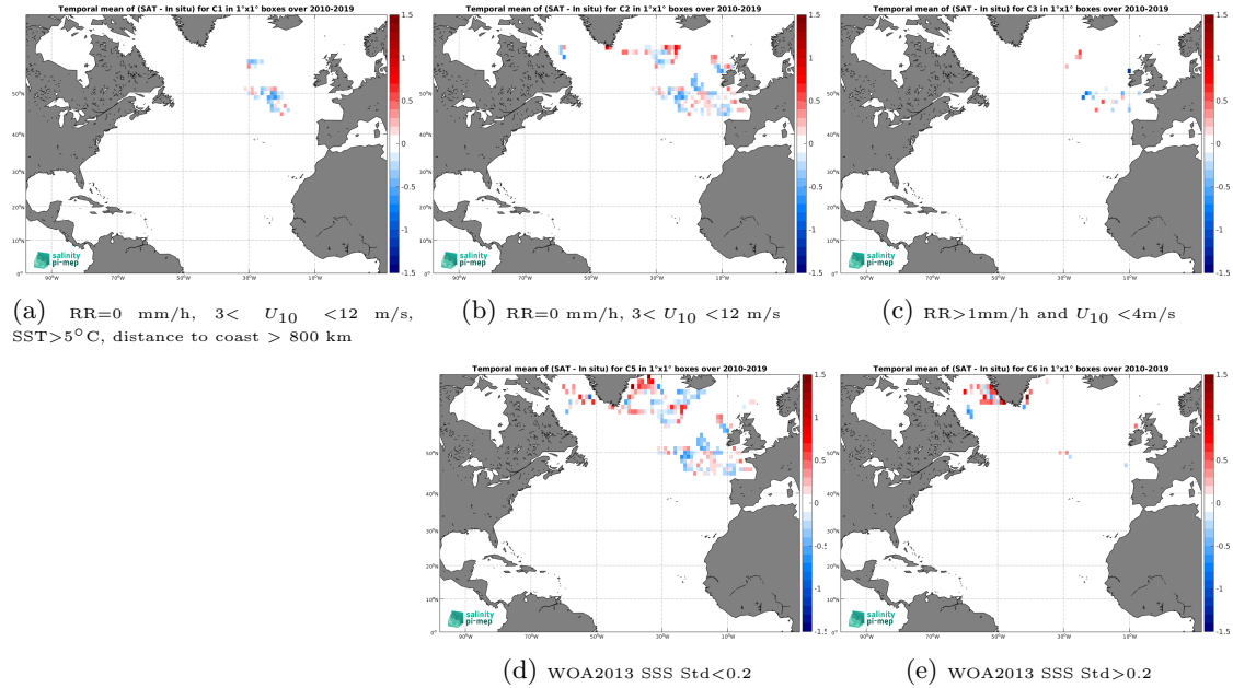
Figure 11: Temporal mean gridded over spatial boxes of size 1^{\circ}\times 1^{\circ} of \Delta\text{SSS} (SMOS SSS L3 Arctic v2 - 9 Days (CATDS-CEC-LOCEAN) - Surface drifters) for 5 different subdatasets corresponding to:RR=0 mm/h, 3 < U_{10} < 12 m/s, SST >5^{\circ}\text{C} , distance to coast > 800 km (a), RR=0 mm/h, 3 < U_{10} < 12 m/s (b), RR >1 mm/h and U_{10} < 4 m/s (c), WOA2013 SSS Std <0.2 (d), WOA2013 SSS Std >0.2 (e).
