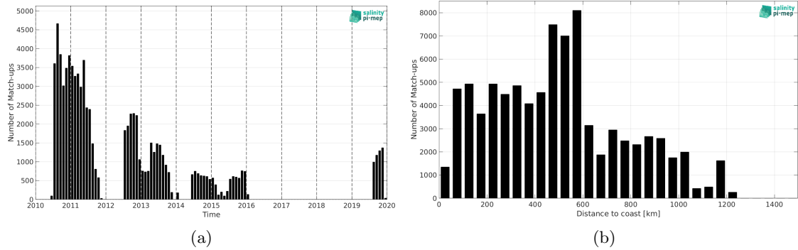
Figure 1: Number of match-ups between Surface drifters and SMOS SSS L3 Arctic v2 - 9 Days (CATDS-CEC-LOCEAN) SSS as a function of time (a) and as function of the distance to coast (b) over the North Atlantic Ocean Pi-MEP region and for the full satellite product period.
