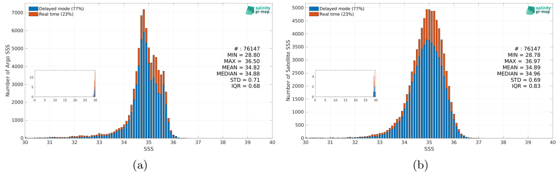
Figure 3: Histograms of SSS from Argo (a) and SMOS SSS L3 Arctic v2 - 9 Days (CATDS-CEC-LOCEAN) (b) considering all match-up pairs per bins of 0.1 over the North Atlantic Ocean Pi-MEP region and for the full satellite product period.
