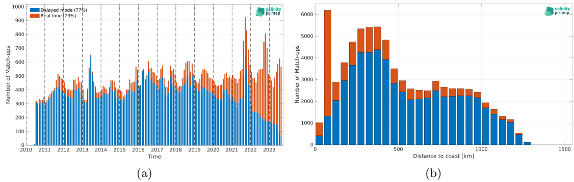
Figure 2: Number of match-ups between Argo and SMOS SSS L3 Arctic v2 - 9 Days (CATDS-CEC-LOCEAN) SSS as a function of time (a) and as function of the distance to coast (b) over the North Atlantic Ocean Pi-MEP region and for the full satellite product period.
