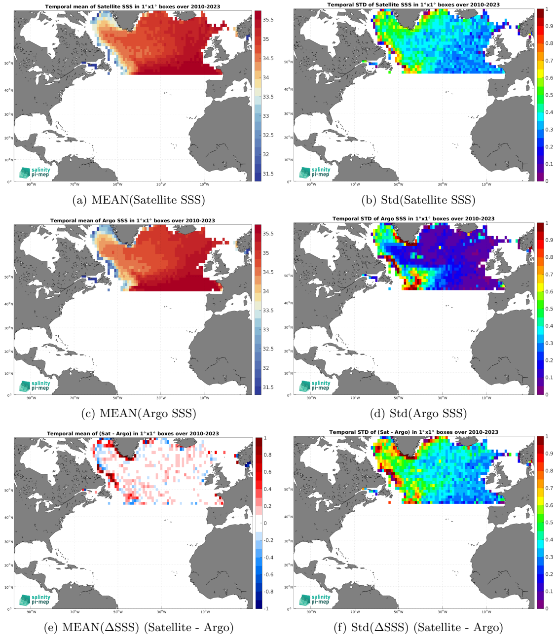
Figure 7: Temporal mean (left) and Std (right) of SSS from SMOS SSS L3 Arctic v2 - 9 Days (CATDS-CEC-LOCEAN) (top), Argo (middle), and of \Delta SSS (Satellite - Argo). Only match-up pairs are used to generate these maps.
