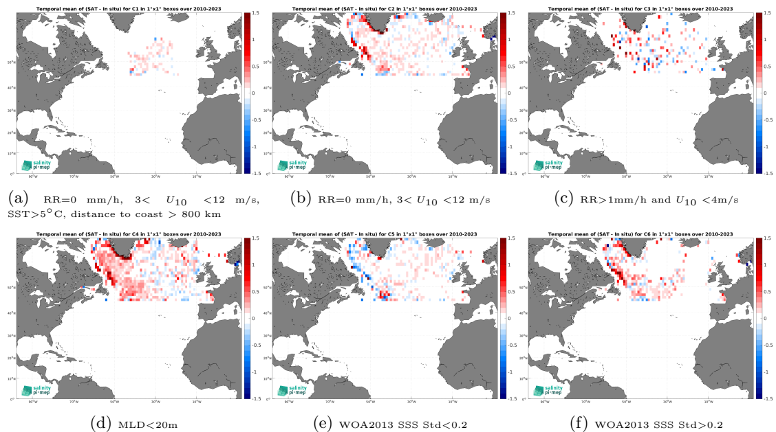
Figure 14: Temporal mean gridded over spatial boxes of size 1^\circ \times 1^\circ of \Delta SSS (SMOS SSS L3 Arctic v2 - 9 Days (CATDS-CEC-LOCEAN) - Argo) for 6 different subdatasets corresponding to:RR=0 mm/h, 3 < U_{10} < 12 m/s, SST > 5^\circ\text{C} , distance to coast > 800 km (a), RR=0 mm/h, 3 < U_{10} < 12 m/s (b), RR > 1 mm/h and U_{10} < 4 m/s (c),MLD < 20 m (d),WOA2013 SSS Std < 0.2 (e),WOA2013 SSS Std > 0.2 (f).
