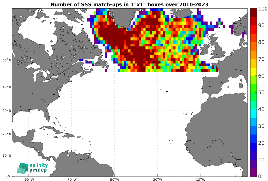
Figure 5: Number of SSS match-ups between Argo SSS and the SMOS SSS L3 Arctic v2 - 9 Days (CATDS-CEC-LOCEAN) SSS product for the North Atlantic Ocean Pi-MEP region over 1^\circ \times 1^\circ boxes and for the full satellite product period.
