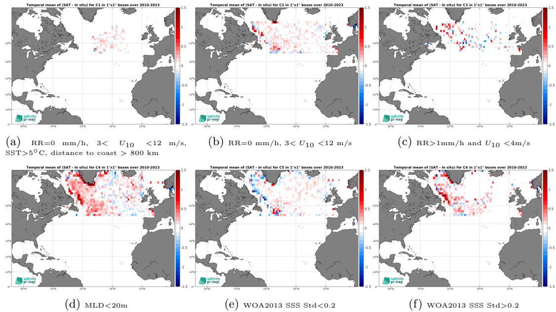
Figure 12: Temporal mean gridded over spatial boxes of size 1^{\circ}\times 1^{\circ} of \Delta\text{SSS} (SMOS SSS L3 Arctic v2 - 9 Days (CATDS-CEC-LOCEAN) - Argo) for 6 different subdatasets corresponding to:RR=0 mm/h, 3 < U_{10} < 12 m/s, SST >5^{\circ}\text{C} , distance to coast > 800 km (a), RR=0 mm/h, 3 < U_{10} < 12 m/s (b), RR >1\text{mm/h} and U_{10} < 4\text{m/s} (c),MLD <20\text{m} (d),WOA2013 SSS Std <0.2 (e),WOA2013 SSS Std >0.2 (f).
