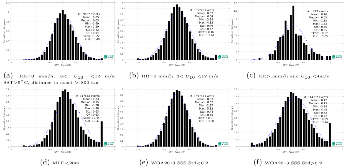
Figure 13: Normalized histogram of \Delta SSS (SMOS SSS L3 Arctic v2 - 9 Days (CATDS-CEC-LOCEAN) - Argo) for 6 different subdatasets corresponding to: RR=0 mm/h, 3 < U_{10} < 12 m/s, SST>5°C, distance to coast > 800 km (a), RR=0 mm/h, 3 < U_{10} < 12 m/s (b), RR>1mm/h and U_{10} < 4 m/s (c), MLD<20m (d), WOA2013 SSS Std<0.2 (e), WOA2013 SSS Std>0.2 (f).
