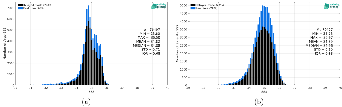
Figure 2: Histograms of SSS from Argo (a) and SMOS SSS L3 Arctic v2 - 9 Days (CATDS-CEC-LOCEAN) (b) considering all match-up pairs per bins of 0.1 over the North Atlantic Ocean Pi-MEP region and for the full satellite product period.
