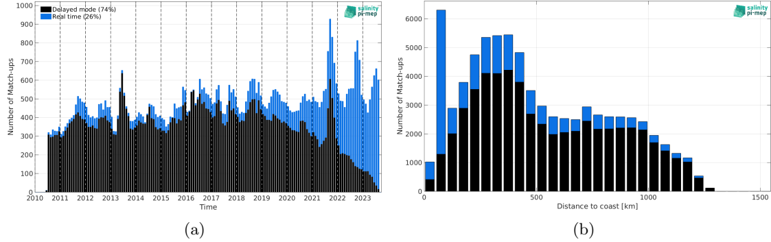
Figure 1: Number of match-ups between Argo and SMOS SSS L3 Arctic v2 - 9 Days (CATDS-CEC-LOCEAN) SSS as a function of time (a) and as function of the distance to coast (b) over the North Atlantic Ocean Pi-MEP region and for the full satellite product period.
