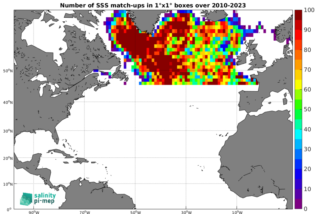
Figure 4: Number of SSS match-ups between Argo SSS and the SMOS SSS L3 Arctic v2 - 9 Days (CATDS-CEC-LOCEAN) SSS product for the North Atlantic Ocean Pi-MEP region over 1^\circ \times 1^\circ boxes and for the full satellite product period.
