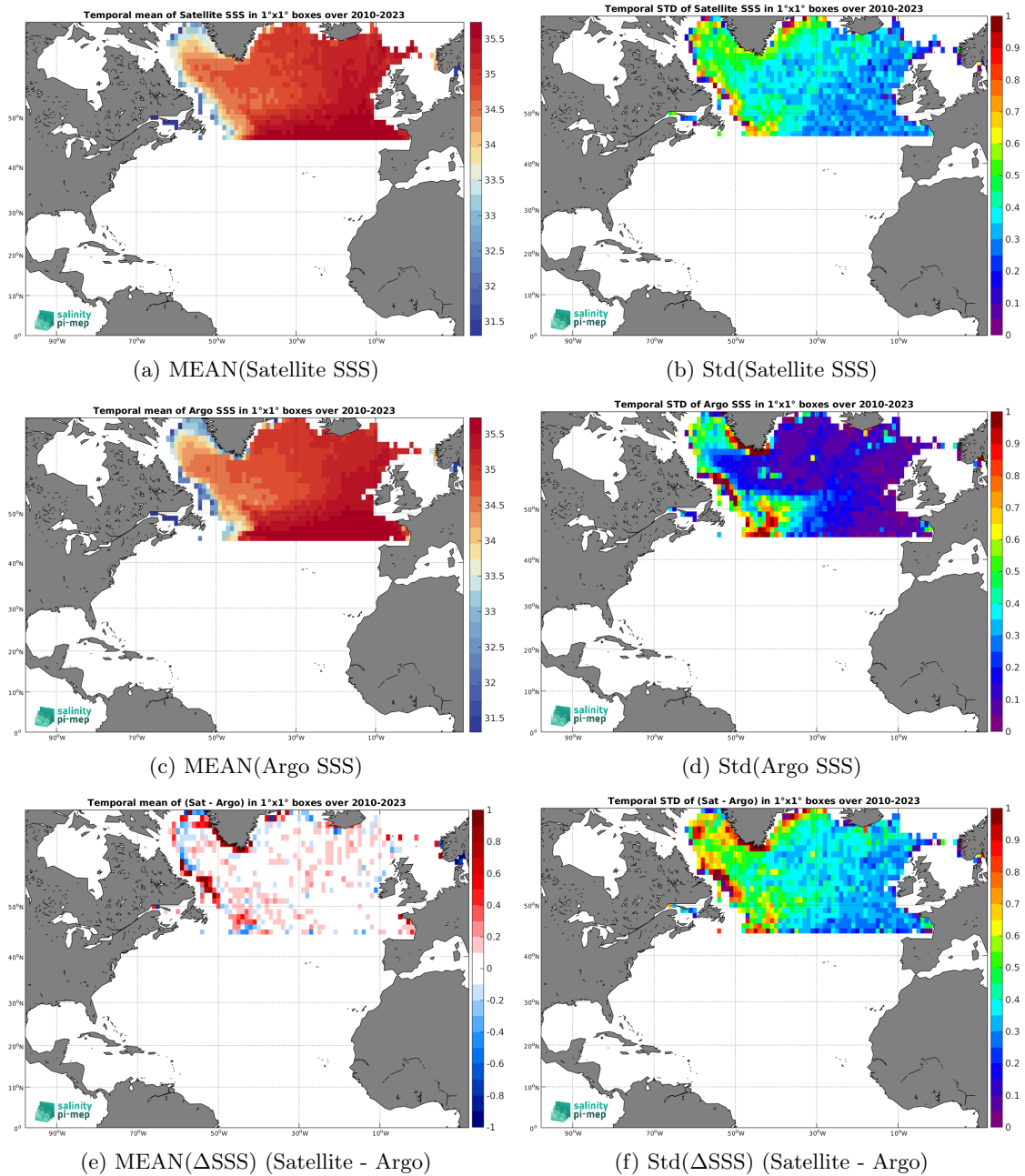
Figure 6: Temporal mean (left) and Std (right) of SSS from SMOS SSS L3 Arctic v2 - 9 Days (CATDS-CEC-LOCEAN) (top), Argo (middle), and of \Delta SSS (Satellite - Argo). Only match-up pairs are used to generate these maps.
