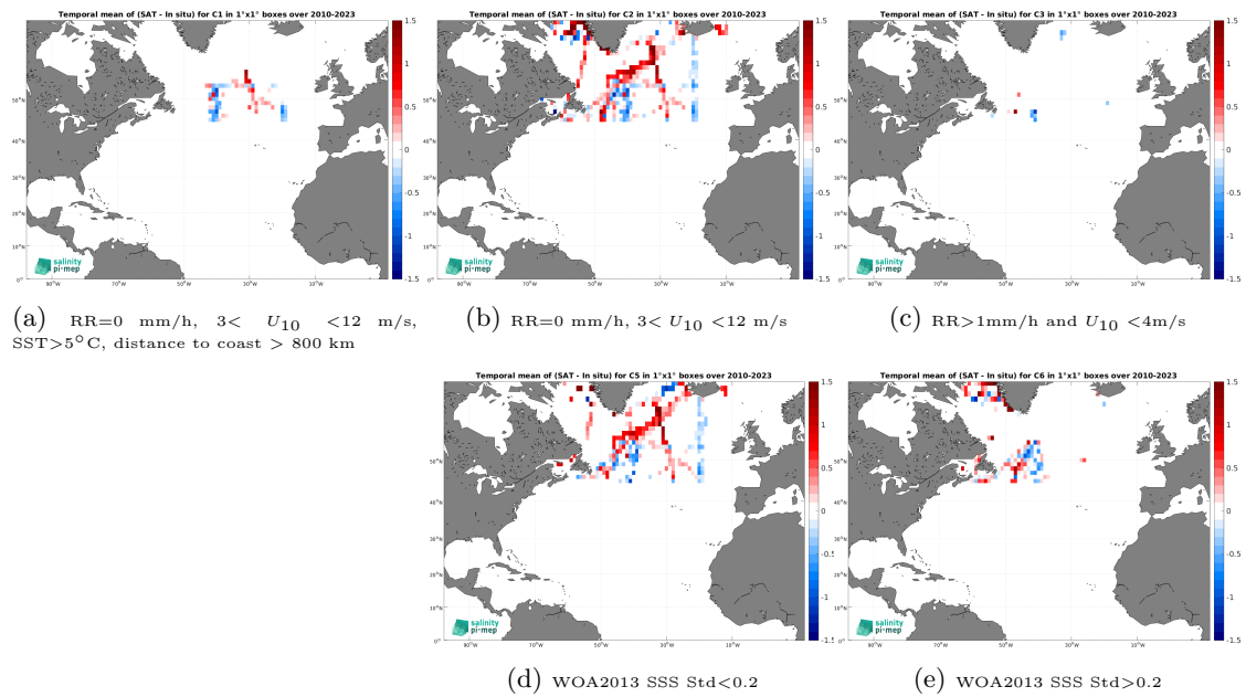
Figure 14: Temporal mean gridded over spatial boxes of size 1^\circ \times 1^\circ of \Delta\text{SSS} (SMOS SSS L3 Arctic v2 - 18 Days (CATDS-CEC-LOCEAN) - TSG (SAMOS)) for 5 different subdatasets corresponding to:RR=0 mm/h, 3 < U_{10} < 12 m/s, SST >5^\circ\text{C} , distance to coast > 800 km (a), RR=0 mm/h, 3 < U_{10} < 12 m/s (b), RR >1 mm/h and U_{10} < 4 m/s (c), WOA2013 SSS Std <0.2 (d), WOA2013 SSS Std >0.2 (e).
