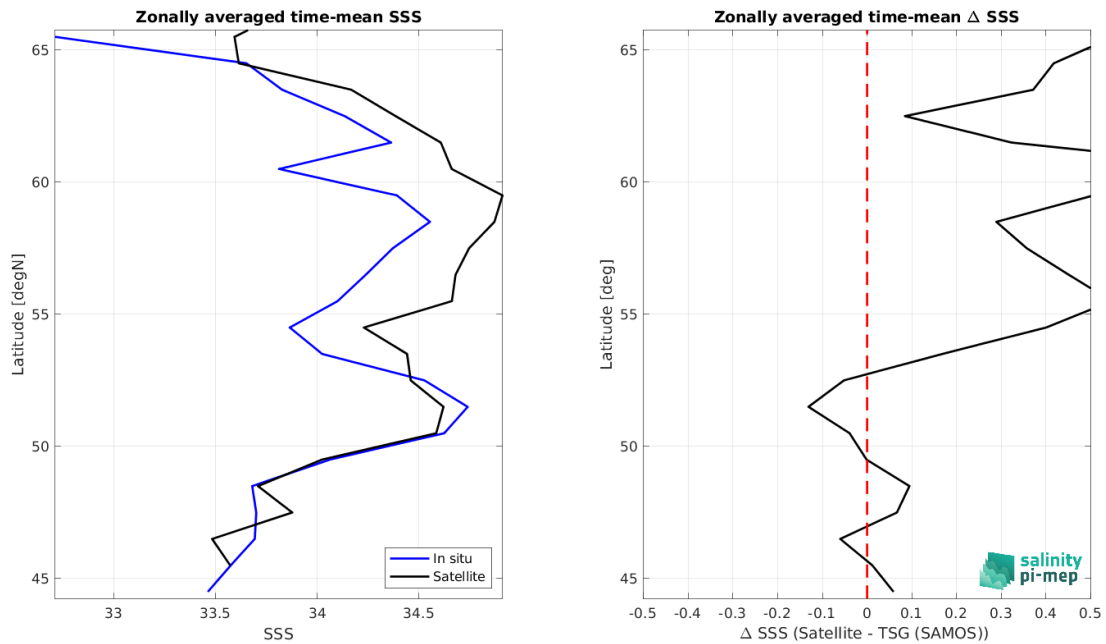
Figure 9: Left panel: Zonal mean SSS from SMOS SSS L3 Arctic v2 - 18 Days (CATDS-CEC-LOCEAN) satellite product (black) and from TSG (SAMOS) (blue). Right panel: Zonal mean of \Delta SSS (Satellite - TSG (SAMOS)) for all the collected Pi-MEP match-up pairs estimated over the full satellite product period.
