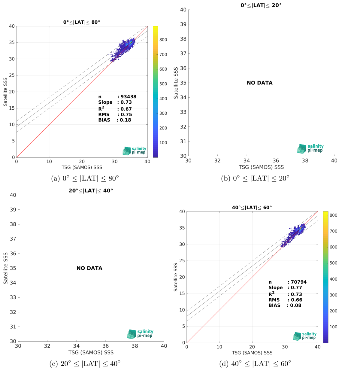
Figure 10: Contour maps of the concentration of SMOS SSS L3 Arctic v2 - 18 Days (CATDS-CEC-LOCEAN) SSS (y-axis) versus TSG (SAMOS) SSS (x-axis) at match-up pairs for different latitude bands. For each plot, the red line shows x=y . The black thin and dashed lines indicate a linear fit through the data cloud and the \pm 95\% confidence levels, respectively. The number match-up pairs n , the slope and R^2 coefficient of the linear fit, the root mean square (RMS) and the mean bias between satellite and in situ data are indicated for each latitude band in each plots.
