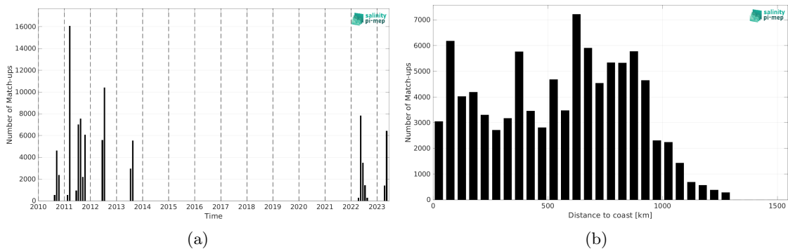
Figure 2: Number of match-ups between TSG (SAMOS) and SMOS SSS L3 Arctic v2 - 18 Days (CATDS-CEC-LOCEAN) SSS as a function of time (a) and as function of the distance to coast (b) over the North Atlantic Ocean Pi-MEP region and for the full satellite product period.
