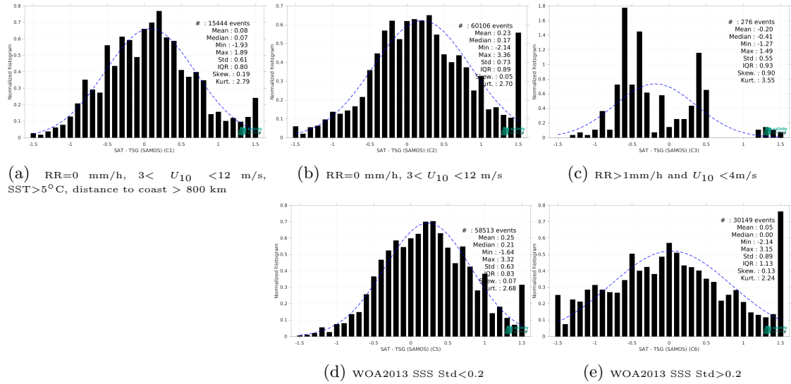
Figure 15: Normalized histogram of \Delta SSS (SMOS SSS L3 Arctic v2 - 18 Days (CATDS-CEC-LOCEAN) - TSG (SAMOS)) for 5 different subdatasets corresponding to: RR=0 mm/h, 3 < U_{10} < 12 m/s, SST > 5°C, distance to coast > 800 km (a), RR=0 mm/h, 3 < U_{10} < 12 m/s (b), RR > 1mm/h and U_{10} < 4 m/s (c), WOA2013 SSS Std < 0.2 (d), WOA2013 SSS Std > 0.2 (e).
