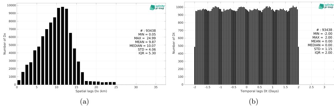
Figure 6: Histograms of the spatial (a) and temporal (b) lags between the location/time of the TSG (SAMOS) measurement and the date of the corresponding SMOS SSS L3 Arctic v2 - 18 Days (CATDS-CEC-LOCEAN) SSS pixel.
