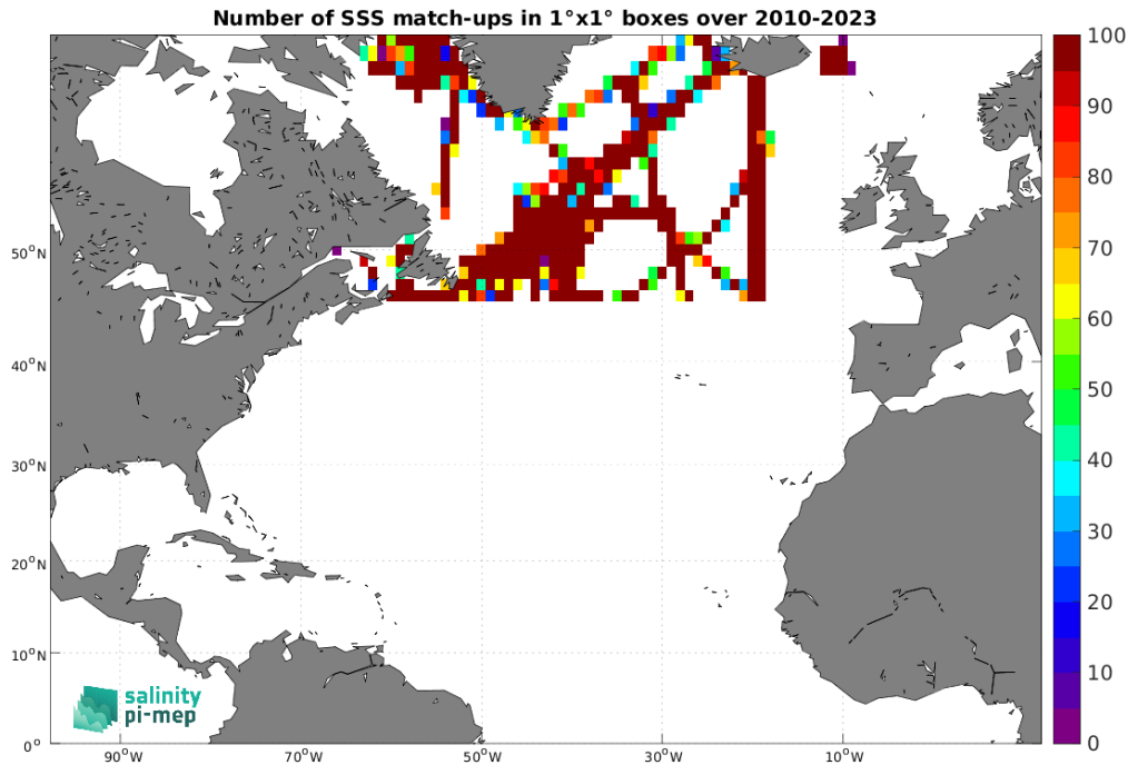
Figure 5: Number of SSS match-ups between TSG (SAMOS) SSS and the SMOS SSS L3 Arctic v2 - 18 Days (CATDS-CEC-LOCEAN) SSS product for the North Atlantic Ocean Pi-MEP region over 1^\circ \times 1^\circ boxes and for the full satellite product period.
