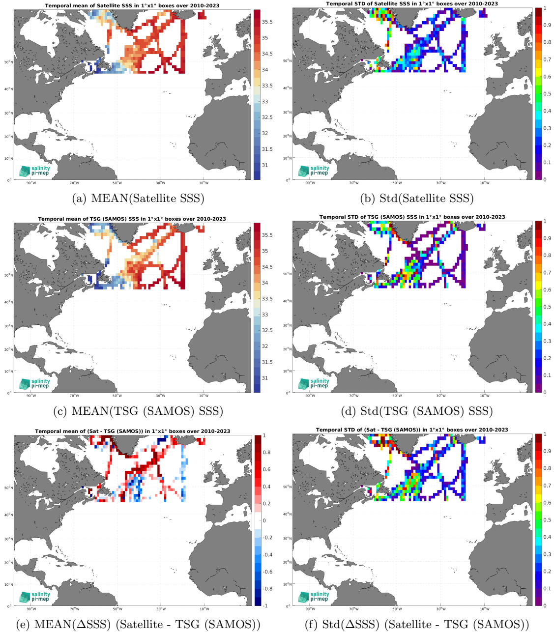
Figure 7: Temporal mean (left) and Std (right) of SSS from SMOS SSS L3 Arctic v2 - 18 Days (CATDS-CEC-LOCEAN) (top), TSG (SAMOS) (middle), and of \Delta SSS (Satellite - TSG (SAMOS)). Only match-up pairs are used to generate these maps.
