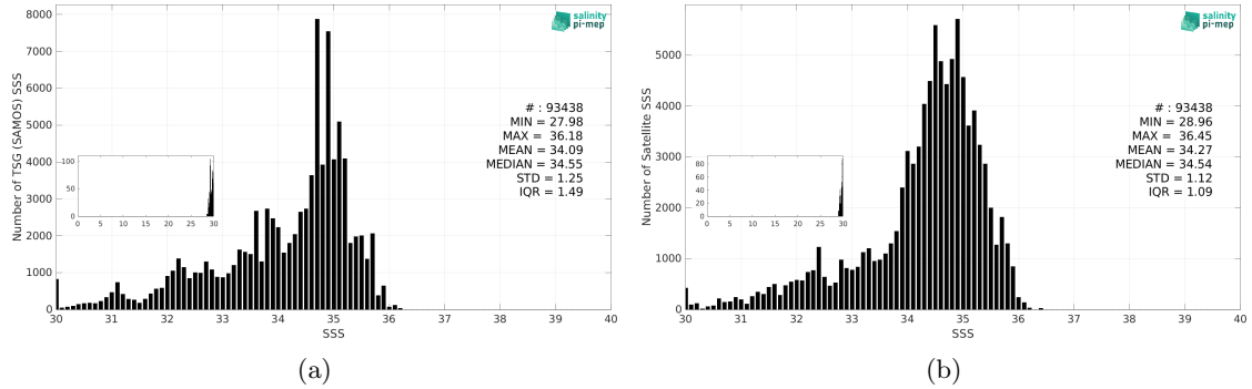
Figure 3: Histograms of SSS from TSG (SAMOS) (a) and SMOS SSS L3 Arctic v2 - 18 Days (CATDS-CEC-LOCEAN) (b) considering all match-up pairs per bins of 0.1 over the North Atlantic Ocean Pi-MEP region and for the full satellite product period.
