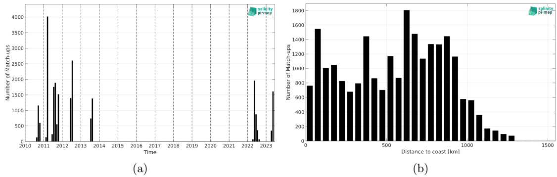
Figure 1: Number of match-ups between TSG (SAMOS) and SMOS SSS L3 Arctic v2 - 18 Days (CATDS-CEC-LOCEAN) SSS as a function of time (a) and as function of the distance to coast (b) over the North Atlantic Ocean Pi-MEP region and for the full satellite product period.
