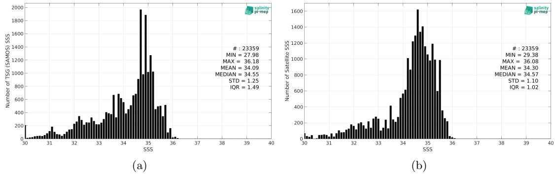
Figure 2: Histograms of SSS from TSG (SAMOS) (a) and SMOS SSS L3 Arctic v2 - 18 Days (CATDS-CEC-LOCEAN) (b) considering all match-up pairs per bins of 0.1 over the North Atlantic Ocean Pi-MEP region and for the full satellite product period.
