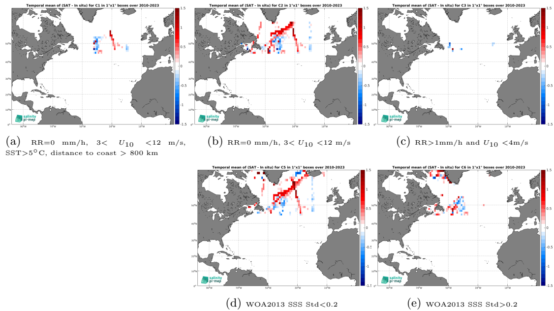
Figure 12: Temporal mean gridded over spatial boxes of size 1^{\circ}\times 1^{\circ} of \Delta\text{SSS} (SMOS SSS L3 Arctic v2 - 18 Days (CATDS-CEC-LOCEAN) - TSG (SAMOS)) for 5 different subdatasets corresponding to: RR=0 mm/h, 3 < U_{10} < 12 m/s, SST > 5^{\circ}\text{C} , distance to coast > 800 km (a), RR=0 mm/h, 3 < U_{10} < 12 m/s (b), RR > 1 mm/h and U_{10} < 4 m/s (c), WOA2013 SSS Std < 0.2 (d), WOA2013 SSS Std > 0.2 (e).
