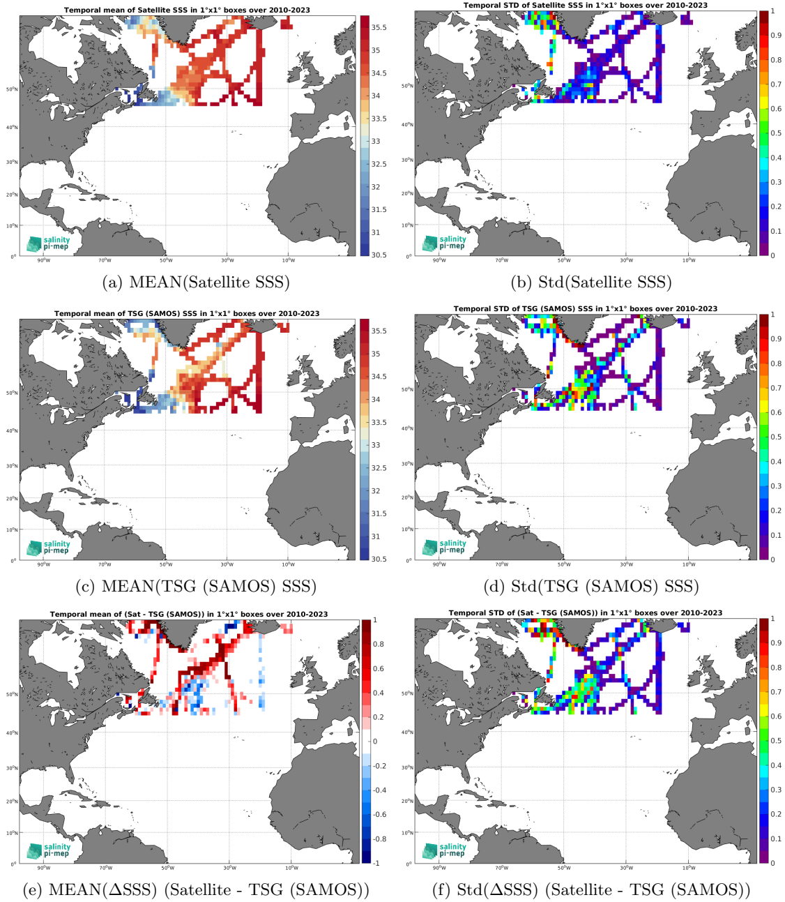
Figure 6: Temporal mean (left) and Std (right) of SSS from SMOS SSS L3 Arctic v2 - 18 Days (CATDS-CEC-LOCEAN) (top), TSG (SAMOS) (middle), and of \Delta SSS (Satellite - TSG (SAMOS)). Only match-up pairs are used to generate these maps.
