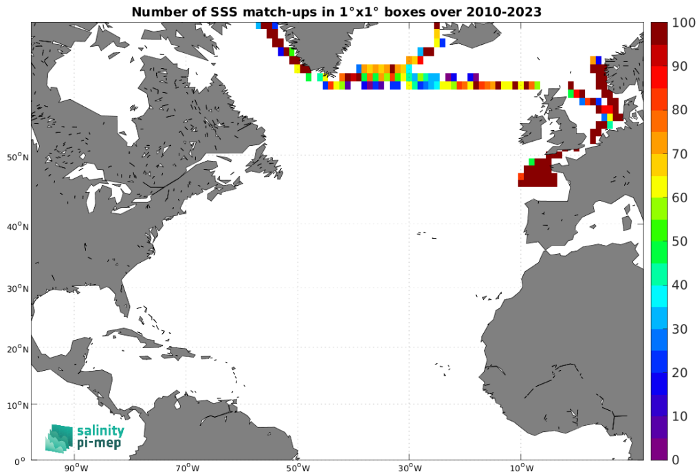
Figure 5: Number of SSS match-ups between TSG (Polarstern) SSS and the SMOS SSS L3 Arctic v2 - 18 Days (CATDS-CEC-LOCEAN) SSS product for the North Atlantic Ocean Pi-MEP region over 1^\circ \times 1^\circ boxes and for the full satellite product period.
