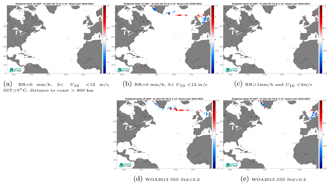
Figure 14: Temporal mean gridded over spatial boxes of size 1^\circ \times 1^\circ of \Delta\text{SSS} (SMOS SSS L3 Arctic v2 - 18 Days (CATDS-CEC-LOCEAN) - TSG (Polarstern)) for 5 different subdatasets corresponding to:RR=0 mm/h, 3 < U_{10} < 12 m/s, SST > 5^\circ\text{C} , distance to coast > 800 km (a), RR=0 mm/h, 3 < U_{10} < 12 m/s (b), RR > 1 mm/h and U_{10} < 4 m/s (c), WOA2013 SSS Std < 0.2 (d), WOA2013 SSS Std > 0.2 (e).
