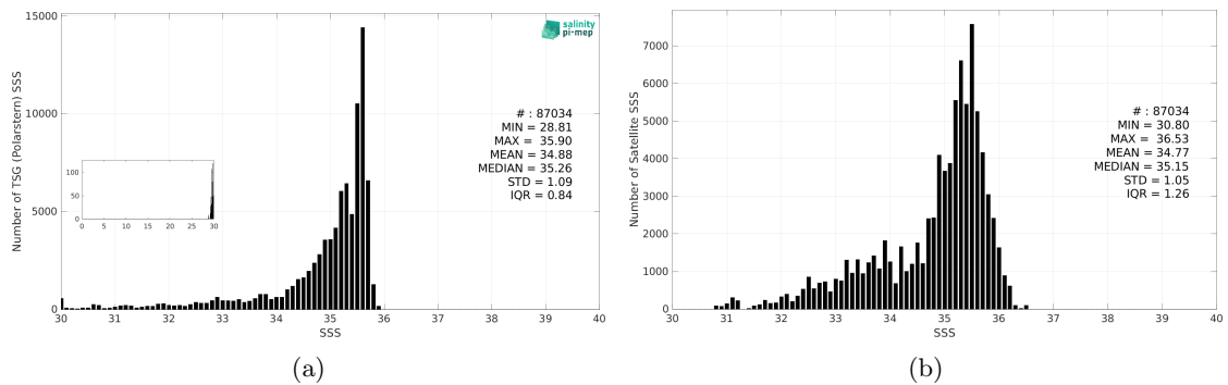
Figure 3: Histograms of SSS from TSG (Polarstern) (a) and SMOS SSS L3 Arctic v2 - 18 Days (CATDS-CEC-LOCEAN) (b) considering all match-up pairs per bins of 0.1 over the North Atlantic Ocean Pi-MEP region and for the full satellite product period.
