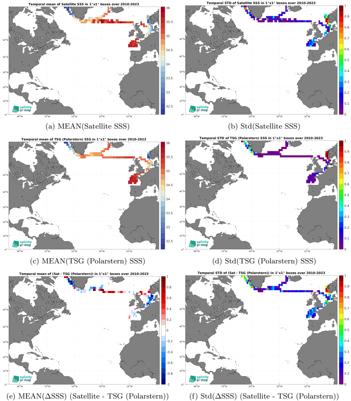
Figure 7: Temporal mean (left) and Std (right) of SSS from SMOS SSS L3 Arctic v2 - 18 Days (CATDS-CEC-LOCEAN) (top), TSG (Polarstern) (middle), and of \Delta SSS (Satellite - TSG (Polarstern)). Only match-up pairs are used to generate these maps.
