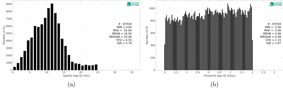
Figure 6: Histograms of the spatial (a) and temporal (b) lags between the location/time of the TSG (Polarstern) measurement and the date of the corresponding SMOS SSS L3 Arctic v2 - 18 Days (CATDS-CEC-LOCEAN) SSS pixel.
