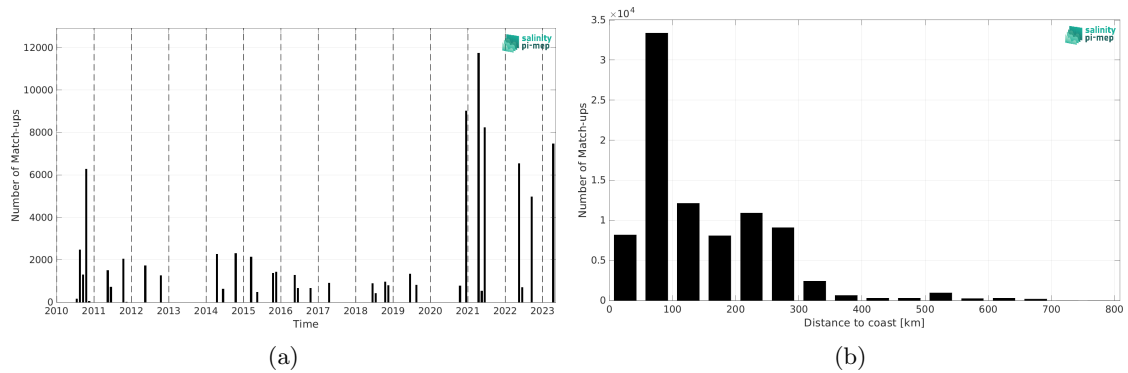
Figure 2: Number of match-ups between TSG (Polarstern) and SMOS SSS L3 Arctic v2 - 18 Days (CATDS-CEC-LOCEAN) SSS as a function of time (a) and as function of the distance to coast (b) over the North Atlantic Ocean Pi-MEP region and for the full satellite product period.
