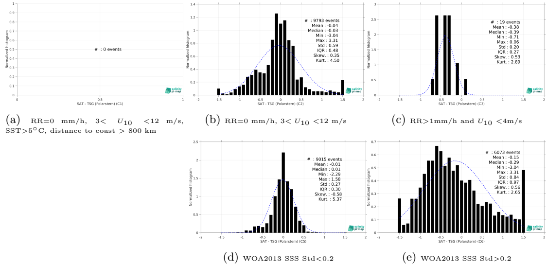
Figure 13: Normalized histogram of \Delta SSS (SMOS SSS L3 Arctic v2 - 18 Days (CATDS-CEC-LOCEAN) - TSG (Polarstern)) for 5 different subdatasets corresponding to: RR=0 mm/h, 3 < U_{10} < 12 m/s, SST > 5°C, distance to coast > 800 km (a), RR=0 mm/h, 3 < U_{10} < 12 m/s (b), RR > 1mm/h and U_{10} < 4 m/s (c), WOA2013 SSS Std < 0.2 (d), WOA2013 SSS Std > 0.2 (e).
