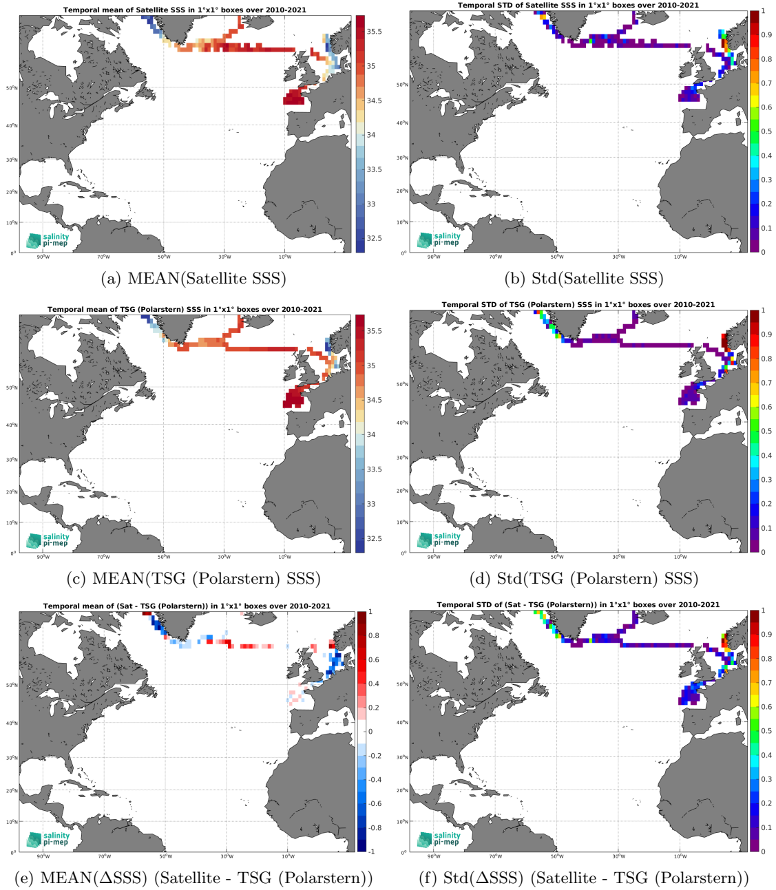
Figure 6: Temporal mean (left) and Std (right) of SSS from SMOS SSS L3 Arctic v2 - 18 Days (CATDS-CEC-LOCEAN) (top), TSG (Polarstern) (middle), and of \Delta SSS (Satellite - TSG (Polarstern)). Only match-up pairs are used to generate these maps.
