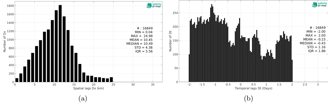
Figure 5: Histograms of the spatial (a) and temporal (b) lags between the location/time of the TSG (Polarstern) measurement and the date of the corresponding SMOS SSS L3 Arctic v2 - 18 Days (CATDS-CEC-LOCEAN) SSS pixel.
