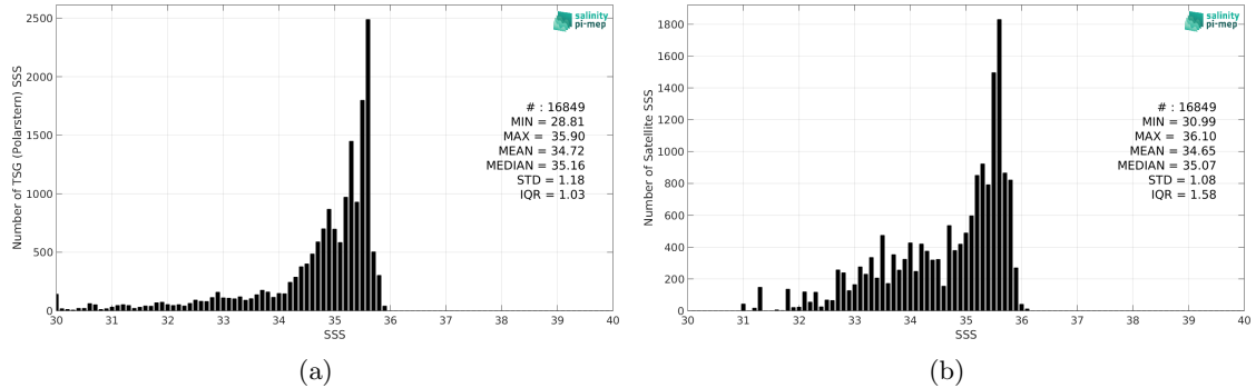
Figure 2: Histograms of SSS from TSG (Polarstern) (a) and SMOS SSS L3 Arctic v2 - 18 Days (CATDS-CEC-LOCEAN) (b) considering all match-up pairs per bins of 0.1 over the North Atlantic Ocean Pi-MEP region and for the full satellite product period.
