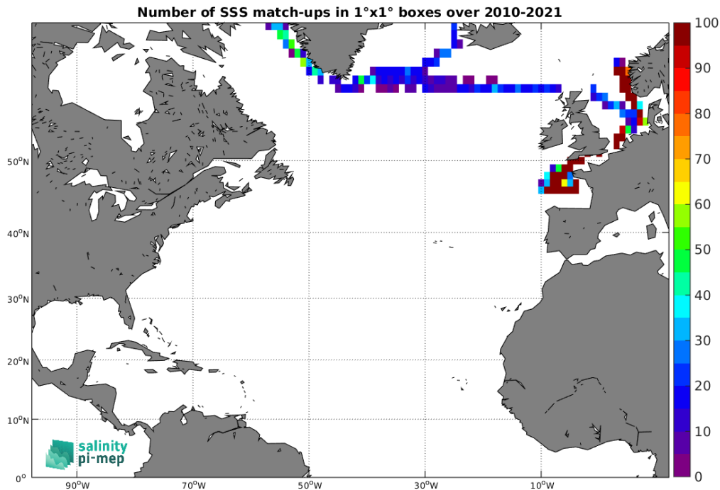
Figure 4: Number of SSS match-ups between TSG (Polarstern) SSS and the SMOS SSS L3 Arctic v2 - 18 Days (CATDS-CEC-LOCEAN) SSS product for the North Atlantic Ocean Pi-MEP region over 1^\circ \times 1^\circ boxes and for the full satellite product period.
