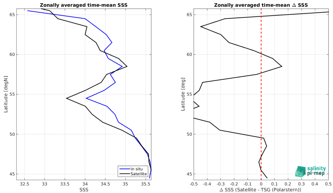
Figure 8: Left panel: Zonal mean SSS from SMOS SSS L3 Arctic v2 - 18 Days (CATDS-CEC-LOCEAN) satellite product (black) and from TSG (Polarstern) (blue). Right panel: Zonal mean of \Delta SSS (Satellite - TSG (Polarstern)) for all the collected Pi-MEP match-up pairs estimated over the full satellite product period.
