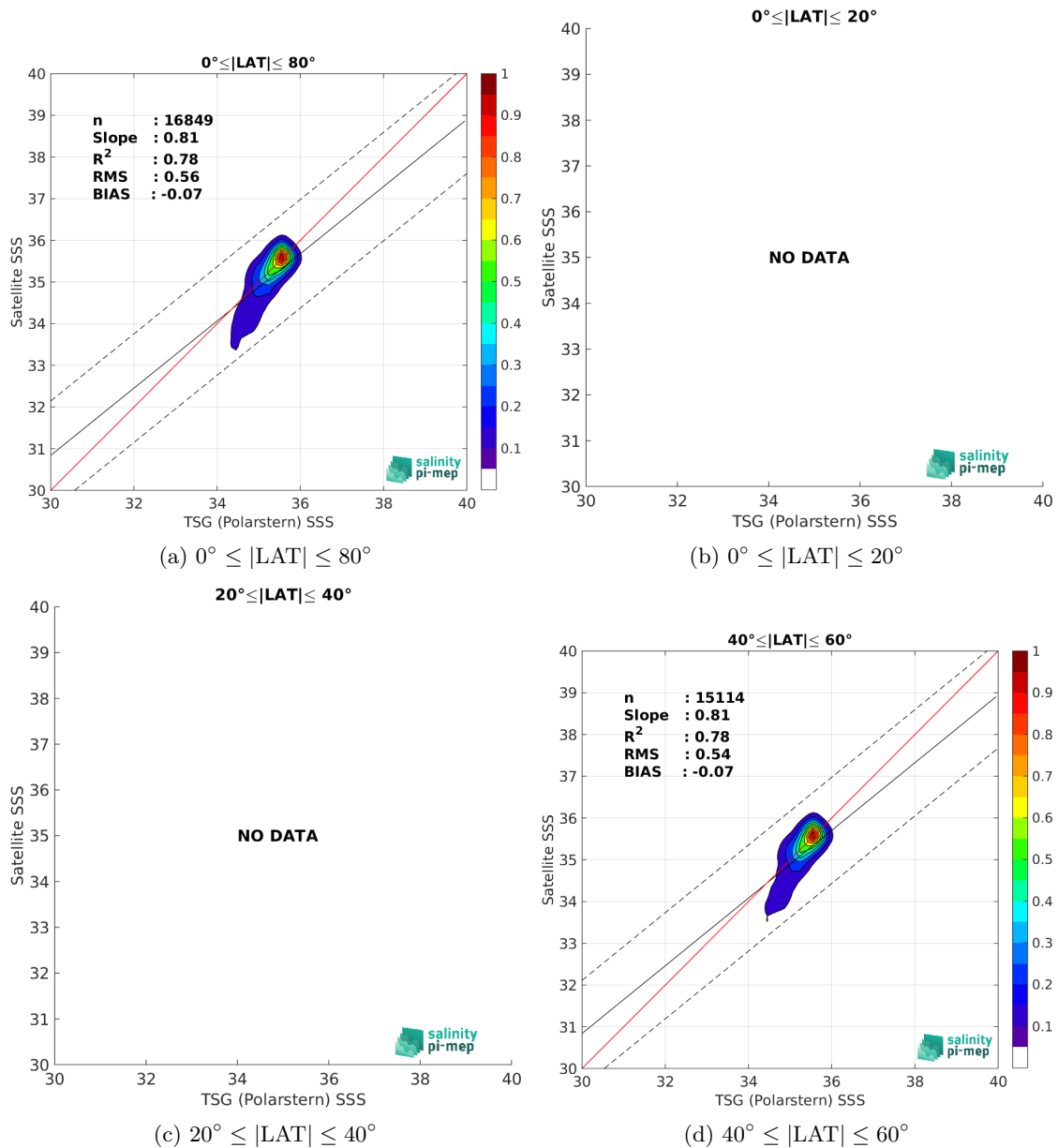
Figure 9: Contour maps of the concentration of SMOS SSS L3 Arctic v2 - 18 Days (CATDS-CEC-LOCEAN) SSS (y-axis) versus TSG (Polarstern) SSS (x-axis) at match-up pairs for different latitude bands. For each plot, the red line shows x=y . The black thin and dashed lines indicate a linear fit through the data cloud and the \pm 95\% confidence levels, respectively. The number match-up pairs n , the slope and R^2 coefficient of the linear fit, the root mean square (RMS) and the mean bias between satellite and in situ data are indicated for each latitude band in each plots.
