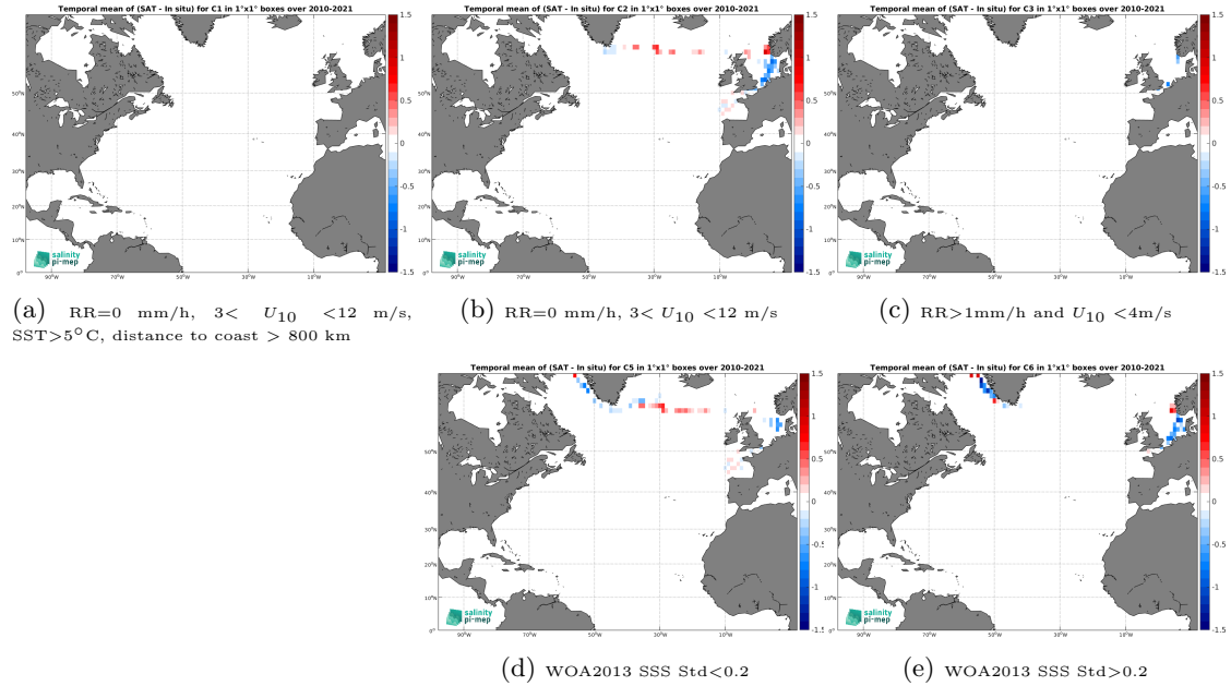
Figure 12: Temporal mean gridded over spatial boxes of size 1^{\circ}\times 1^{\circ} of \Delta\text{SSS} (SMOS SSS L3 Arctic v2 - 18 Days (CATDS-CEC-LOCEAN) - TSG (Polarstern)) for 5 different subdatasets corresponding to: RR=0 mm/h, 3 < U_{10} < 12 m/s, SST > 5^{\circ}\text{C} , distance to coast > 800 km (a), RR=0 mm/h, 3 < U_{10} < 12 m/s (b), RR > 1 mm/h and U_{10} < 4 m/s (c), WOA2013 SSS Std < 0.2 (d), WOA2013 SSS Std > 0.2 (e).
