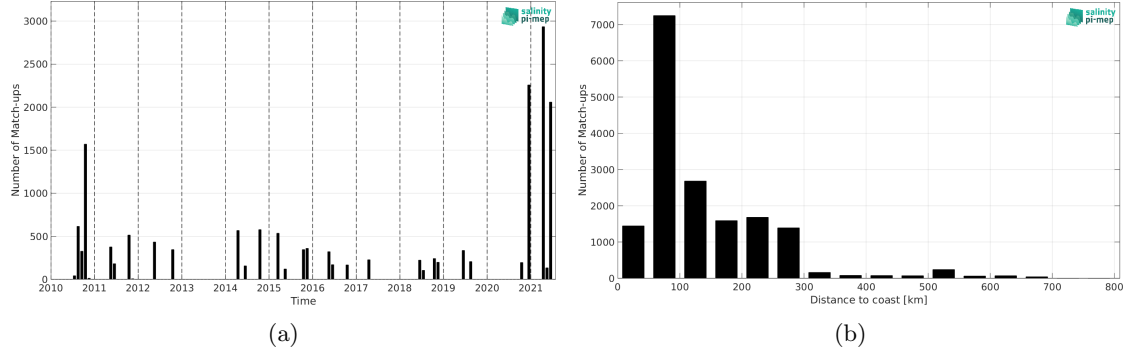
Figure 1: Number of match-ups between TSG (Polarstern) and SMOS SSS L3 Arctic v2 - 18 Days (CATDS-CEC-LOCEAN) SSS as a function of time (a) and as function of the distance to coast (b) over the North Atlantic Ocean Pi-MEP region and for the full satellite product period.
