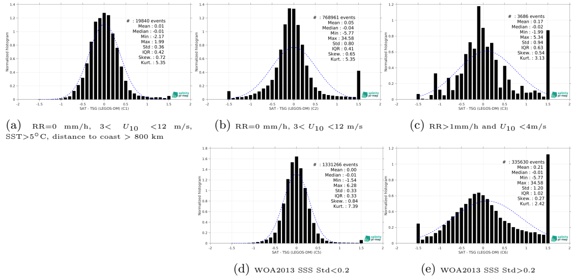
Figure 13: Normalized histogram of \Delta SSS (SMOS SSS L3 Arctic v2 - 18 Days (CATDS-CEC-LOCEAN) - TSG (LEGOS-DM)) for 5 different subdatasets corresponding to: RR=0 mm/h, 3 < U_{10} < 12 m/s, SST>5°C, distance to coast > 800 km (a), RR=0 mm/h, 3 < U_{10} < 12 m/s (b), RR>1mm/h and U_{10} < 4 m/s (c), WOA2013 SSS Std<0.2 (d), WOA2013 SSS Std>0.2 (e).
