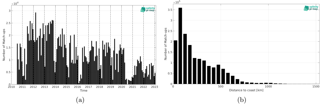
Figure 1: Number of match-ups between TSG (LEGOS-DM) and SMOS SSS L3 Arctic v2 - 18 Days (CATDS-CEC-LOCEAN) SSS as a function of time (a) and as function of the distance to coast (b) over the North Atlantic Ocean Pi-MEP region and for the full satellite product period.
