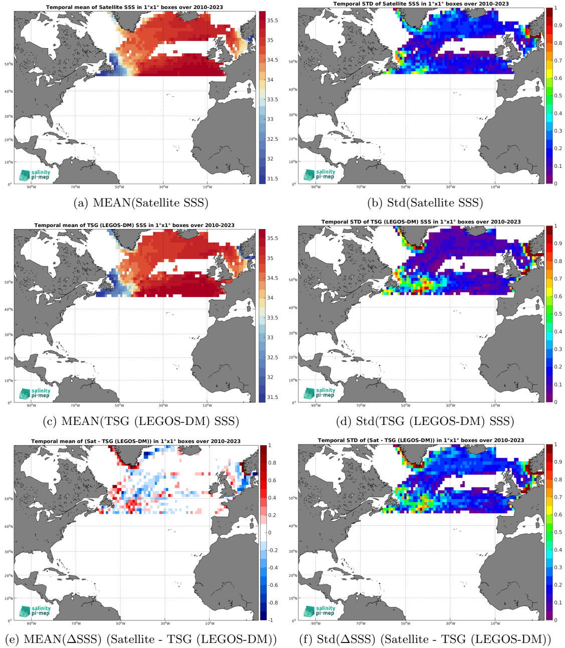
Figure 6: Temporal mean (left) and Std (right) of SSS from SMOS SSS L3 Arctic v2 - 18 Days (CATDS-CEC-LOCEAN) (top), TSG (LEGOS-DM) (middle), and of \Delta SSS (Satellite - TSG (LEGOS-DM)). Only match-up pairs are used to generate these maps.
