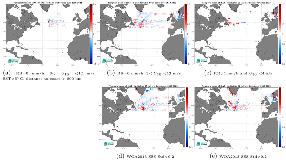
Figure 12: Temporal mean gridded over spatial boxes of size 1^{\circ}\times 1^{\circ} of \Delta\text{SSS} (SMOS SSS L3 Arctic v2 - 18 Days (CATDS-CEC-LOCEAN) - TSG (LEGOS-DM)) for 5 different subdatasets corresponding to:RR=0 mm/h, 3 < U_{10} < 12 m/s, SST > 5^{\circ}\text{C} , distance to coast > 800 km (a), RR=0 mm/h, 3 < U_{10} < 12 m/s (b), RR > 1 mm/h and U_{10} < 4 m/s (c), WOA2013 SSS Std < 0.2 (d), WOA2013 SSS Std > 0.2 (e).
