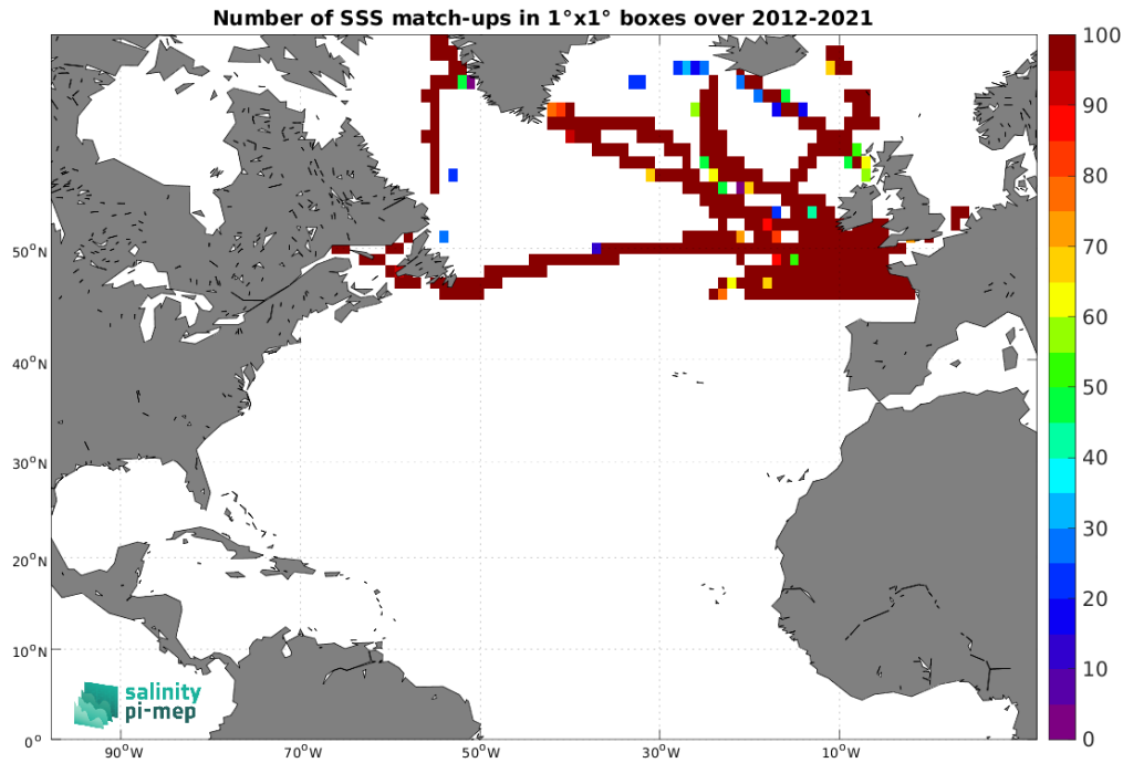
Figure 5: Number of SSS match-ups between TSG (GOSUD-Sailing-ship) SSS and the SMOS SSS L3 Arctic v2 - 18 Days (CATDS-CEC-LOCEAN) SSS product for the North Atlantic Ocean Pi-MEP region over 1^\circ \times 1^\circ boxes and for the full satellite product period.
