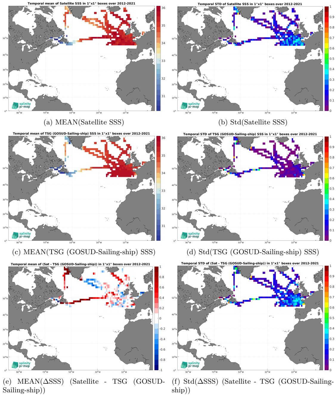
Figure 7: Temporal mean (left) and Std (right) of SSS from SMOS SSS L3 Arctic v2 - 18 Days (CATDS-CEC-LOCEAN) (top), TSG (GOSUD-Sailing-ship) (middle), and of \Delta SSS (Satellite - TSG (GOSUD-Sailing-ship)). Only match-up pairs are used to generate these maps.
