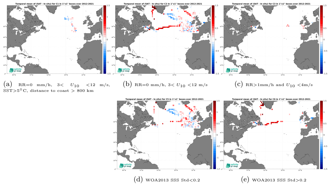
Figure 14: Temporal mean gridded over spatial boxes of size 1^\circ \times 1^\circ of \Delta SSS (SMOS SSS L3 Arctic v2 - 18 Days (CATDS-CEC-LOCEAN) - TSG (GOSUD-Sailing-ship)) for 5 different subdatasets corresponding to:RR=0 mm/h, 3 < U_{10} < 12 m/s, SST >5^\circ\text{C} , distance to coast > 800 km (a), RR=0 mm/h, 3 < U_{10} < 12 m/s (b), RR >1 mm/h and U_{10} < 4 m/s (c), WOA2013 SSS Std <0.2 (d), WOA2013 SSS Std >0.2 (e).
