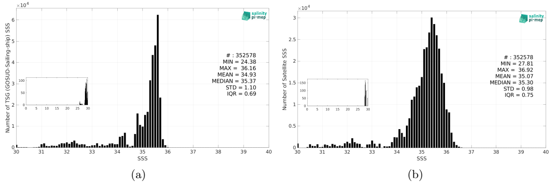
Figure 3: Histograms of SSS from TSG (GOSUD-Sailing-ship) (a) and SMOS SSS L3 Arctic v2 - 18 Days (CATDS-CEC-LOCEAN) (b) considering all match-up pairs per bins of 0.1 over the North Atlantic Ocean Pi-MEP region and for the full satellite product period.
