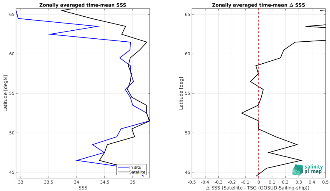
Figure 8: Left panel: Zonal mean SSS from SMOS SSS L3 Arctic v2 - 18 Days (CATDS-CEC-LOCEAN) satellite product (black) and from TSG (GOSUD-Sailing-ship) (blue). Right panel: Zonal mean of \Delta SSS (Satellite - TSG (GOSUD-Sailing-ship)) for all the collected Pi-MEP match-up pairs estimated over the full satellite product period.
