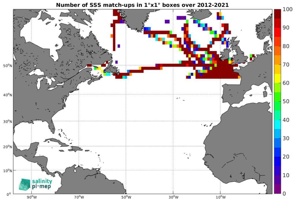
Figure 4: Number of SSS match-ups between TSG (GOSUD-Sailing-ship) SSS and the SMOS SSS L3 Arctic v2 - 18 Days (CATDS-CEC-LOCEAN) SSS product for the North Atlantic Ocean Pi-MEP region over 1^\circ \times 1^\circ boxes and for the full satellite product period.
