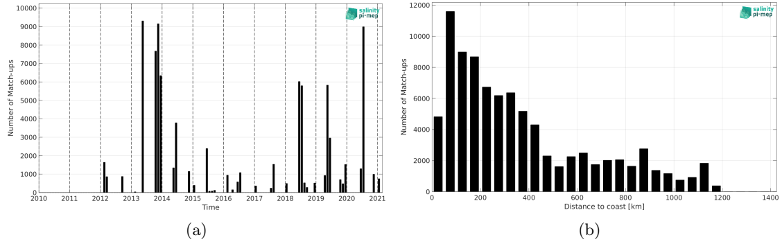
Figure 1: Number of match-ups between TSG (GOSUD-Sailing-ship) and SMOS SSS L3 Arctic v2 - 18 Days (CATDS-CEC-LOCEAN) SSS as a function of time (a) and as function of the distance to coast (b) over the North Atlantic Ocean Pi-MEP region and for the full satellite product period.
