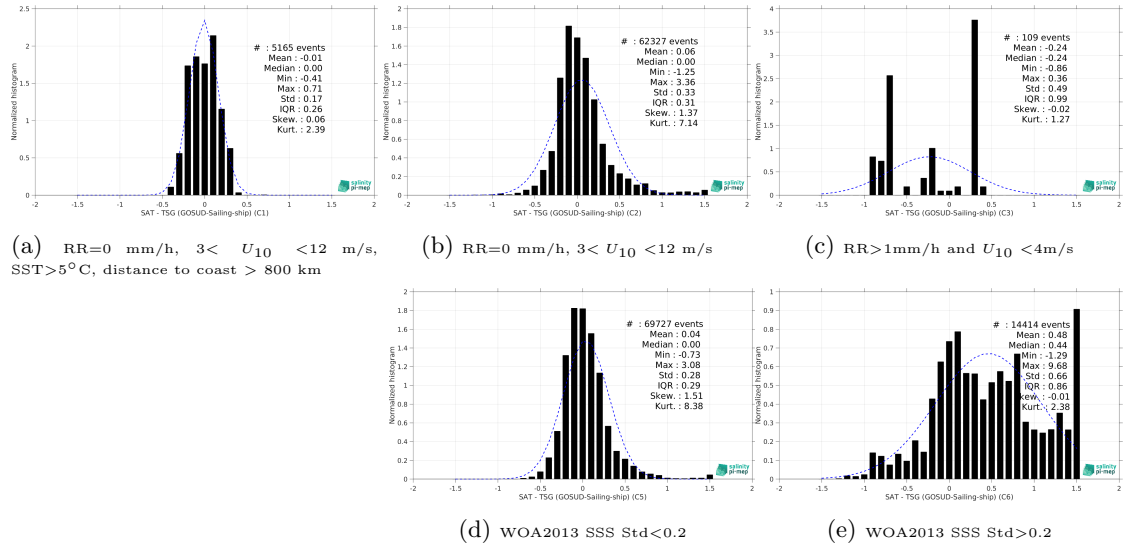
Figure 13: Normalized histogram of \Delta SSS (SMOS SSS L3 Arctic v2 - 18 Days (CATDS-CEC-LOCEAN) - TSG (GOSUD-Sailing-ship)) for 5 different subdatasets corresponding to: RR=0 mm/h, 3 < U_{10} < 12 m/s, SST > 5°C, distance to coast > 800 km (a), RR=0 mm/h, 3 < U_{10} < 12 m/s (b), RR > 1mm/h and U_{10} < 4 m/s (c), WOA2013 SSS Std < 0.2 (d), WOA2013 SSS Std > 0.2 (e).
