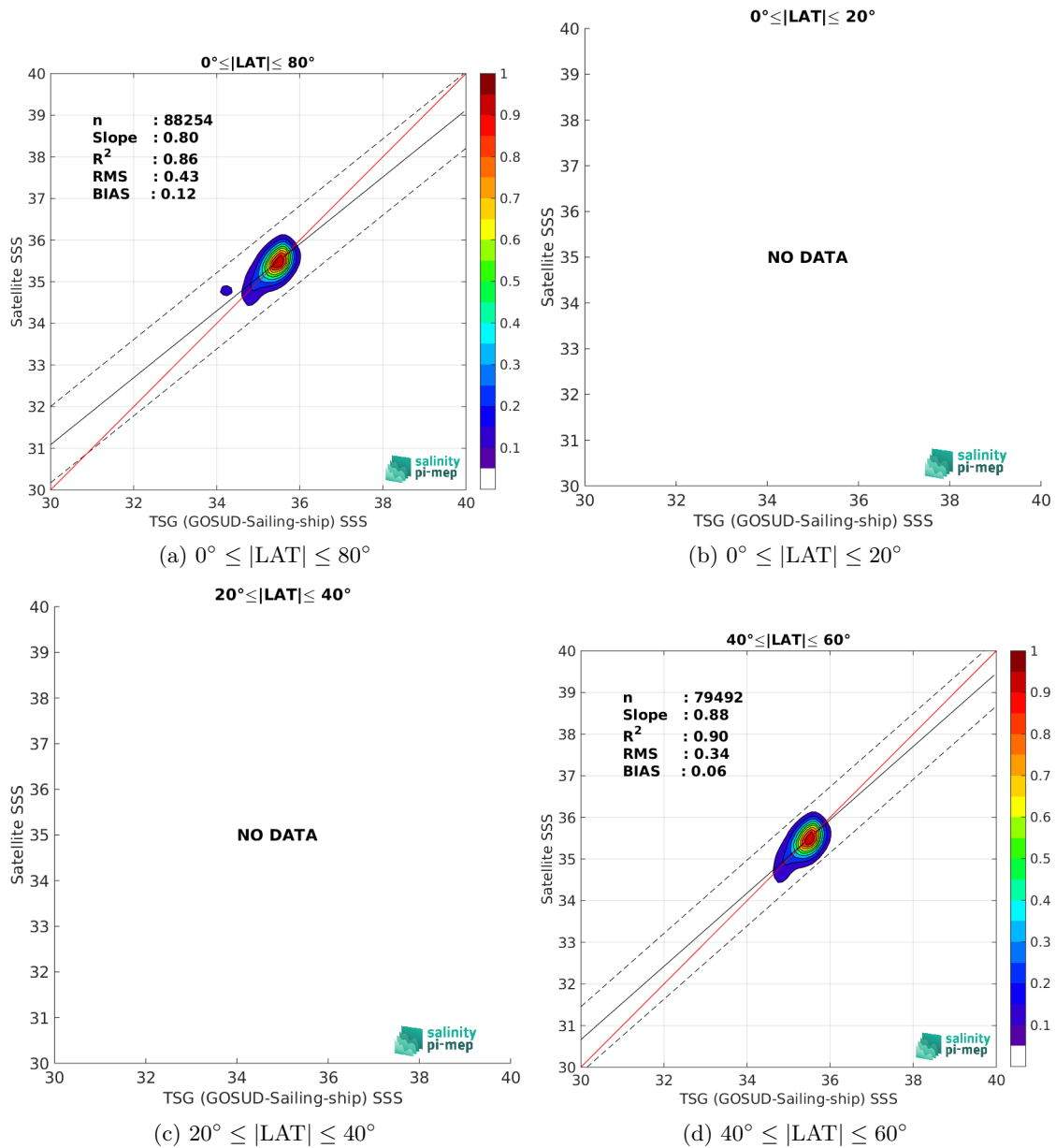
Figure 9: Contour maps of the concentration of SMOS SSS L3 Arctic v2 - 18 Days (CATDS-CEC-LOCEAN) SSS (y-axis) versus TSG (GOSUD-Sailing-ship) SSS (x-axis) at match-up pairs for different latitude bands. For each plot, the red line shows x=y . The black thin and dashed lines indicate a linear fit through the data cloud and the \pm 95\% confidence levels, respectively. The number match-up pairs n , the slope and R^2 coefficient of the linear fit, the root mean square (RMS) and the mean bias between satellite and in situ data are indicated for each latitude band in each plots.
