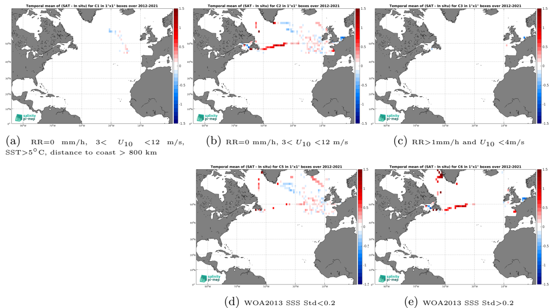
Figure 12: Temporal mean gridded over spatial boxes of size 1^{\circ}\times 1^{\circ} of \Delta SSS (SMOS SSS L3 Arctic v2 - 18 Days (CATDS-CEC-LOCEAN) - TSG (GOSUD-Sailing-ship)) for 5 different subdatasets corresponding to:RR=0 mm/h, 3 < U_{10} < 12 m/s, SST > 5^{\circ}\text{C} , distance to coast > 800 km (a), RR=0 mm/h, 3 < U_{10} < 12 m/s (b), RR > 1 mm/h and U_{10} < 4 m/s (c), WOA2013 SSS Std < 0.2 (d), WOA2013 SSS Std > 0.2 (e).
