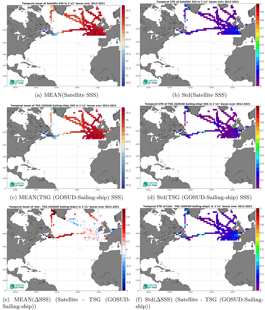
Figure 6: Temporal mean (left) and Std (right) of SSS from SMOS SSS L3 Arctic v2 - 18 Days (CATDS-CEC-LOCEAN) (top), TSG (GOSUD-Sailing-ship) (middle), and of \Delta SSS (Satellite - TSG (GOSUD-Sailing-ship)). Only match-up pairs are used to generate these maps.
