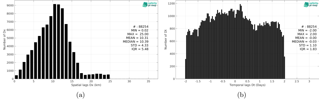
Figure 5: Histograms of the spatial (a) and temporal (b) lags between the location/time of the TSG (GOSUD-Sailing-ship) measurement and the date of the corresponding SMOS SSS L3 Arctic v2 - 18 Days (CATDS-CEC-LOCEAN) SSS pixel.
