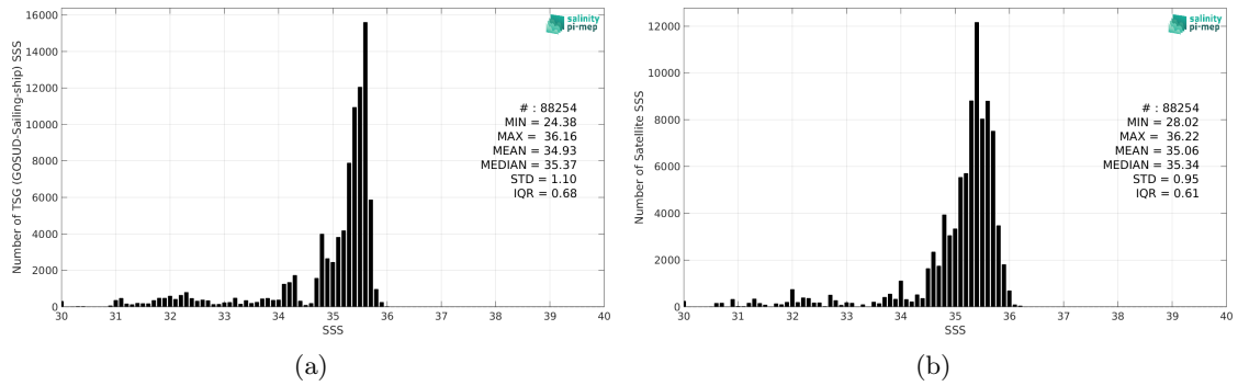
Figure 2: Histograms of SSS from TSG (GOSUD-Sailing-ship) (a) and SMOS SSS L3 Arctic v2 - 18 Days (CATDS-CEC-LOCEAN) (b) considering all match-up pairs per bins of 0.1 over the North Atlantic Ocean Pi-MEP region and for the full satellite product period.
