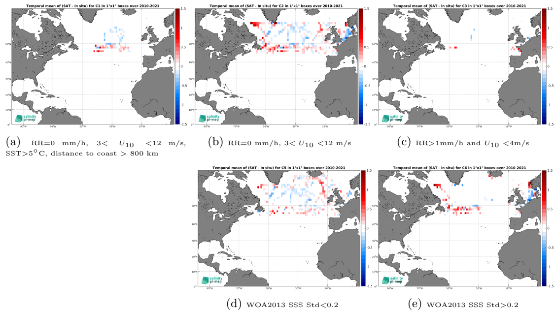
Figure 12: Temporal mean gridded over spatial boxes of size 1^{\circ}\times 1^{\circ} of \Delta SSS (SMOS SSS L3 Arctic v2 - 18 Days (CATDS-CEC-LOCEAN) - TSG (GOSUD-Research-vessel)) for 5 different subdatasets corresponding to:RR=0 mm/h, 3 < U_{10} < 12 m/s, SST >5^{\circ}\text{C} , distance to coast > 800 km (a), RR=0 mm/h, 3 < U_{10} < 12 m/s (b), RR >1 mm/h and U_{10} < 4 m/s (c), WOA2013 SSS Std <0.2 (d), WOA2013 SSS Std >0.2 (e).
