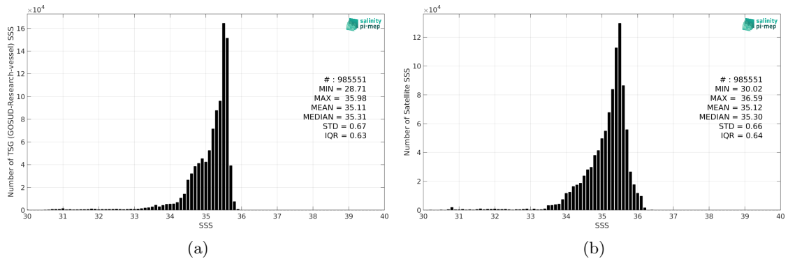
Figure 2: Histograms of SSS from TSG (GOSUD-Research-vessel) (a) and SMOS SSS L3 Arctic v2 - 18 Days (CATDS-CEC-LOCEAN) (b) considering all match-up pairs per bins of 0.1 over the North Atlantic Ocean Pi-MEP region and for the full satellite product period.
