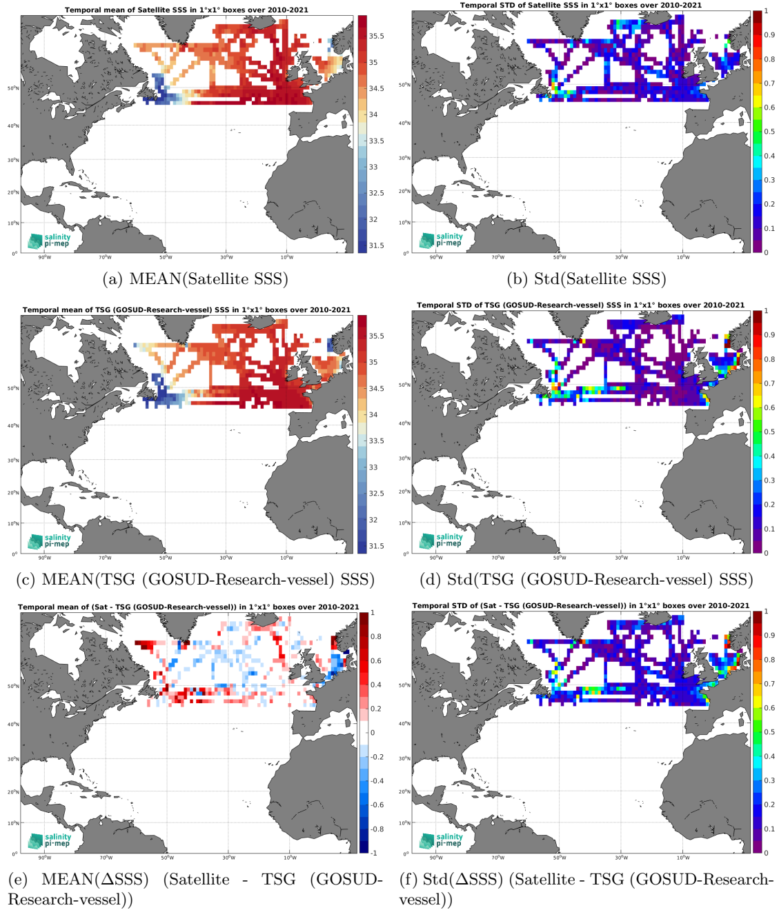
Figure 6: Temporal mean (left) and Std (right) of SSS from SMOS SSS L3 Arctic v2 - 18 Days (CATDS-CEC-LOCEAN) (top), TSG (GOSUD-Research-vessel) (middle), and of \Delta SSS (Satellite - TSG (GOSUD-Research-vessel)). Only match-up pairs are used to generate these maps.
