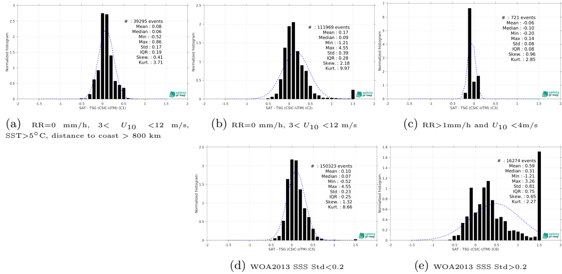
Figure 13: Normalized histogram of \Delta SSS (SMOS SSS L3 Arctic v2 - 18 Days (CATDS-CEC-LOCEAN) - TSG (CSIC-UTM)) for 5 different subdatasets corresponding to: RR=0 mm/h, 3 < U_{10} < 12 m/s, SST>5°C, distance to coast > 800 km (a), RR=0 mm/h, 3 < U_{10} < 12 m/s (b), RR>1mm/h and U_{10} < 4 m/s (c), WOA2013 SSS Std<0.2 (d), WOA2013 SSS Std>0.2 (e).
