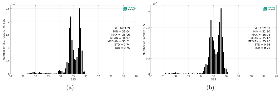
Figure 2: Histograms of SSS from TSG (CSIC-UTM) (a) and SMOS SSS L3 Arctic v2 - 18 Days (CATDS-CEC-LOCEAN) (b) considering all match-up pairs per bins of 0.1 over the North Atlantic Ocean Pi-MEP region and for the full satellite product period.
