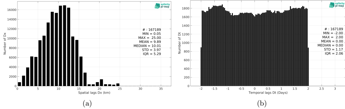
Figure 5: Histograms of the spatial (a) and temporal (b) lags between the location/time of the TSG (CSIC-UTM) measurement and the date of the corresponding SMOS SSS L3 Arctic v2 - 18 Days (CATDS-CEC-LOCEAN) SSS pixel.
