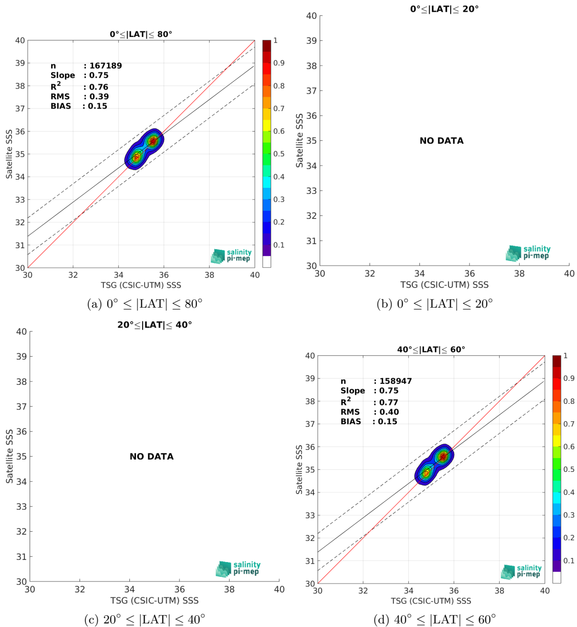
Figure 9: Contour maps of the concentration of SMOS SSS L3 Arctic v2 - 18 Days (CATDS-CEC-LOCEAN) SSS (y-axis) versus TSG (CSIC-UTM) SSS (x-axis) at match-up pairs for different latitude bands. For each plot, the red line shows x=y . The black thin and dashed lines indicate a linear fit through the data cloud and the \pm 95\% confidence levels, respectively. The number match-up pairs n , the slope and R^2 coefficient of the linear fit, the root mean square (RMS) and the mean bias between satellite and in situ data are indicated for each latitude band in each plots.
