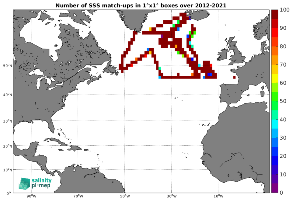
Figure 4: Number of SSS match-ups between TSG (CSIC-UTM) SSS and the SMOS SSS L3 Arctic v2 - 18 Days (CATDS-CEC-LOCEAN) SSS product for the North Atlantic Ocean Pi-MEP region over 1^\circ \times 1^\circ boxes and for the full satellite product period.
