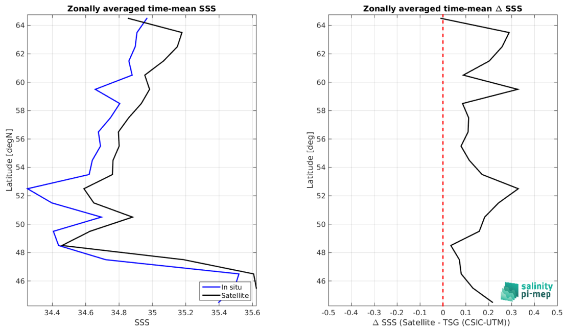
Figure 8: Left panel: Zonal mean SSS from SMOS SSS L3 Arctic v2 - 18 Days (CATDS-CEC-LOCEAN) satellite product (black) and from TSG (CSIC-UTM) (blue). Right panel: Zonal mean of \Delta SSS (Satellite - TSG (CSIC-UTM)) for all the collected Pi-MEP match-up pairs estimated over the full satellite product period.
