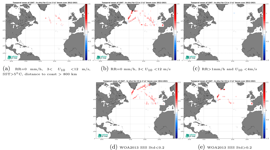
Figure 12: Temporal mean gridded over spatial boxes of size 1^{\circ}\times 1^{\circ} of \Delta\text{SSS} (SMOS SSS L3 Arctic v2 - 18 Days (CATDS-CEC-LOCEAN) - TSG (CSIC-UTM)) for 5 different subdatasets corresponding to:RR=0 mm/h, 3 < U_{10} < 12 m/s, SST > 5^{\circ}\text{C} , distance to coast > 800 km (a), RR=0 mm/h, 3 < U_{10} < 12 m/s (b), RR > 1 mm/h and U_{10} < 4 m/s (c), WOA2013 SSS Std < 0.2 (d), WOA2013 SSS Std > 0.2 (e).
