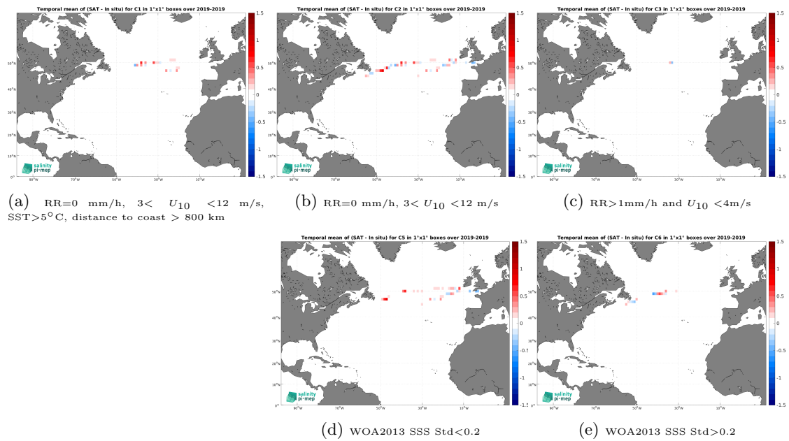
Figure 14: Temporal mean gridded over spatial boxes of size 1^\circ \times 1^\circ of \Delta\text{SSS} (SMOS SSS L3 Arctic v2 - 18 Days (CATDS-CEC-LOCEAN) - Saildrone) for 5 different subdatasets corresponding to:RR=0 mm/h, 3 < U_{10} < 12 m/s, SST >5^\circ\text{C} , distance to coast > 800 km (a), RR=0 mm/h, 3 < U_{10} < 12 m/s (b), RR >1 mm/h and U_{10} < 4 m/s (c), WOA2013 SSS Std <0.2 (d), WOA2013 SSS Std >0.2 (e).
