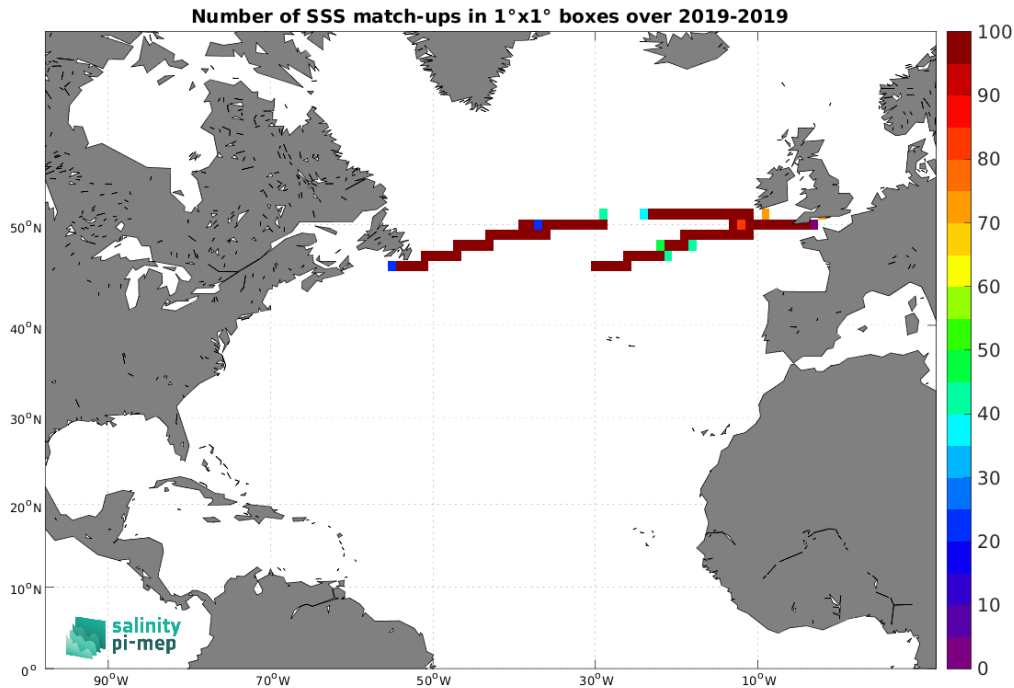
Figure 5: Number of SSS match-ups between Saildrone SSS and the SMOS SSS L3 Arctic v2 - 18 Days (CATDS-CEC-LOCEAN) SSS product for the North Atlantic Ocean Pi-MEP region over 1^\circ \times 1^\circ boxes and for the full satellite product period.
