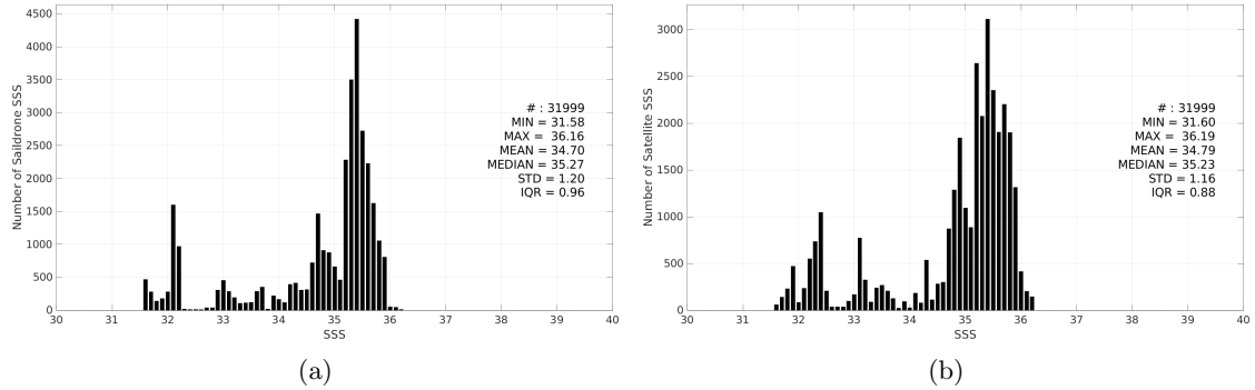
Figure 3: Histograms of SSS from Saildrone (a) and SMOS SSS L3 Arctic v2 - 18 Days (CATDS-CEC-LOCEAN) (b) considering all match-up pairs per bins of 0.1 over the North Atlantic Ocean Pi-MEP region and for the full satellite product period.
