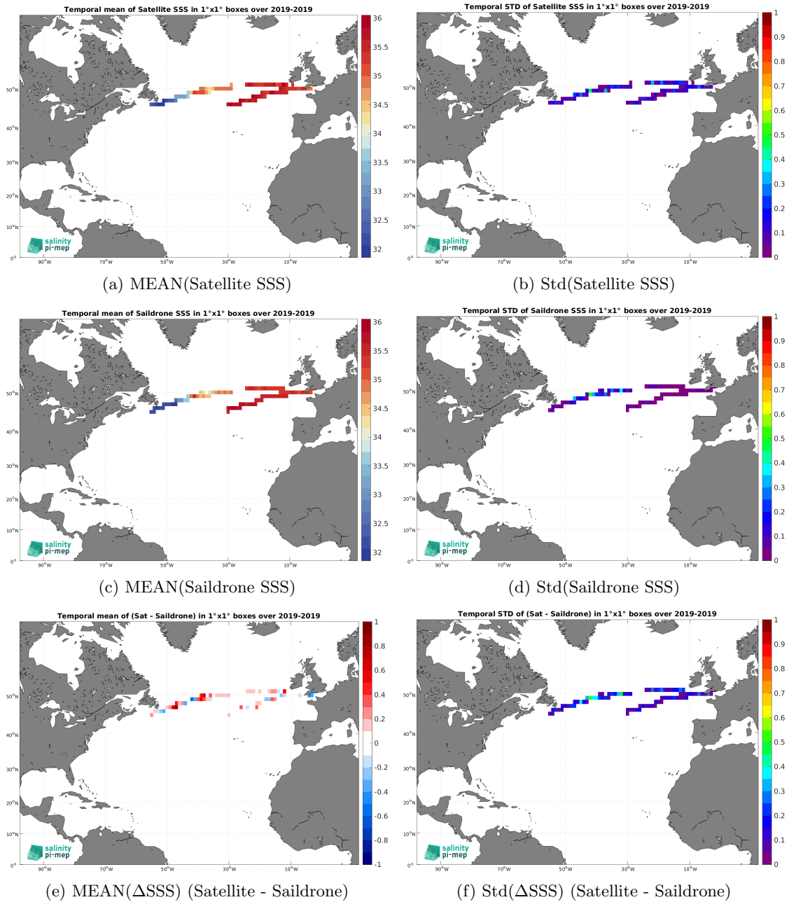
Figure 7: Temporal mean (left) and Std (right) of SSS from SMOS SSS L3 Arctic v2 - 18 Days (CATDS-CEC-LOCEAN) (top), Saildrone (middle), and of \Delta SSS (Satellite - Saildrone). Only match-up pairs are used to generate these maps.
