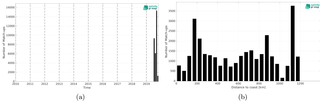
Figure 2: Number of match-ups between Saildrone and SMOS SSS L3 Arctic v2 - 18 Days (CATDS-CEC-LOCEAN) SSS as a function of time (a) and as function of the distance to coast (b) over the North Atlantic Ocean Pi-MEP region and for the full satellite product period.
