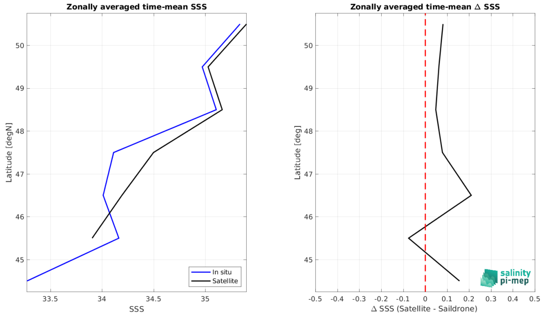
Figure 9: Left panel: Zonal mean SSS from SMOS SSS L3 Arctic v2 - 18 Days (CATDS-CEC-LOCEAN) satellite product (black) and from Saildrone (blue). Right panel: Zonal mean of \Delta SSS (Satellite - Saildrone) for all the collected Pi-MEP match-up pairs estimated over the full satellite product period.
