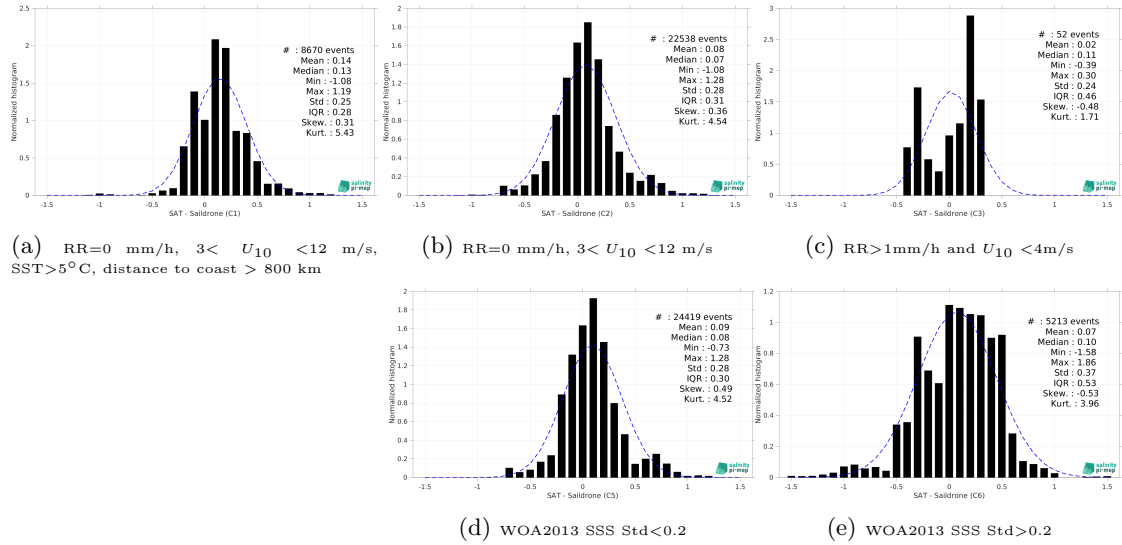
Figure 15: Normalized histogram of \Delta SSS (SMOS SSS L3 Arctic v2 - 18 Days (CATDS-CEC-LOCEAN) - Saildrone) for 5 different subdatasets corresponding to: RR=0 mm/h, 3 < U_{10} < 12 m/s, SST>5°C, distance to coast > 800 km (a), RR=0 mm/h, 3 < U_{10} < 12 m/s (b), RR>1mm/h and U_{10} < 4 m/s (c), WOA2013 SSS Std<0.2 (d), WOA2013 SSS Std>0.2 (e).
