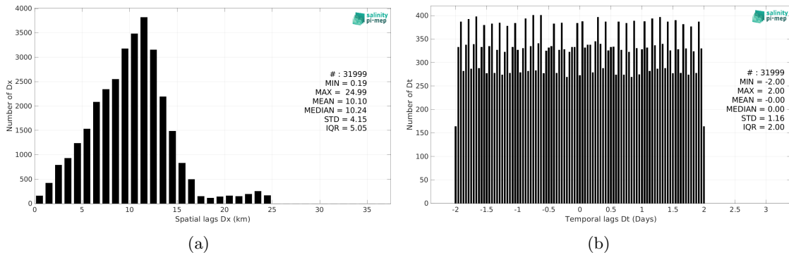
Figure 6: Histograms of the spatial (a) and temporal (b) lags between the location/time of the Saildrone measurement and the date of the corresponding SMOS SSS L3 Arctic v2 - 18 Days (CATDS-CEC-LOCEAN) SSS pixel.
