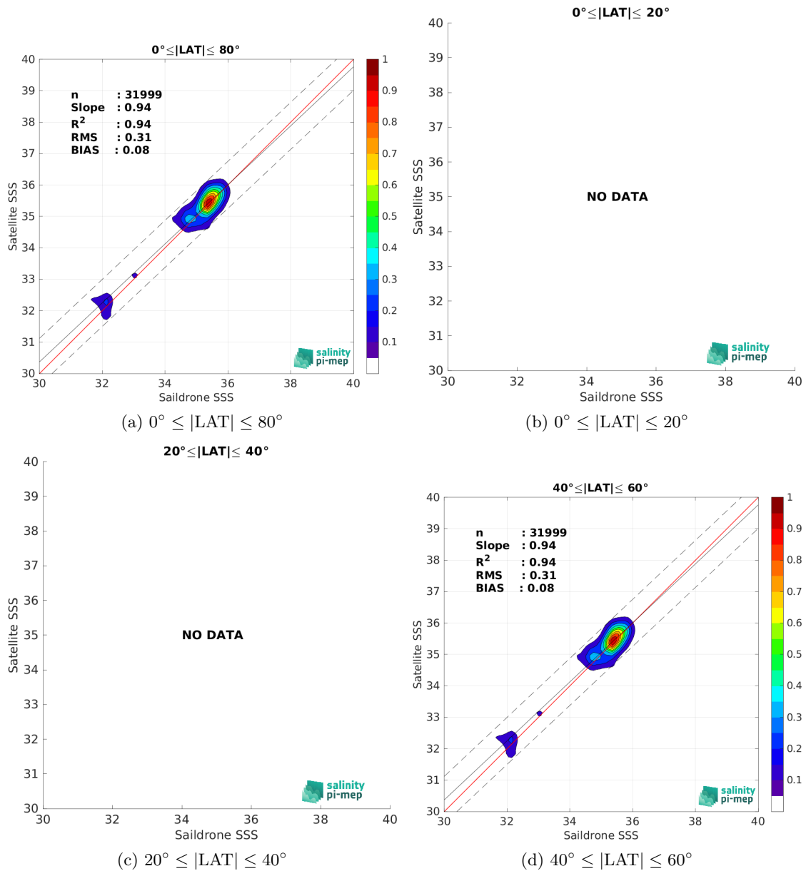
Figure 10: Contour maps of the concentration of SMOS SSS L3 Arctic v2 - 18 Days (CATDS-CEC-LOCEAN) SSS (y-axis) versus Saildrone SSS (x-axis) at match-up pairs for different latitude bands. For each plot, the red line shows x=y . The black thin and dashed lines indicate a linear fit through the data cloud and the \pm 95\% confidence levels, respectively. The number match-up pairs n , the slope and R^2 coefficient of the linear fit, the root mean square (RMS) and the mean bias between satellite and in situ data are indicated for each latitude band in each plots.
