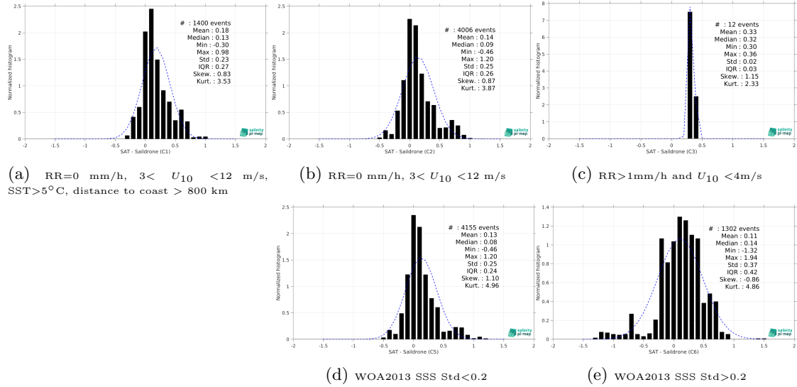
Figure 13: Normalized histogram of \Delta SSS (SMOS SSS L3 Arctic v2 - 18 Days (CATDS-CEC-LOCEAN) - Saldrone) for 5 different subdatasets corresponding to: RR=0 mm/h, 3 < U_{10} < 12 m/s, SST > 5°C, distance to coast > 800 km (a), RR=0 mm/h, 3 < U_{10} < 12 m/s (b), RR > 1mm/h and U_{10} < 4 m/s (c), WOA2013 SSS Std < 0.2 (d), WOA2013 SSS Std > 0.2 (e).
