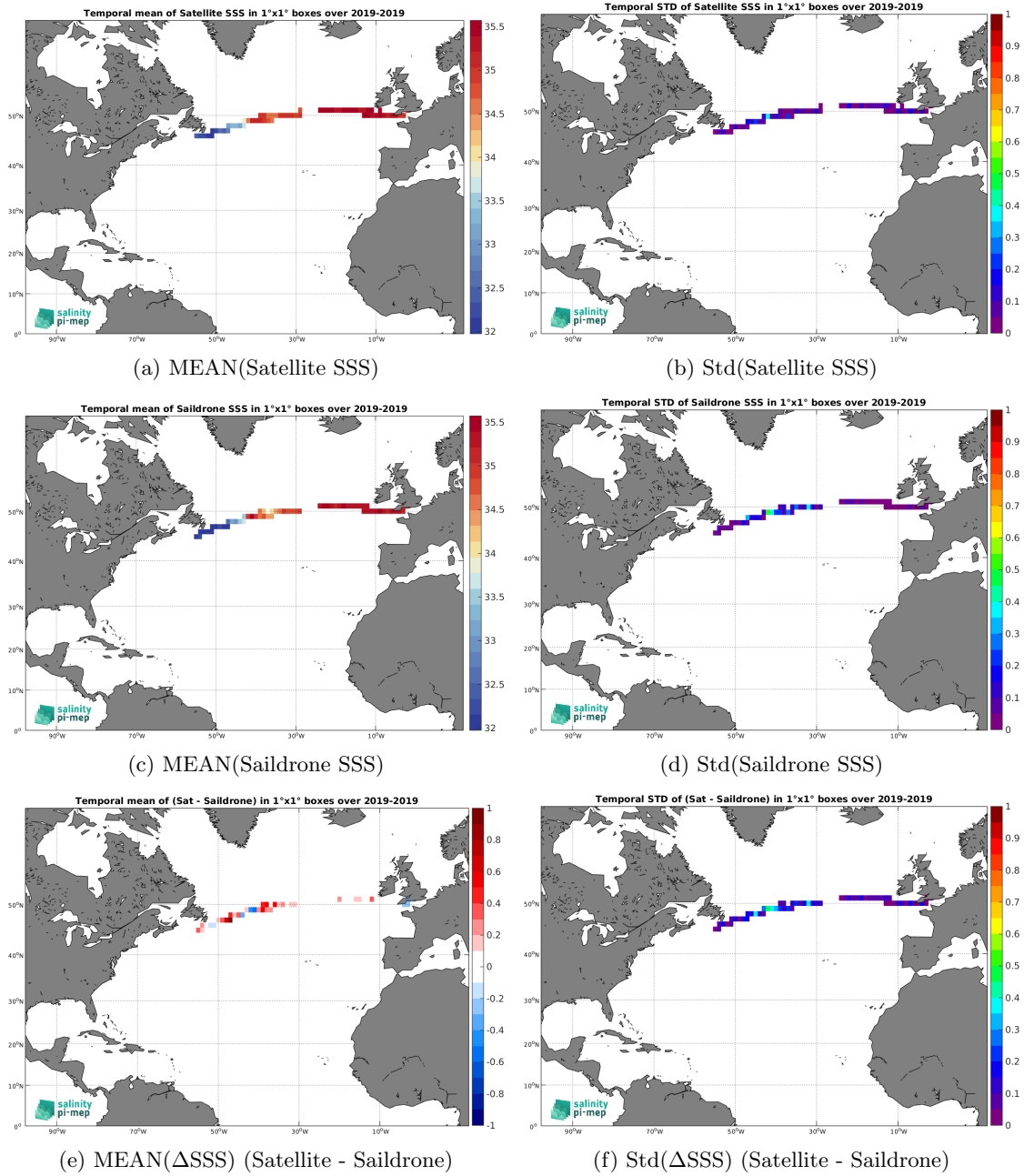
Figure 6: Temporal mean (left) and Std (right) of SSS from SMOS SSS L3 Arctic v2 - 18 Days (CATDS-CEC-LOCEAN) (top), Saildrone (middle), and of \Delta SSS (Satellite - Saildrone). Only match-up pairs are used to generate these maps.
