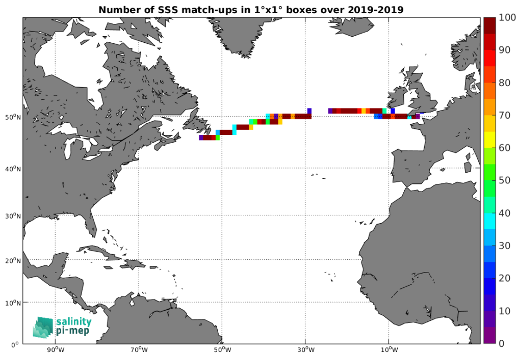
Figure 4: Number of SSS match-ups between Saildrone SSS and the SMOS SSS L3 Arctic v2 - 18 Days (CATDS-CEC-LOCEAN) SSS product for the North Atlantic Ocean Pi-MEP region over 1^\circ \times 1^\circ boxes and for the full satellite product period.
