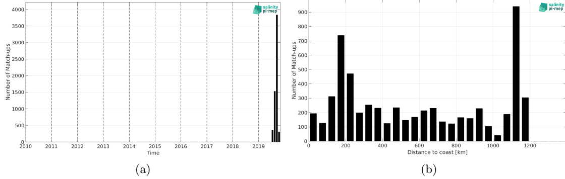
Figure 1: Number of match-ups between Saildrone and SMOS SSS L3 Arctic v2 - 18 Days (CATDS-CEC-LOCEAN) SSS as a function of time (a) and as function of the distance to coast (b) over the North Atlantic Ocean Pi-MEP region and for the full satellite product period.
