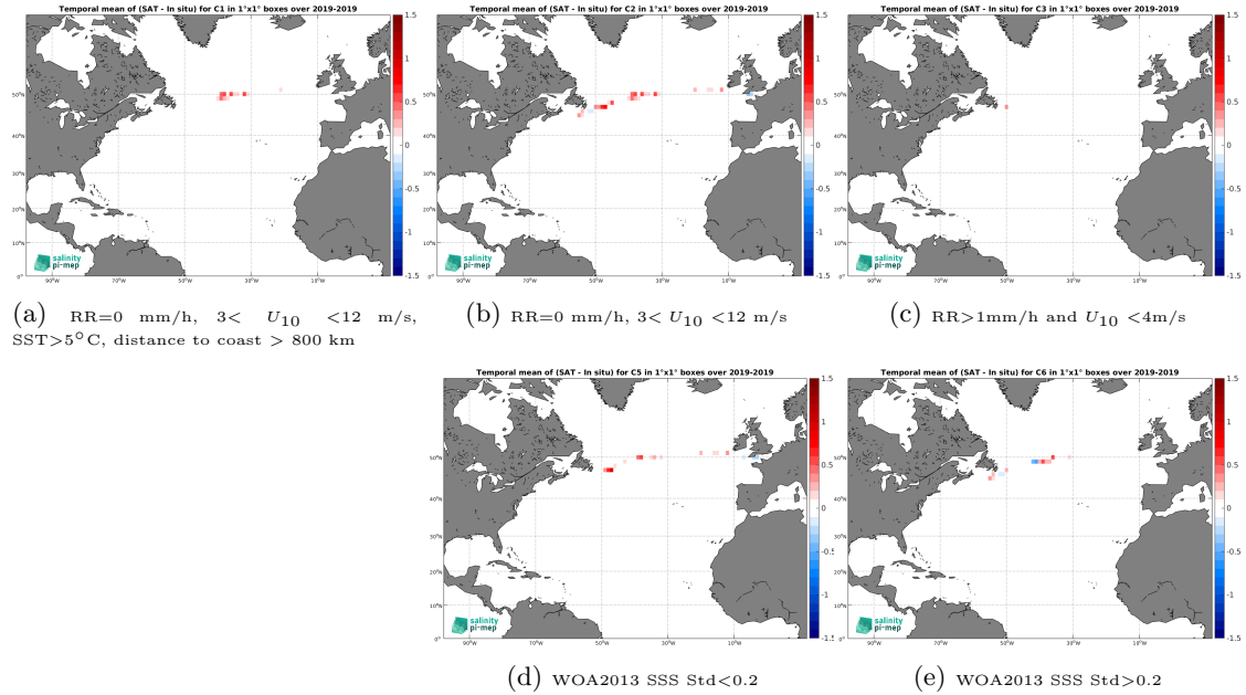
Figure 12: Temporal mean gridded over spatial boxes of size 1^{\circ}\times 1^{\circ} of \Delta\text{SSS} (SMOS SSS L3 Arctic v2 - 18 Days (CATDS-CEC-LOCEAN) - Saildrone) for 5 different subdatasets corresponding to: RR=0 mm/h, 3 < U_{10} < 12 m/s, SST > 5^{\circ}\text{C} , distance to coast > 800 km (a), RR=0 mm/h, 3 < U_{10} < 12 m/s (b), RR > 1 mm/h and U_{10} < 4 m/s (c), WOA2013 SSS Std < 0.2 (d), WOA2013 SSS Std > 0.2 (e).
