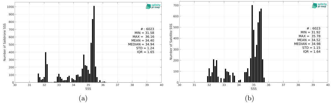
Figure 2: Histograms of SSS from Saildrone (a) and SMOS SSS L3 Arctic v2 - 18 Days (CATDS-CEC-LOCEAN) (b) considering all match-up pairs per bins of 0.1 over the North Atlantic Ocean Pi-MEP region and for the full satellite product period.
