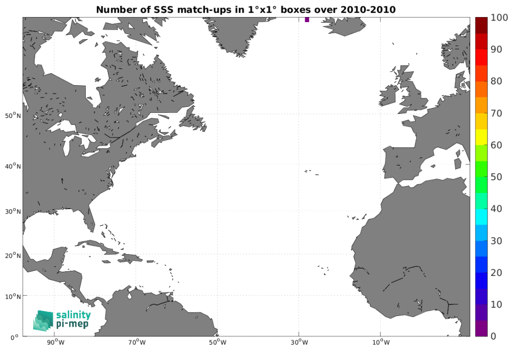
Figure 5: Number of SSS match-ups between Marine mammals SSS and the SMOS SSS L3 Arctic v2 - 18 Days (CATDS-CEC-LOCEAN) SSS product for the North Atlantic Ocean Pi-MEP region over 1^\circ \times 1^\circ boxes and for the full satellite product period.
