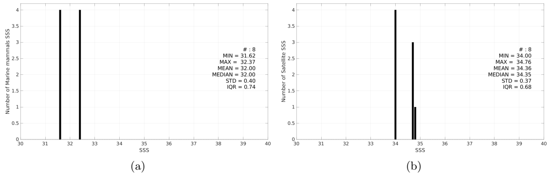
Figure 3: Histograms of SSS from Marine mammals (a) and SMOS SSS L3 Arctic v2 - 18 Days (CATDS-CEC-LOCEAN) (b) considering all match-up pairs per bins of 0.1 over the North Atlantic Ocean Pi-MEP region and for the full satellite product period.
