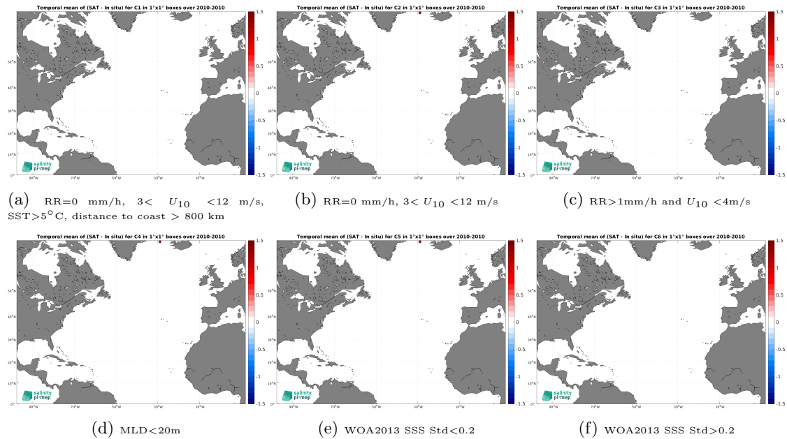
Figure 14: Temporal mean gridded over spatial boxes of size 1^\circ \times 1^\circ of \Delta SSS (SMOS SSS L3 Arctic v2 - 18 Days (CATDS-CEC-LOCEAN) - Marine mammals) for 6 different subdatasets corresponding to:RR=0 mm/h, 3 < U_{10} < 12 m/s, SST > 5^\circ\text{C} , distance to coast > 800 km (a), RR=0 mm/h, 3 < U_{10} < 12 m/s (b), RR > 1 mm/h and U_{10} < 4 m/s (c),MLD < 20 m (d),WOA2013 SSS Std < 0.2 (e),WOA2013 SSS Std > 0.2 (f).
