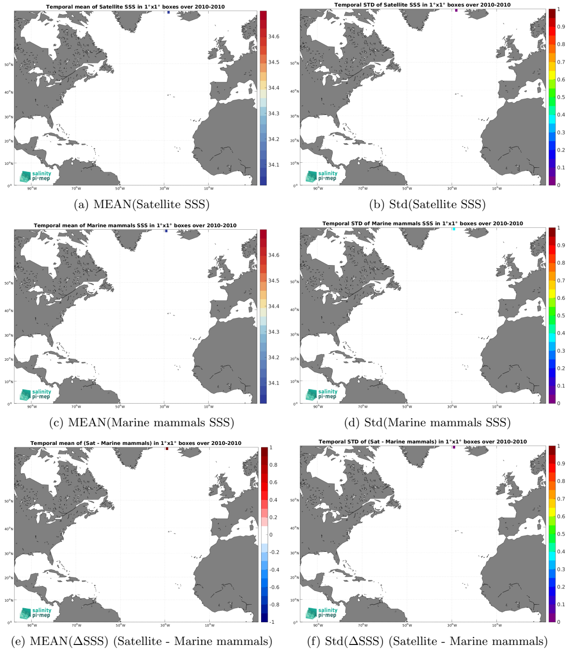
Figure 7: Temporal mean (left) and Std (right) of SSS from SMOS SSS L3 Arctic v2 - 18 Days (CATDS-CEC-LOCEAN) (top), Marine mammals (middle), and of \Delta SSS (Satellite - Marine mammals). Only match-up pairs are used to generate these maps.
