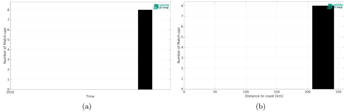
Figure 2: Number of match-ups between Marine mammals and SMOS SSS L3 Arctic v2 - 18 Days (CATDS-CEC-LOCEAN) SSS as a function of time (a) and as function of the distance to coast (b) over the North Atlantic Ocean Pi-MEP region and for the full satellite product period.
