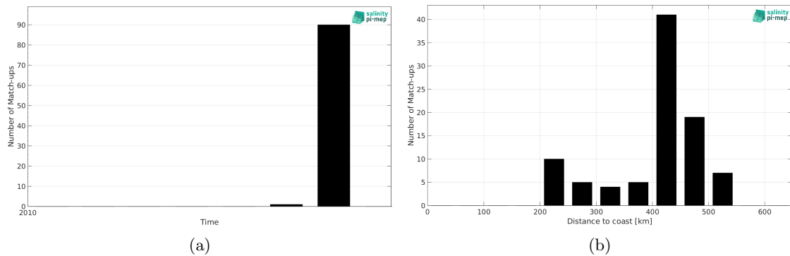
Figure 1: Number of match-ups between Marine mammals and SMOS SSS L3 Arctic v2 - 18 Days (CATDS-CEC-LOCEAN) SSS as a function of time (a) and as function of the distance to coast (b) over the North Atlantic Ocean Pi-MEP region and for the full satellite product period.
