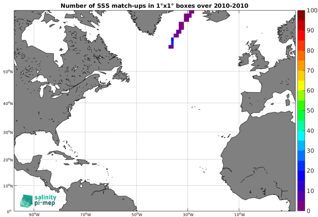
Figure 4: Number of SSS match-ups between Marine mammals SSS and the SMOS SSS L3 Arctic v2 - 18 Days (CATDS-CEC-LOCEAN) SSS product for the North Atlantic Ocean Pi-MEP region over 1^\circ \times 1^\circ boxes and for the full satellite product period.
