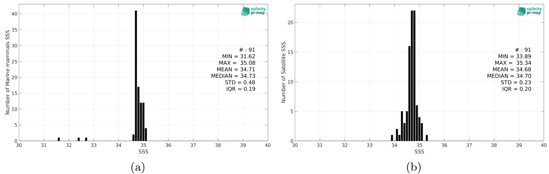
Figure 2: Histograms of SSS from Marine mammals (a) and SMOS SSS L3 Arctic v2 - 18 Days (CATDS-CEC-LOCEAN) (b) considering all match-up pairs per bins of 0.1 over the North Atlantic Ocean Pi-MEP region and for the full satellite product period.
