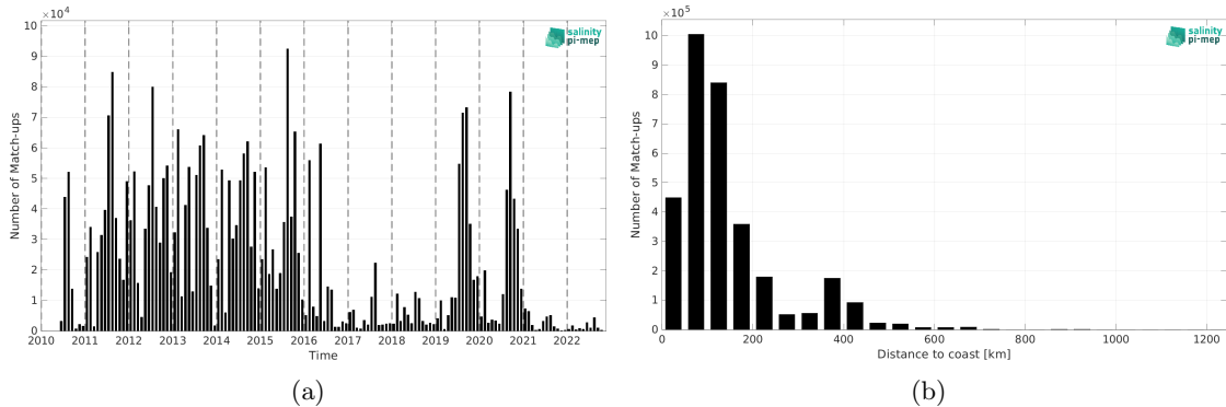
Figure 2: Number of match-ups between ICES and SMOS SSS L3 Arctic v2 - 18 Days (CATDS-CEC-LOCEAN) SSS as a function of time (a) and as function of the distance to coast (b) over the North Atlantic Ocean Pi-MEP region and for the full satellite product period.
