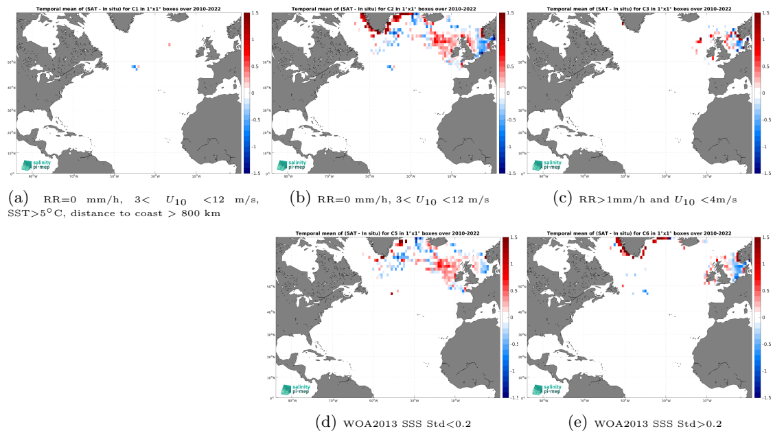
Figure 14: Temporal mean gridded over spatial boxes of size 1^\circ \times 1^\circ of \Delta\text{SSS} (SMOS SSS L3 Arctic v2 - 18 Days (CATDS-CEC-LOCEAN) - ICES) for 5 different subdatasets corresponding to:RR=0 mm/h, 3 < U_{10} < 12 m/s, SST > 5°C, distance to coast > 800 km (a), RR=0 mm/h, 3 < U_{10} < 12 m/s (b), RR > 1mm/h and U_{10} < 4 m/s (c), WOA2013 SSS Std < 0.2 (d), WOA2013 SSS Std > 0.2 (e).
