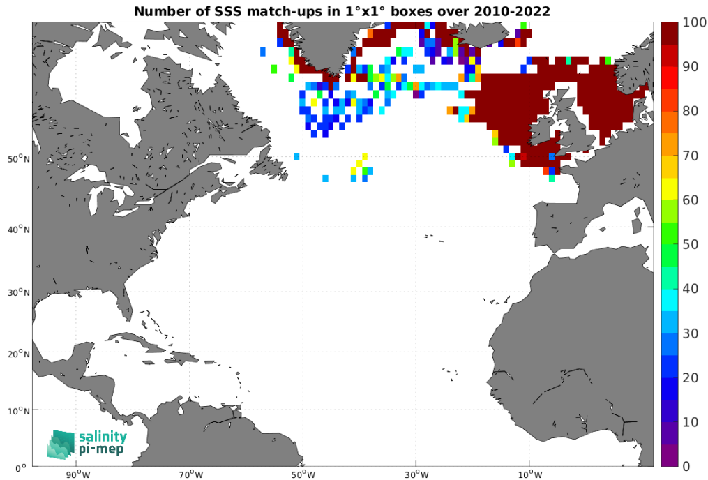
Figure 5: Number of SSS match-ups between ICES SSS and the SMOS SSS L3 Arctic v2 - 18 Days (CATDS-CEC-LOCEAN) SSS product for the North Atlantic Ocean Pi-MEP region over 1^\circ \times 1^\circ boxes and for the full satellite product period.
