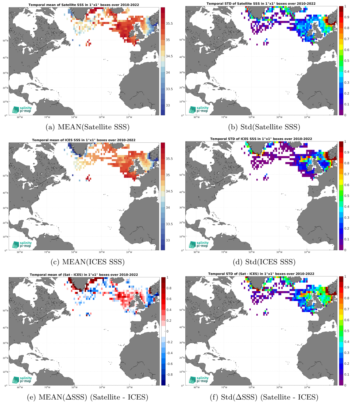
Figure 7: Temporal mean (left) and Std (right) of SSS from SMOS SSS L3 Arctic v2 - 18 Days (CATDS-CEC-LOCEAN) (top), ICES (middle), and of \Delta SSS (Satellite - ICES). Only match-up pairs are used to generate these maps.
