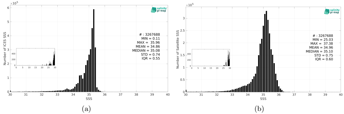
Figure 3: Histograms of SSS from ICES (a) and SMOS SSS L3 Arctic v2 - 18 Days (CATDS-CEC-LOCEAN) (b) considering all match-up pairs per bins of 0.1 over the North Atlantic Ocean Pi-MEP region and for the full satellite product period.
