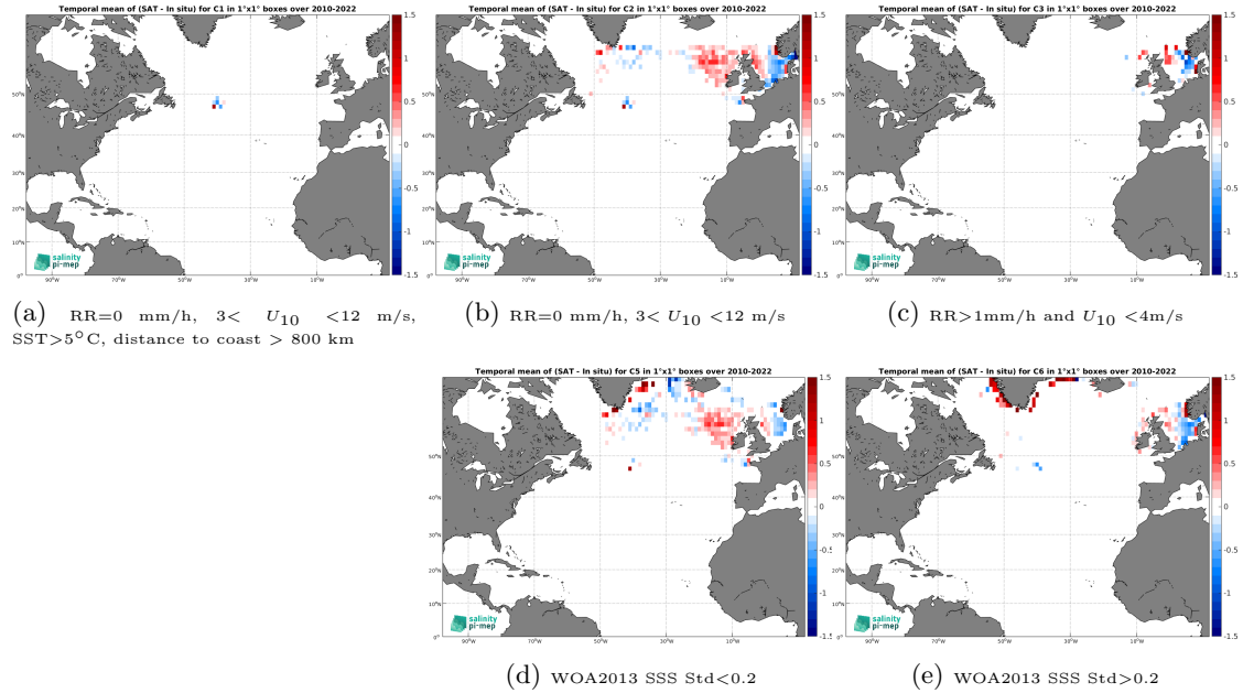
Figure 12: Temporal mean gridded over spatial boxes of size 1^{\circ}\times 1^{\circ} of \Delta\text{SSS} (SMOS SSS L3 Arctic v2 - 18 Days (CATDS-CEC-LOCEAN) - ICES) for 5 different subdatasets corresponding to: RR=0 mm/h, 3 < U_{10} < 12 m/s, SST > 5^{\circ}\text{C} , distance to coast > 800 km (a), RR=0 mm/h, 3 < U_{10} < 12 m/s (b), RR > 1 mm/h and U_{10} < 4 m/s (c), WOA2013 SSS Std < 0.2 (d), WOA2013 SSS Std > 0.2 (e).
