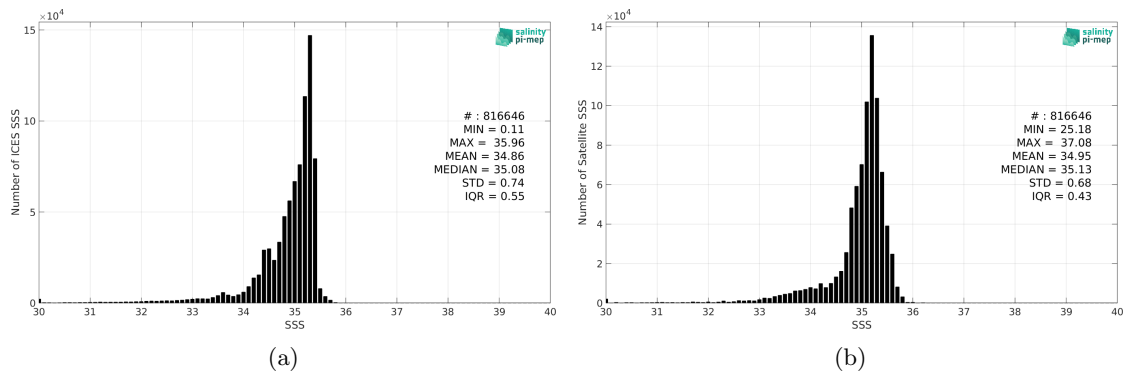
Figure 2: Histograms of SSS from ICES (a) and SMOS SSS L3 Arctic v2 - 18 Days (CATDS-CEC-LOCEAN) (b) considering all match-up pairs per bins of 0.1 over the North Atlantic Ocean Pi-MEP region and for the full satellite product period.
