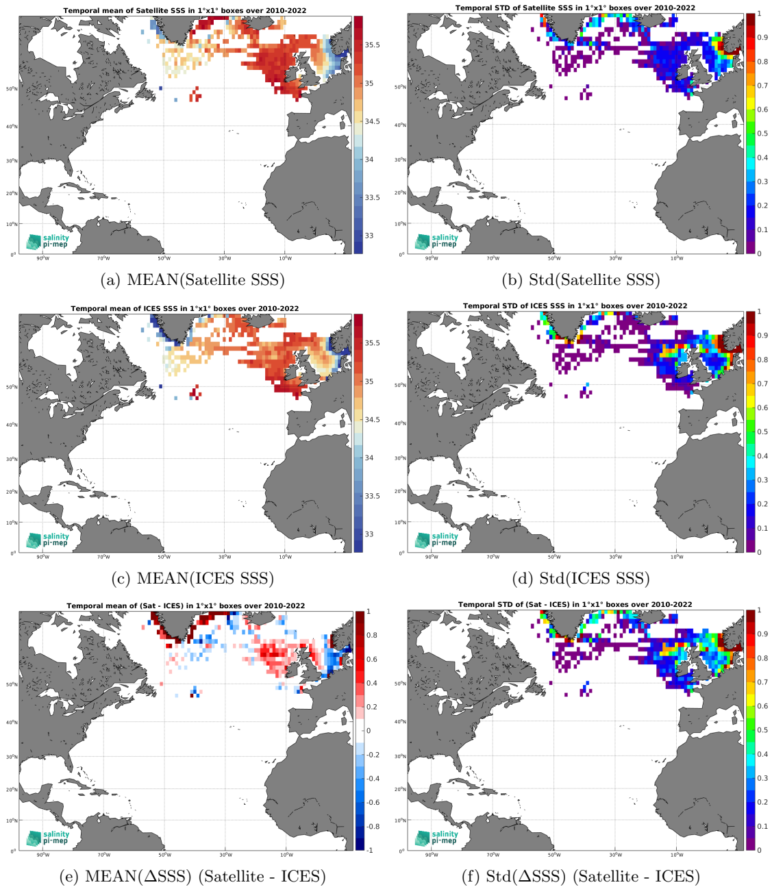
Figure 6: Temporal mean (left) and Std (right) of SSS from SMOS SSS L3 Arctic v2 - 18 Days (CATDS-CEC-LOCEAN) (top), ICES (middle), and of \Delta SSS (Satellite - ICES). Only match-up pairs are used to generate these maps.
