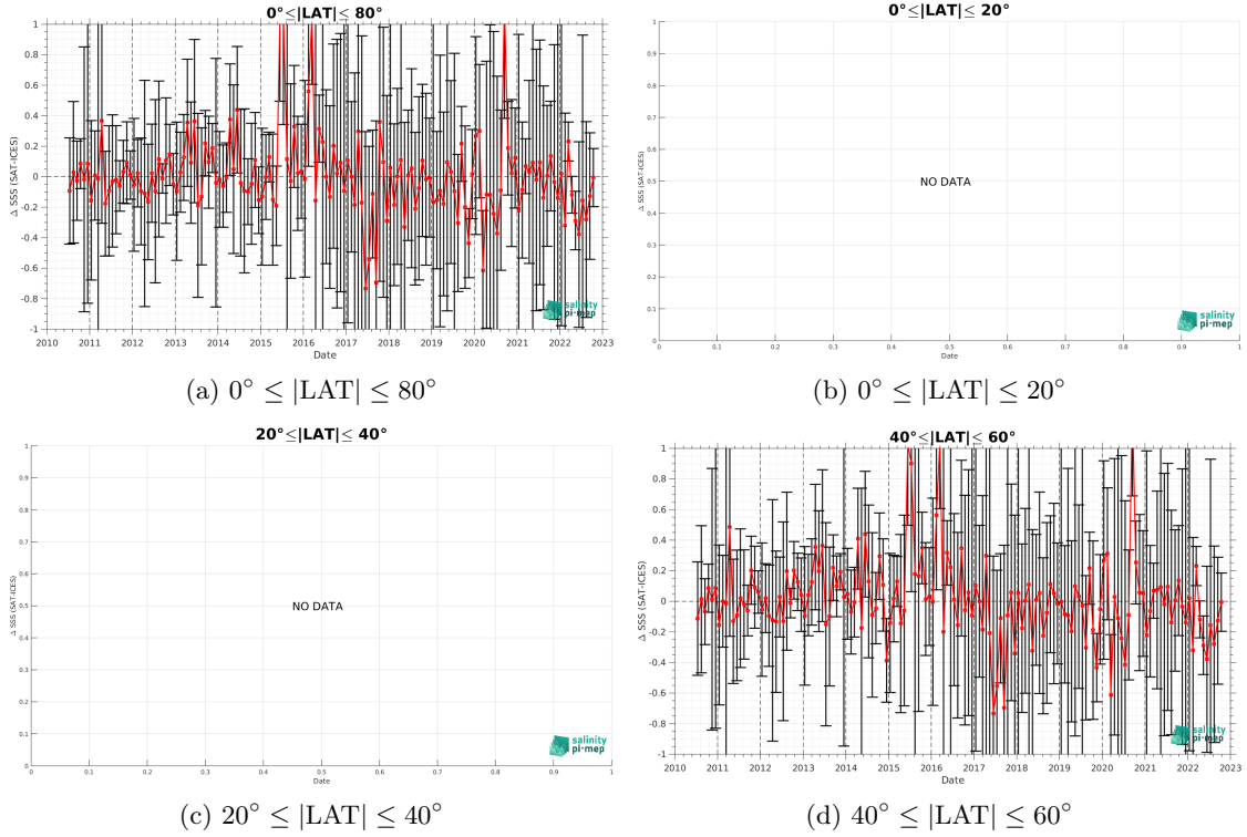
Figure 10: Monthly median (red curves) of \Delta SSS (Satellite - ICES) and \pm 1 Std (black vertical thick bars) as function of time for all the collected Pi-MEP match-up pairs estimated over the North Atlantic Ocean Pi-MEP region and for the full satellite product period are shown for different latitude bands: (a) 80^{\circ}\text{S}-80^{\circ}\text{N} , (b) 20^{\circ}\text{S}-20^{\circ}\text{N} , (c) 40^{\circ}\text{S}-20^{\circ}\text{S} and 20^{\circ}\text{N}-40^{\circ}\text{N} and (d) 60^{\circ}\text{S}-40^{\circ}\text{S} and 40^{\circ}\text{N}-60^{\circ}\text{N} .
