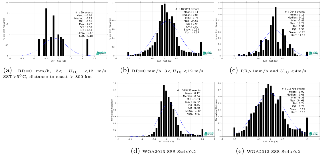
Figure 13: Normalized histogram of \Delta SSS (SMOS SSS L3 Arctic v2 - 18 Days (CATDS-CEC-LOCEAN) - ICES) for 5 different subdatasets corresponding to: RR=0 mm/h, 3 < U_{10} < 12 m/s, SST>5°C, distance to coast > 800 km (a), RR=0 mm/h, 3 < U_{10} < 12 m/s (b), RR>1mm/h and U_{10} < 4 m/s (c), WOA2013 SSS Std<0.2 (d), WOA2013 SSS Std>0.2 (e).
