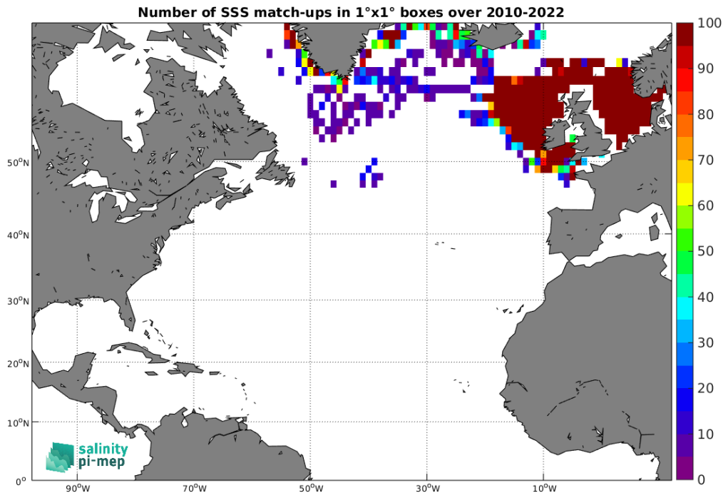
Figure 4: Number of SSS match-ups between ICES SSS and the SMOS SSS L3 Arctic v2 - 18 Days (CATDS-CEC-LOCEAN) SSS product for the North Atlantic Ocean Pi-MEP region over 1^\circ \times 1^\circ boxes and for the full satellite product period.
