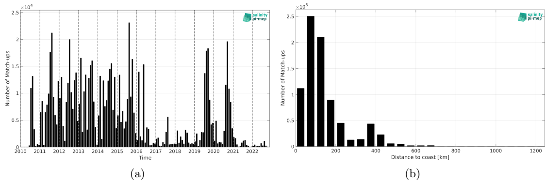
Figure 1: Number of match-ups between ICES and SMOS SSS L3 Arctic v2 - 18 Days (CATDS-CEC-LOCEAN) SSS as a function of time (a) and as function of the distance to coast (b) over the North Atlantic Ocean Pi-MEP region and for the full satellite product period.
