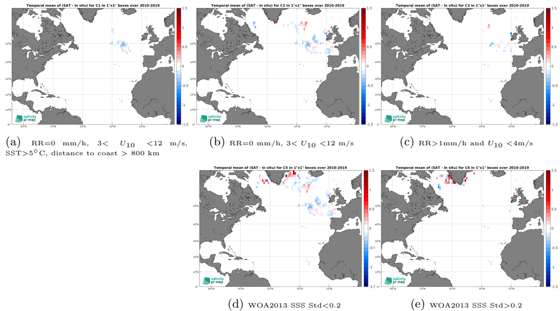
Figure 11: Temporal mean gridded over spatial boxes of size 1^{\circ}\times 1^{\circ} of \Delta\text{SSS} (SMOS SSS L3 Arctic v2 - 18 Days (CATDS-CEC-LOCEAN) - Surface drifters) for 5 different subdatasets corresponding to:RR=0 mm/h, 3 < U_{10} < 12 m/s, SST > 5^{\circ}\text{C} , distance to coast > 800 km (a), RR=0 mm/h, 3 < U_{10} < 12 m/s (b), RR > 1 mm/h and U_{10} < 4 m/s (c), WOA2013 SSS Std < 0.2 (d), WOA2013 SSS Std > 0.2 (e).
