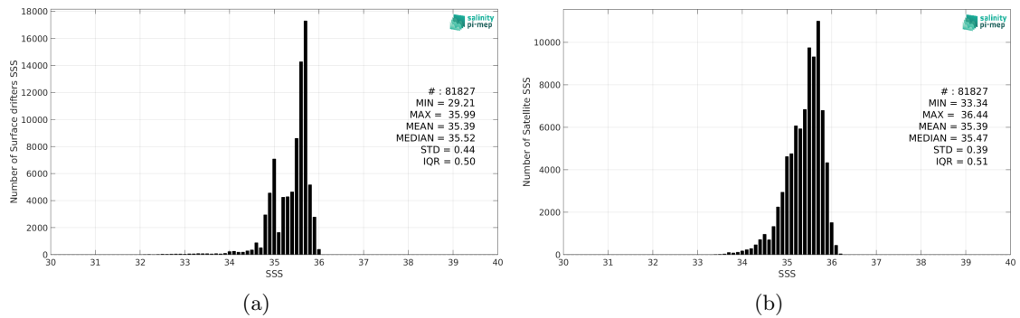
Figure 2: Histograms of SSS from Surface drifters (a) and SMOS SSS L3 Arctic v2 - 18 Days (CATDS-CEC-LOCEAN) (b) considering all match-up pairs per bins of 0.1 over the North Atlantic Ocean Pi-MEP region and for the full satellite product period.
