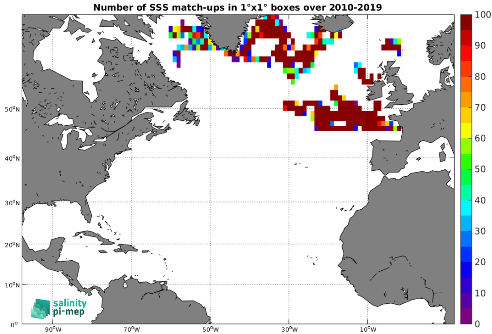
Figure 3: Number of SSS match-ups between Surface drifters SSS and the SMOS SSS L3 Arctic v2 - 18 Days (CATDS-CEC-LOCEAN) SSS product for the North Atlantic Ocean Pi-MEP region over 1^\circ \times 1^\circ boxes and for the full satellite product period.
