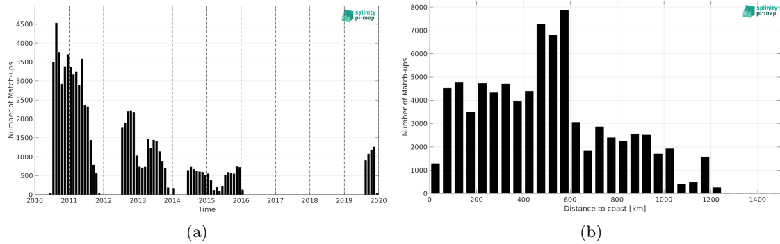
Figure 1: Number of match-ups between Surface drifters and SMOS SSS L3 Arctic v2 - 18 Days (CATDS-CEC-LOCEAN) SSS as a function of time (a) and as function of the distance to coast (b) over the North Atlantic Ocean Pi-MEP region and for the full satellite product period.
