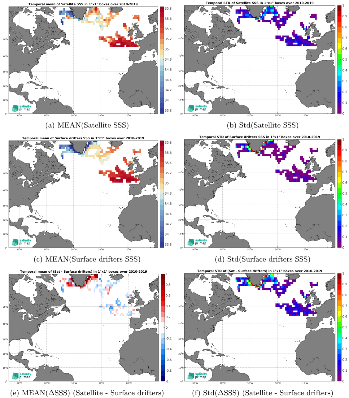
Figure 5: Temporal mean (left) and Std (right) of SSS from SMOS SSS L3 Arctic v2 - 18 Days (CATDS-CEC-LOCEAN) (top), Surface drifters (middle), and of \Delta SSS (Satellite - Surface drifters). Only match-up pairs are used to generate these maps.
