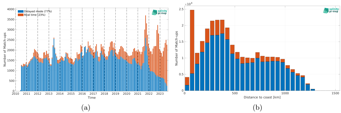
Figure 2: Number of match-ups between Argo and SMOS SSS L3 Arctic v2 - 18 Days (CATDS-CEC-LOCEAN) SSS as a function of time (a) and as function of the distance to coast (b) over the North Atlantic Ocean Pi-MEP region and for the full satellite product period.
