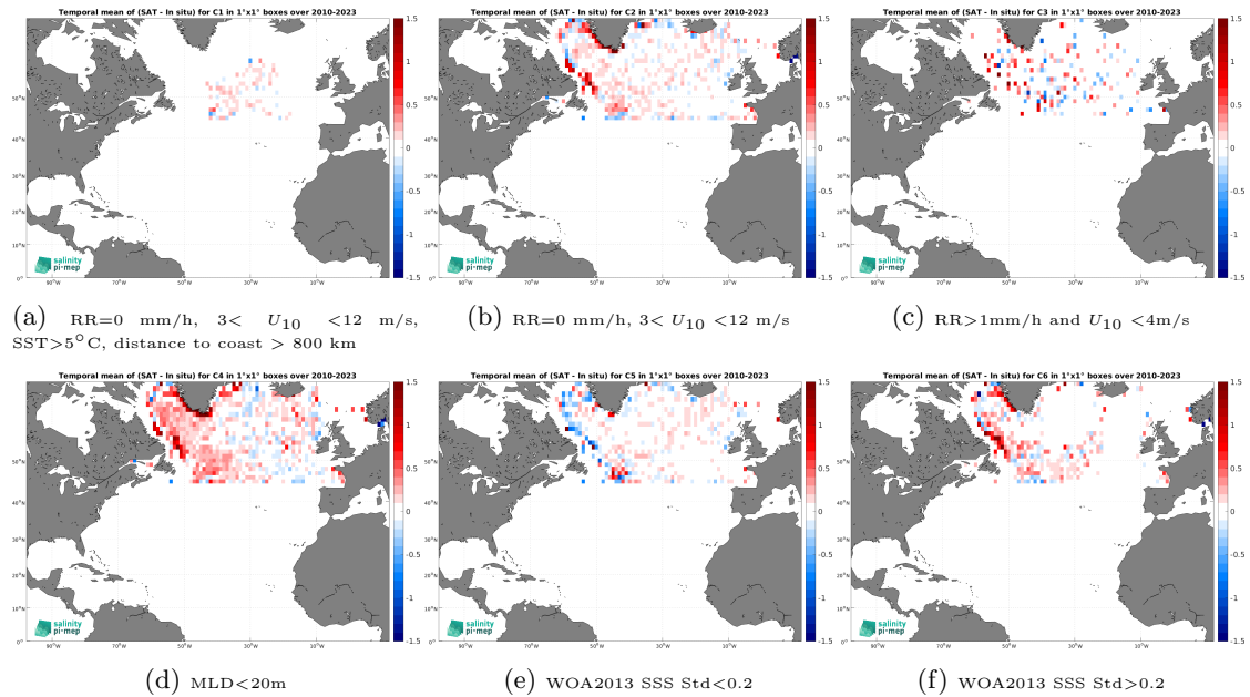
Figure 14: Temporal mean gridded over spatial boxes of size 1^\circ \times 1^\circ of \Delta SSS (SMOS SSS L3 Arctic v2 - 18 Days (CATDS-CEC-LOCEAN) - Argo) for 6 different subdatasets corresponding to:RR=0 mm/h, 3 < U_{10} < 12 m/s, SST > 5^\circ\text{C} , distance to coast > 800 km (a), RR=0 mm/h, 3 < U_{10} < 12 m/s (b), RR > 1 mm/h and U_{10} < 4 m/s (c),MLD < 20 m (d),WOA2013 SSS Std < 0.2 (e),WOA2013 SSS Std > 0.2 (f).
