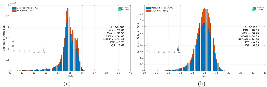
Figure 3: Histograms of SSS from Argo (a) and SMOS SSS L3 Arctic v2 - 18 Days (CATDS-CEC-LOCEAN) (b) considering all match-up pairs per bins of 0.1 over the North Atlantic Ocean Pi-MEP region and for the full satellite product period.
