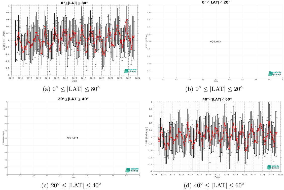
Figure 11: Monthly median (red curves) of \Delta SSS (Satellite - Argo) and \pm 1 Std (black vertical thick bars) as function of time for all the collected Pi-MEP match-up pairs estimated over the North Atlantic Ocean Pi-MEP region and for the full satellite product period are shown for different latitude bands: (a) 80^\circ\text{S}-80^\circ\text{N} , (b) 20^\circ\text{S}-20^\circ\text{N} , (c) 40^\circ\text{S}-20^\circ\text{S} and 20^\circ\text{N}-40^\circ\text{N} and (d) 60^\circ\text{S}-40^\circ\text{S} and 40^\circ\text{N}-60^\circ\text{N} .
