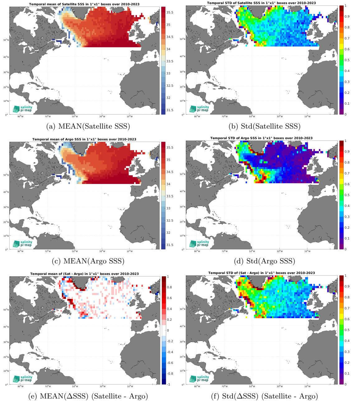
Figure 7: Temporal mean (left) and Std (right) of SSS from SMOS SSS L3 Arctic v2 - 18 Days (CATDS-CEC-LOCEAN) (top), Argo (middle), and of \Delta SSS (Satellite - Argo). Only match-up pairs are used to generate these maps.
