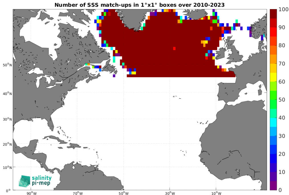
Figure 5: Number of SSS match-ups between Argo SSS and the SMOS SSS L3 Arctic v2 - 18 Days (CATDS-CEC-LOCEAN) SSS product for the North Atlantic Ocean Pi-MEP region over 1^\circ \times 1^\circ boxes and for the full satellite product period.
